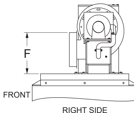
Figure 32. Blower Assembly Position 3
