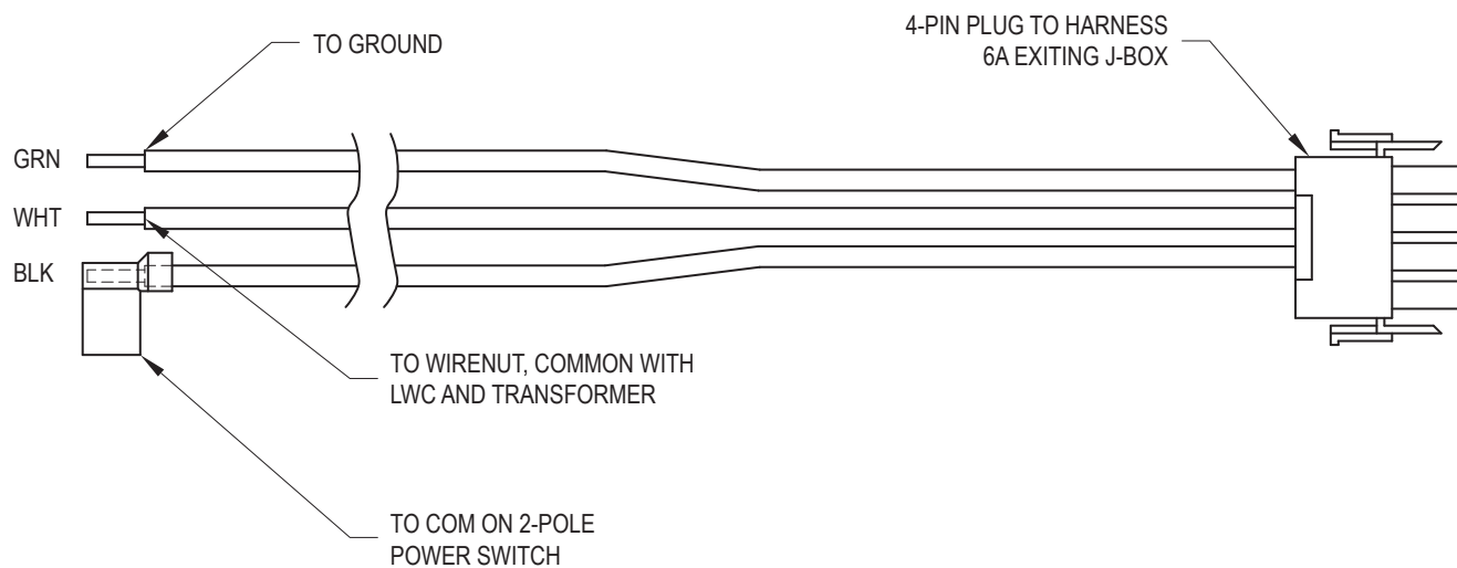
Figure 10. Harness 4, Models 0962-1826
