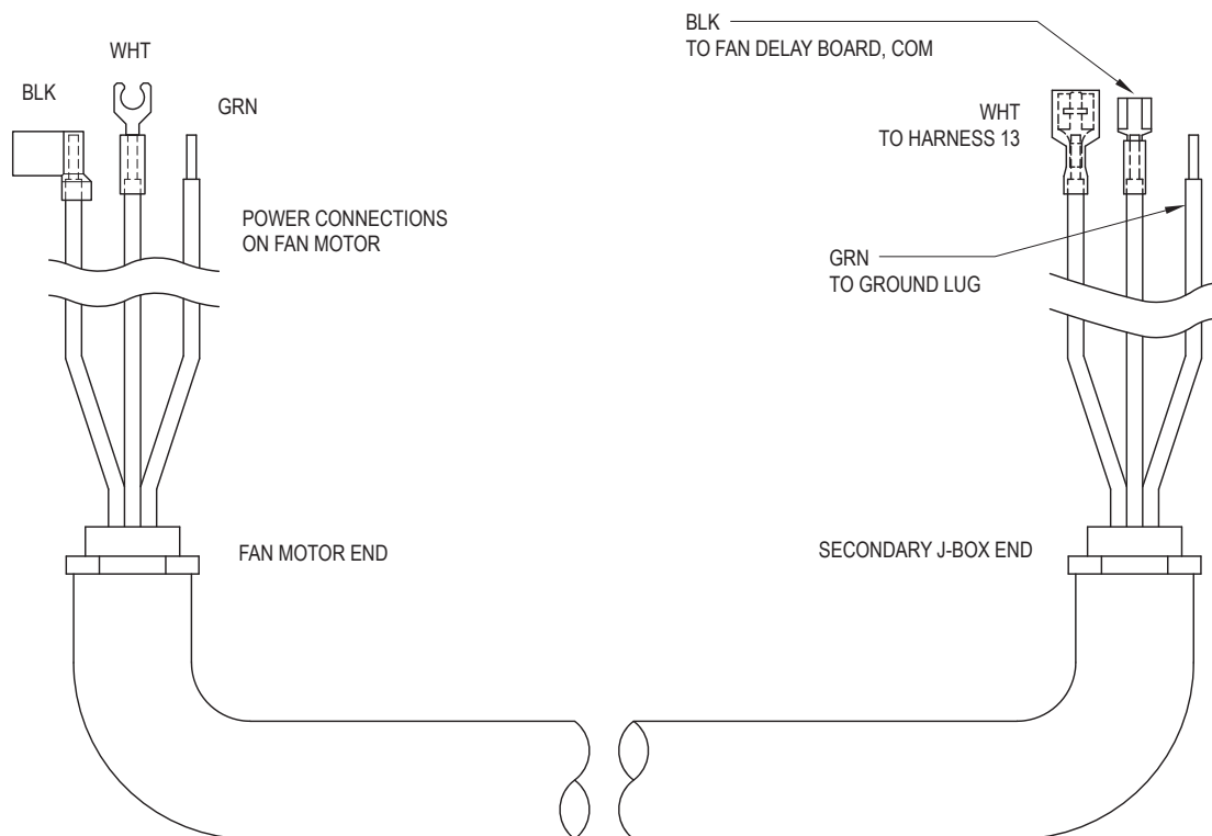
Figure 22. Harness 11, Models 2100-4001
