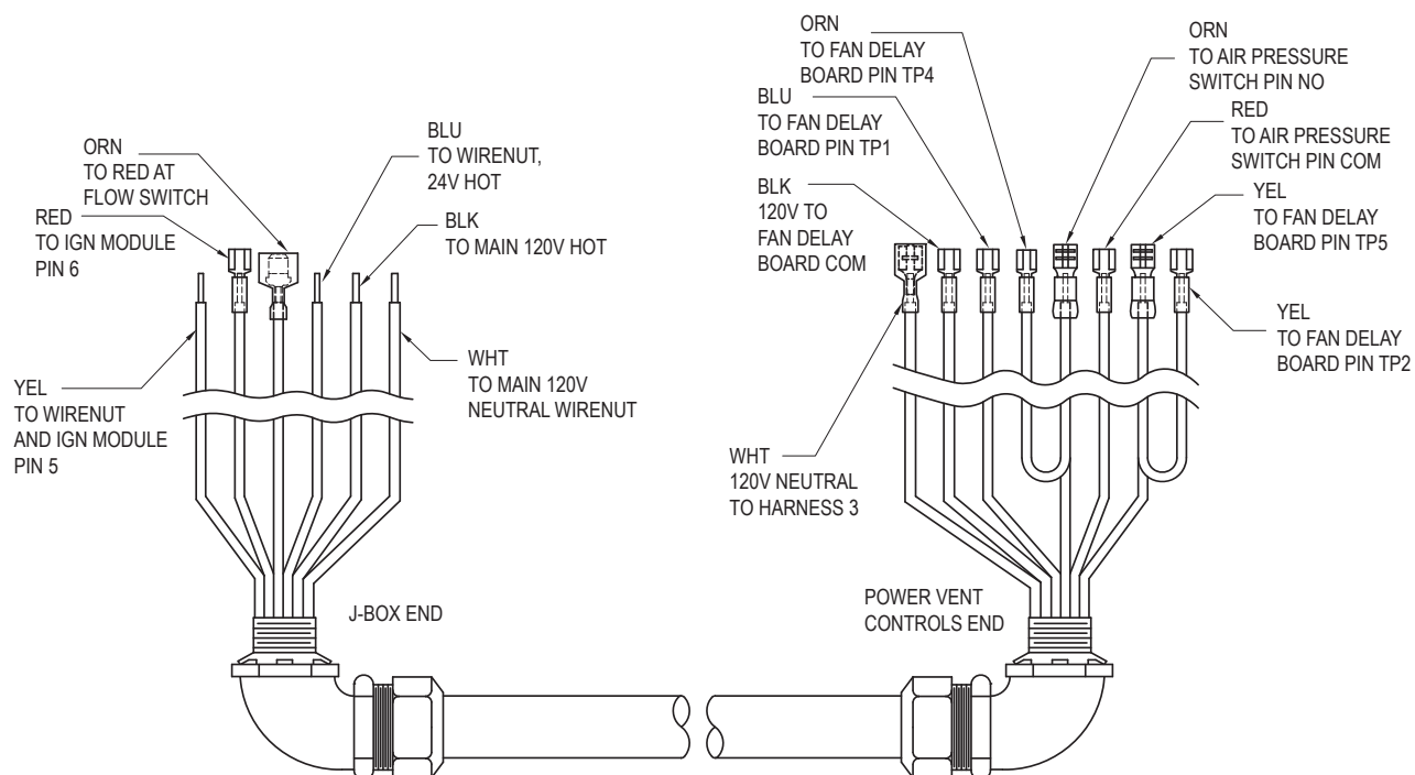
Figure 6. Harness 2, Models 0514-0824
