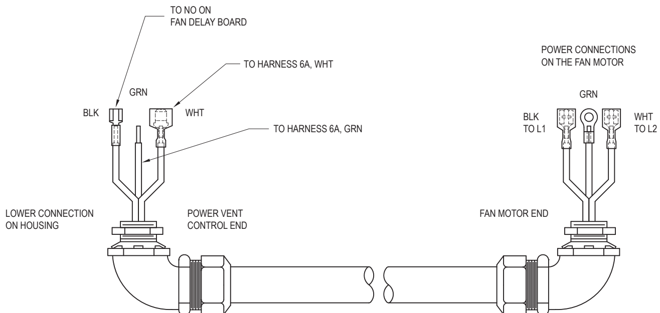
Figure 13. Harness 7, Models 0962-1826
