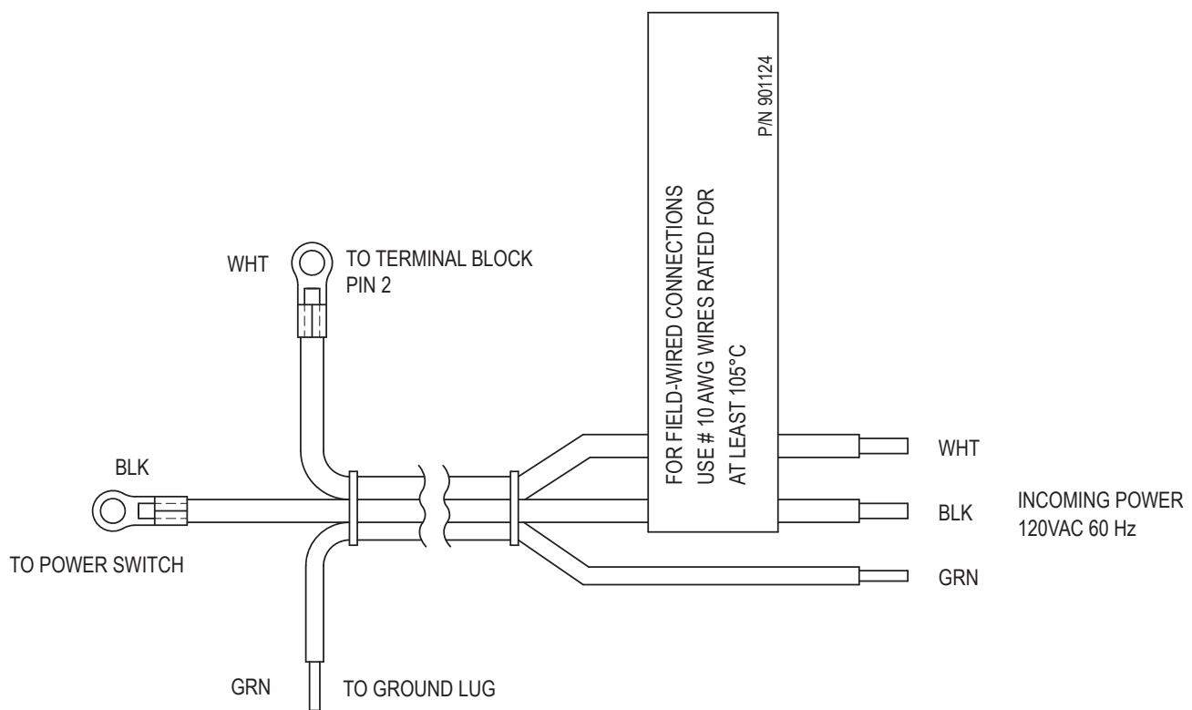
Figure 19. Harness 8, Models 2100-4001
