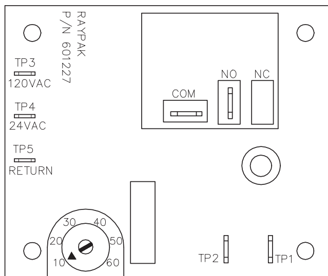
Figure 28. Solid State Fan Delay Board
