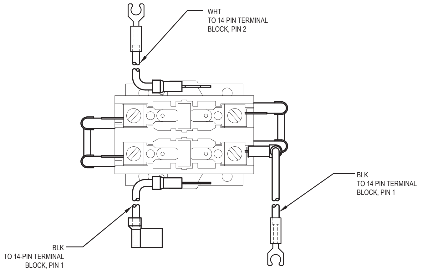
Figure 17. Contactor Assembly
