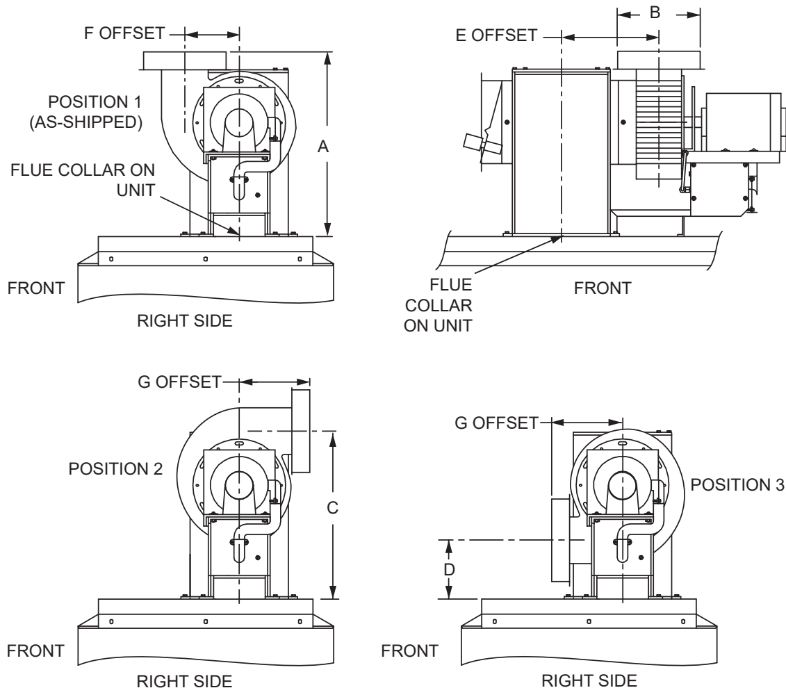
Figure 1. Dimensions, Models 0514-1826
