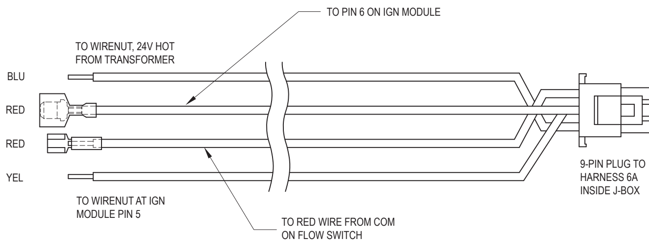
Figure 11. Harness 5, Models 0962-1826
