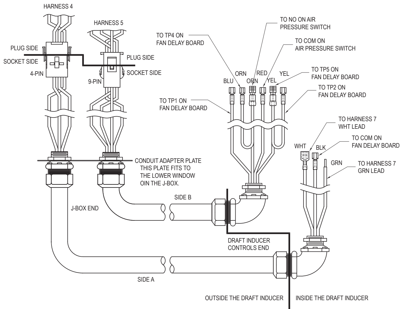
Figure 12. Harness 6, Models 0962-1826
