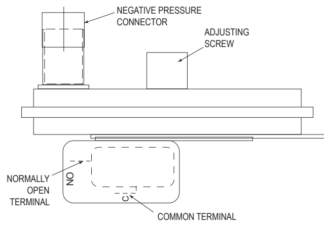
Figure 29. Draft Proving Switch
