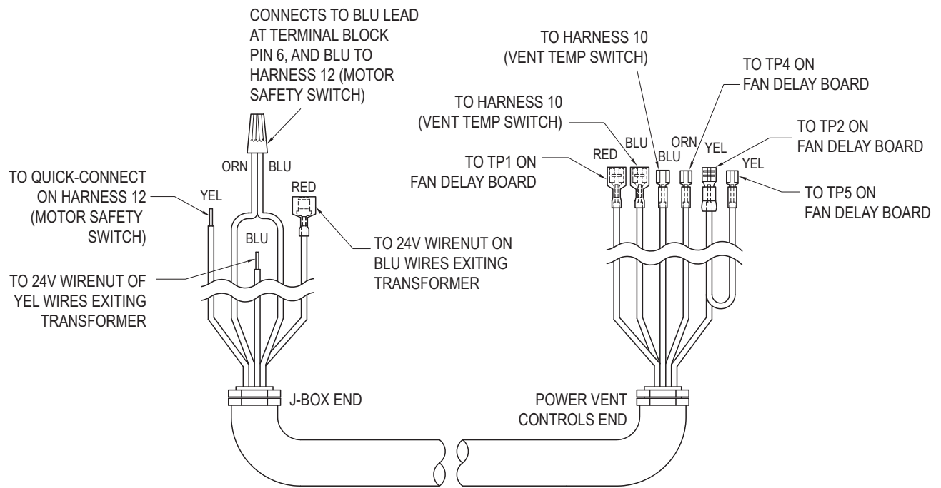
Figure 20. Harness 9, Models 2100-4001
