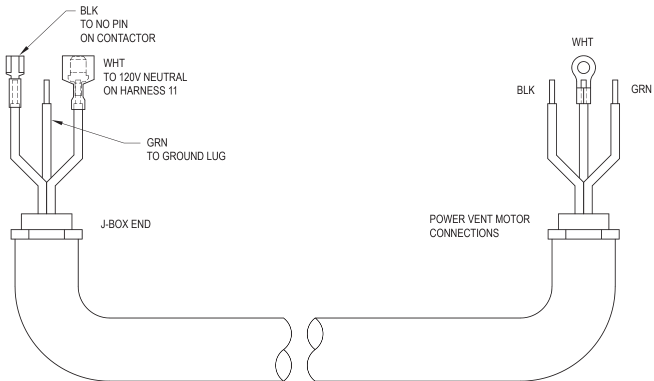
Figure 24. Harness 13, Models 2100-4001
