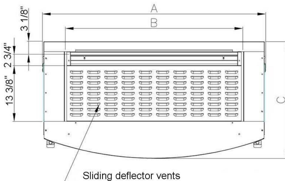
TOP VIEW
