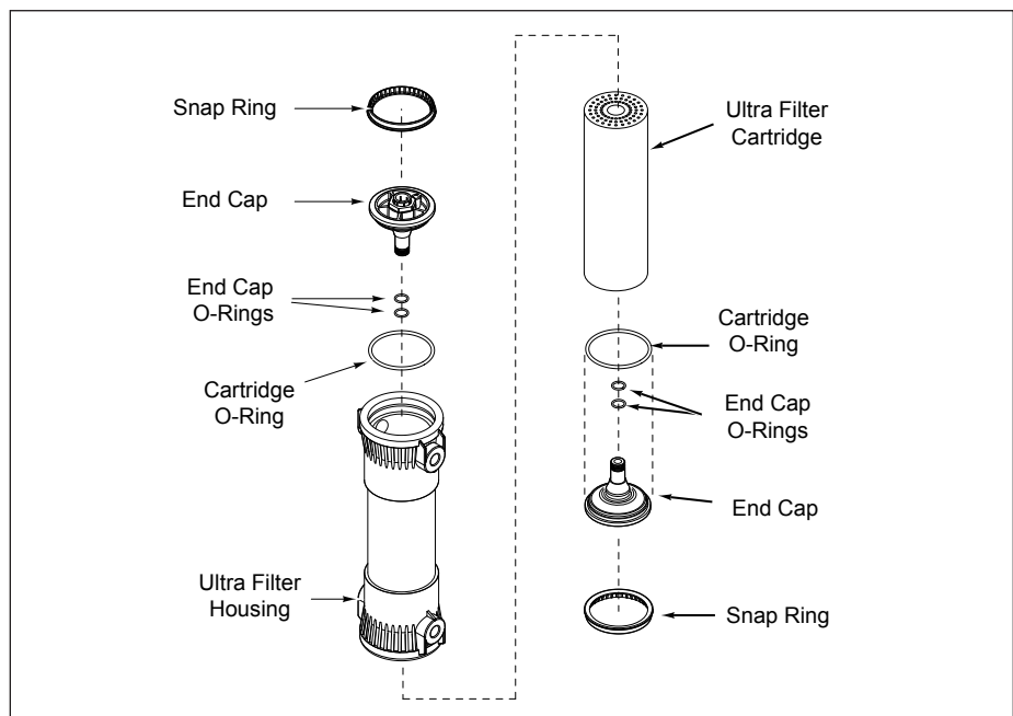
Figure 7. Install Bypass
