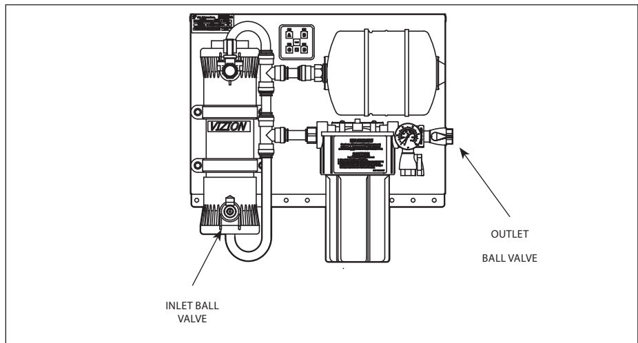
Figure 6. Inlet and Outlet Connections
