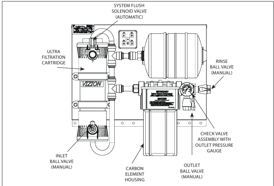
Figure 1. System Components
