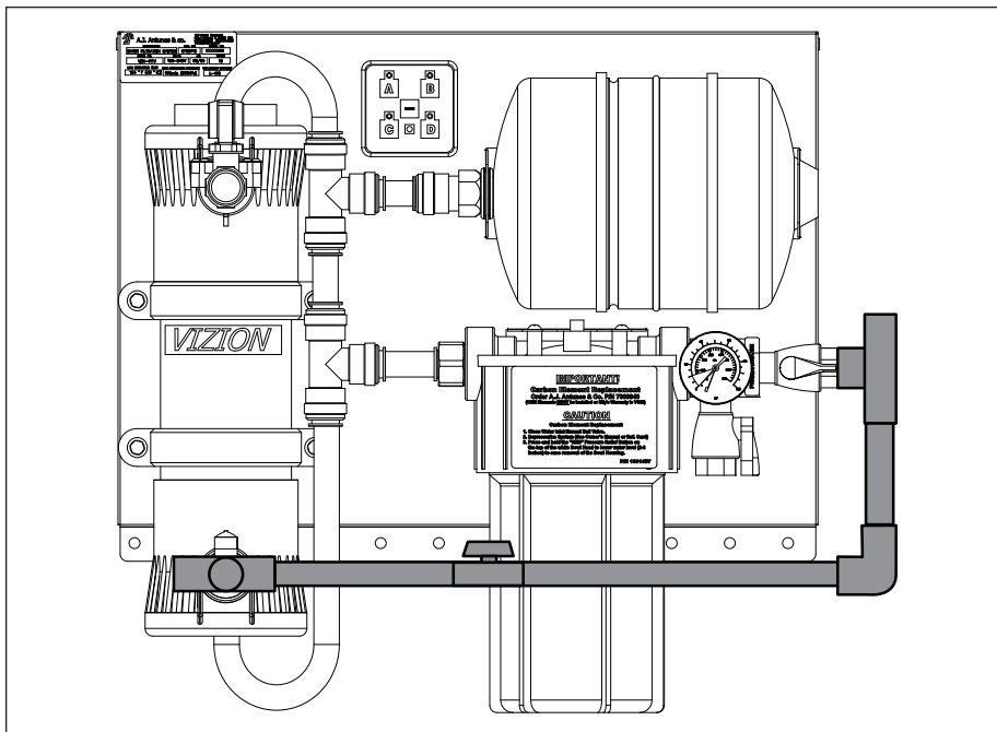
Figure 7. Install Bypass
