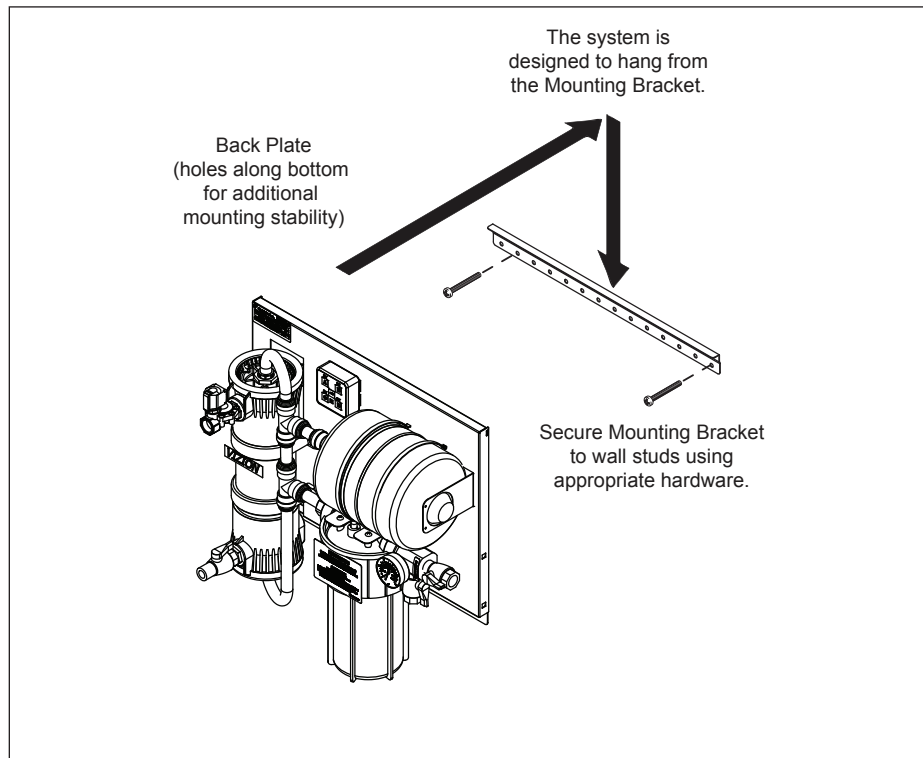
Figure 2. Mounting the System
