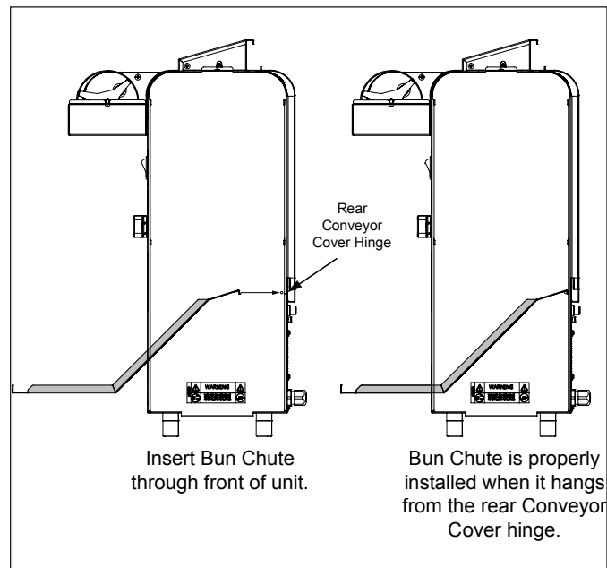
Figure 1. Installing Bun Chute
