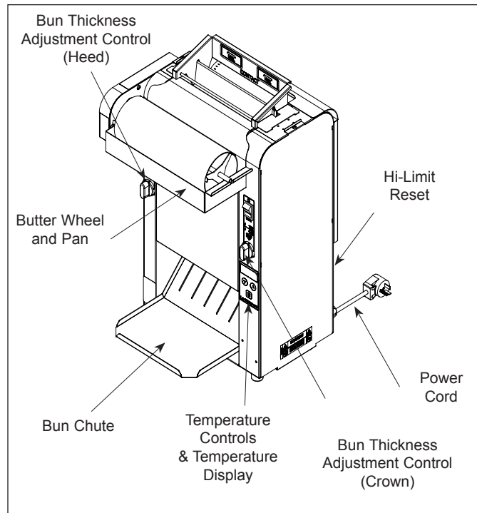
Figure 3. VCTM-2 Toaster
