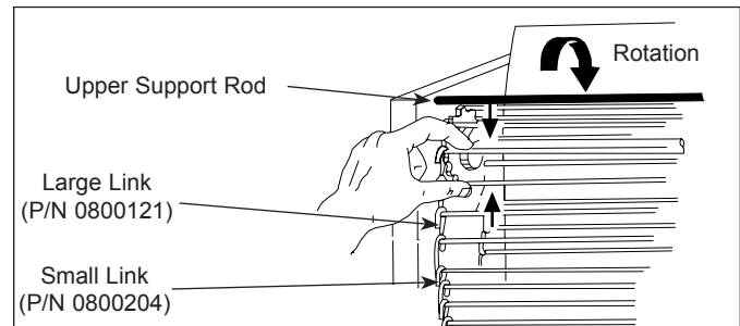
Figure 12. Removing Conveyor Belt Chains
