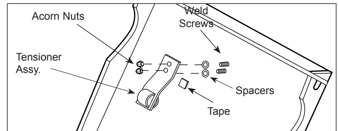
Figure 14. Replacing Roller Tensioner Assy.
