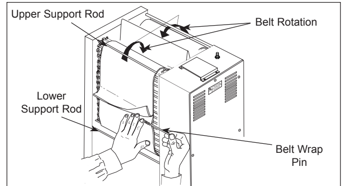
Figure 9. Installing Belt Wrap
