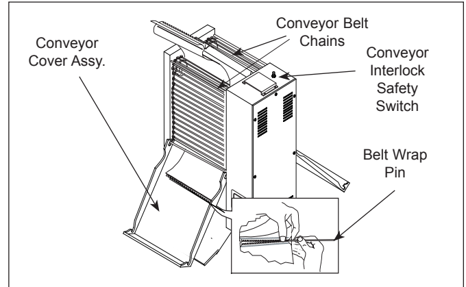
Figure 8. Removing Belt Wrap
