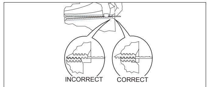
Figure 10. Aligning Belt Teeth
