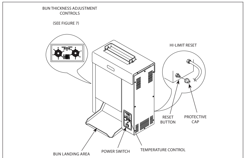
Figure 6. Toaster Controls
