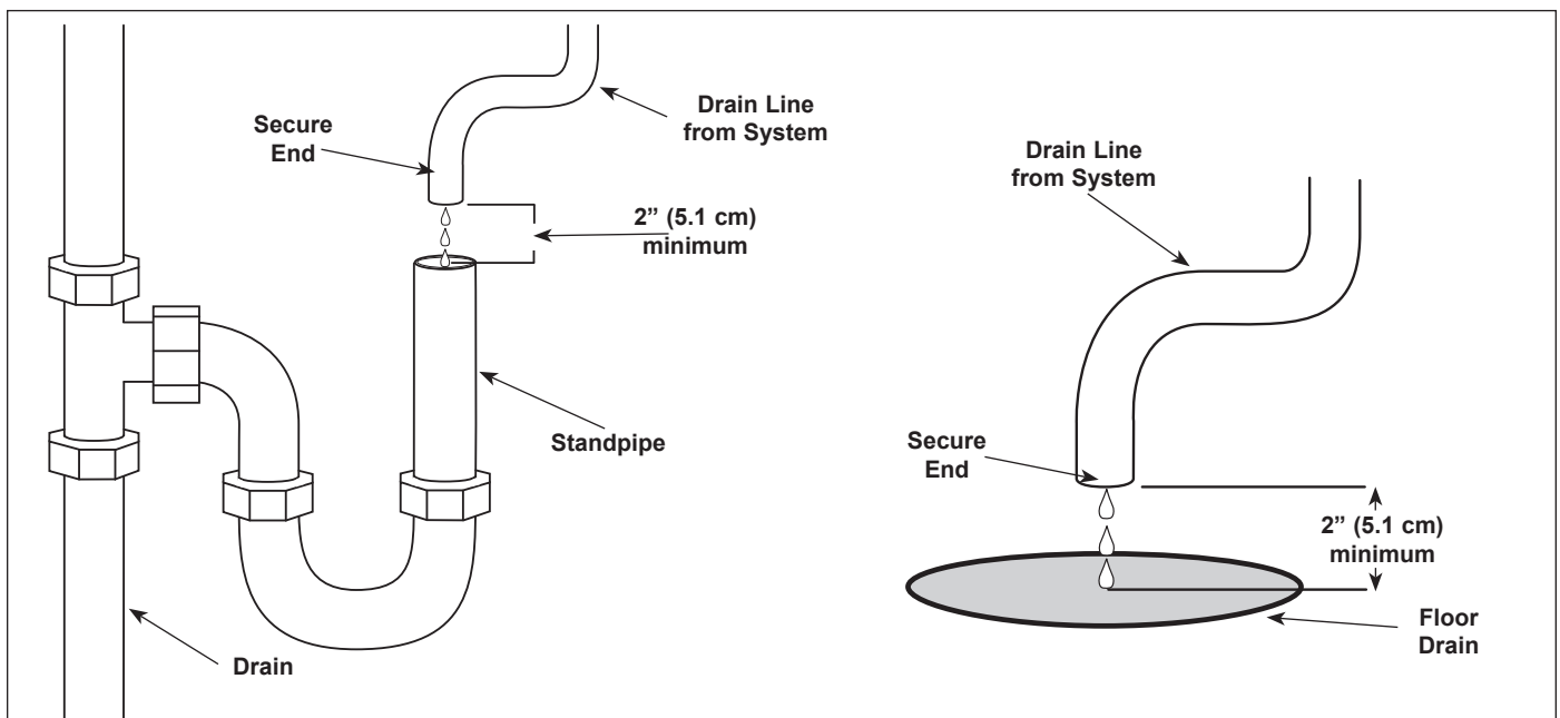
Figure 4. Proper Draining
