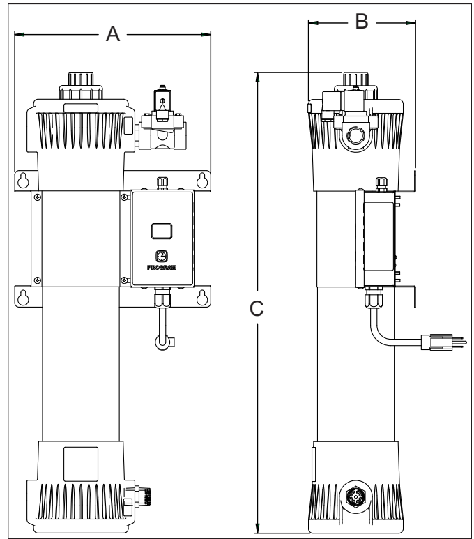
Figure 1. Dimensions
