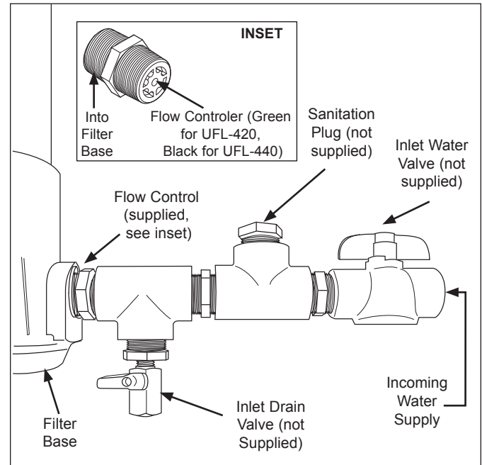
Figure 3. Inlet Water Plumbing
