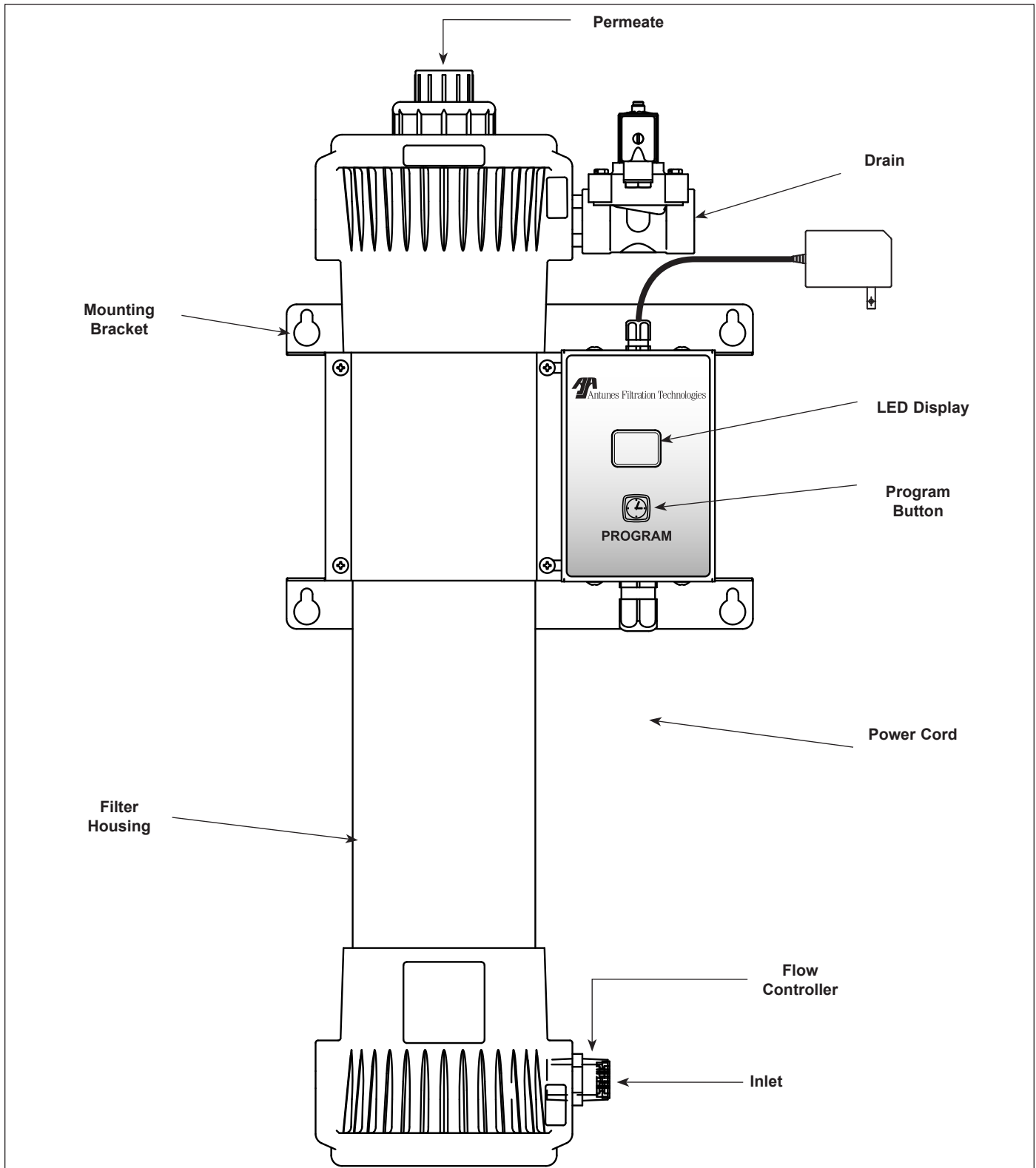
Figure 2. Components
