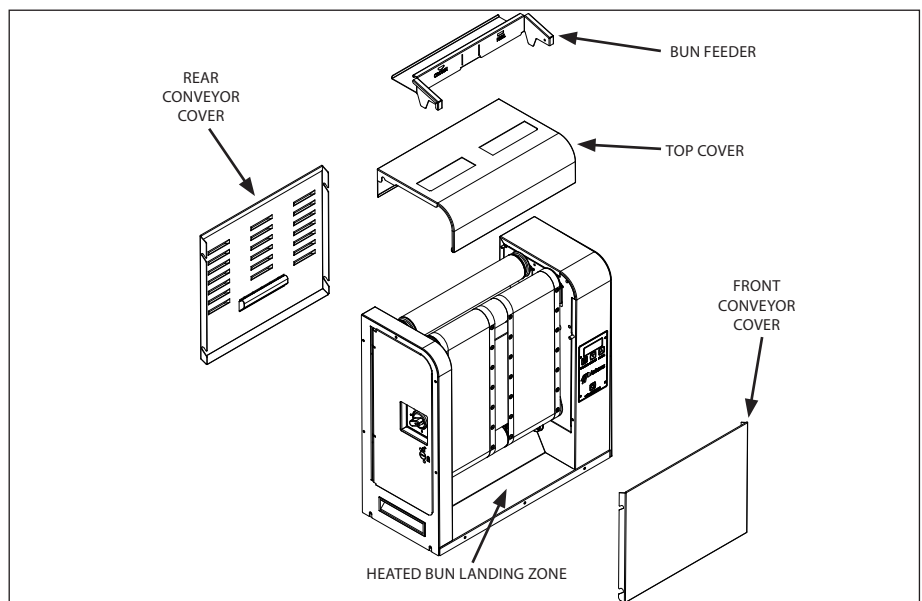
Figure 3. Components
