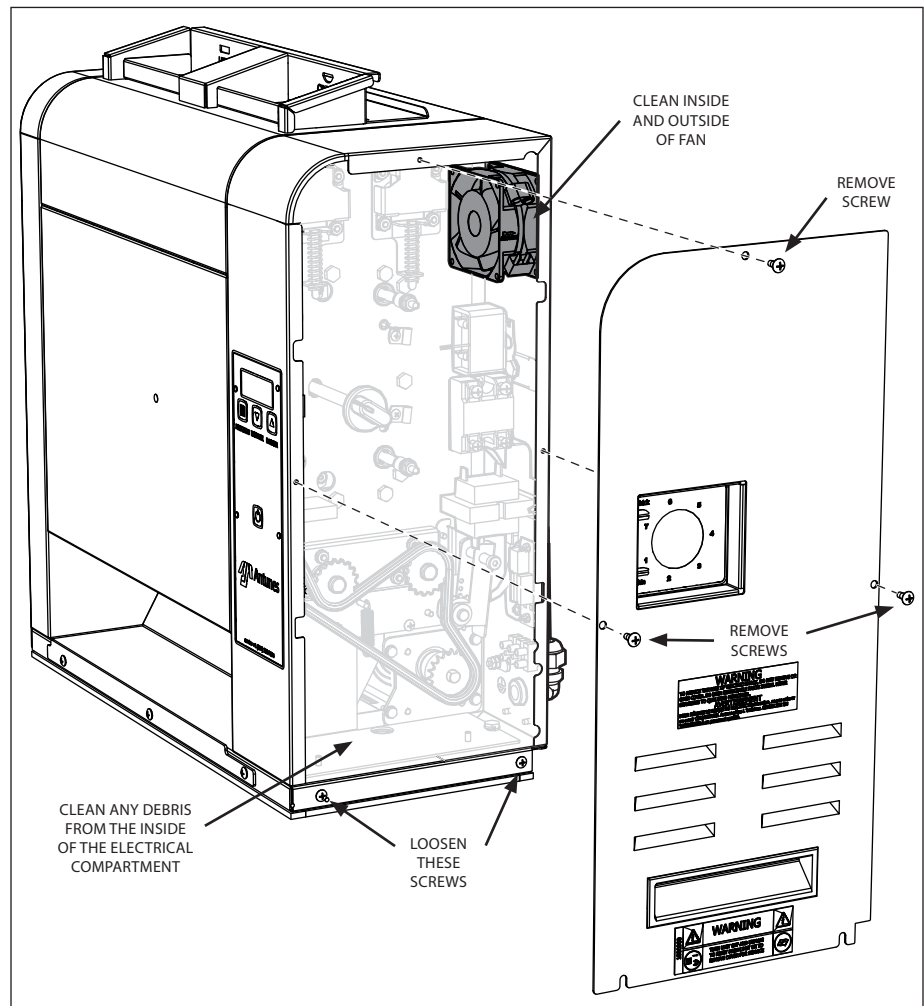
Figure 13. Cleaning Fan and Electrical Compartment
