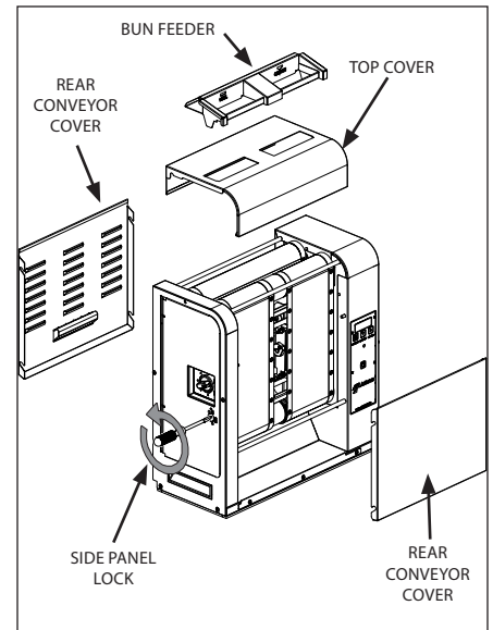
Figure 10. Removing Components
