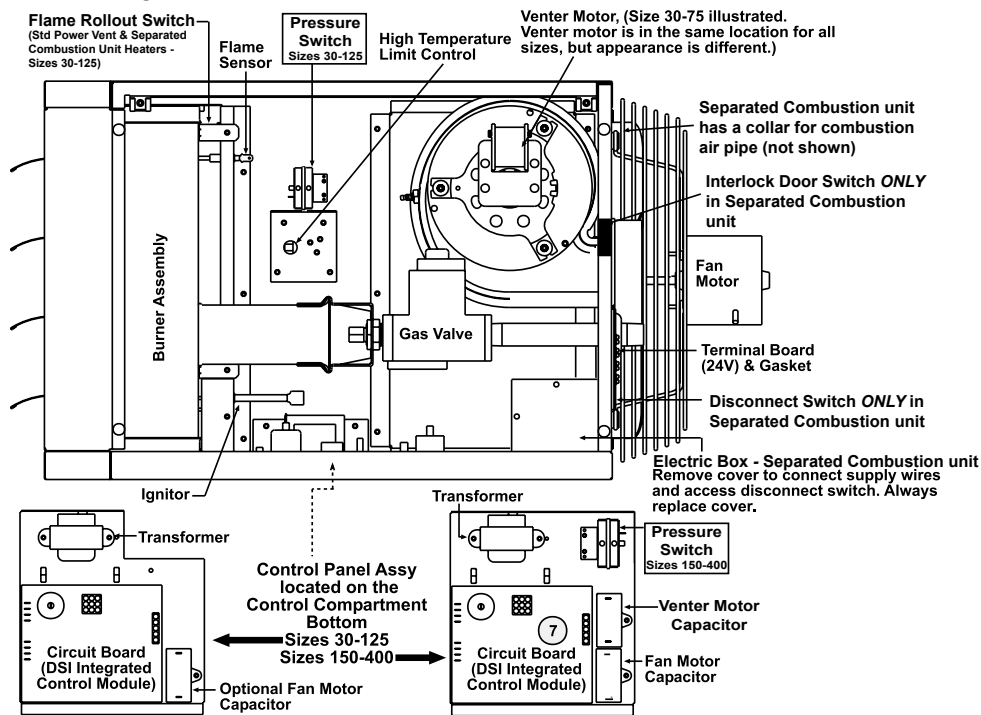
Figure 2 Pressure Switch Location (UDAP unit is illustrated) Pressure switch is in the same location for all models
