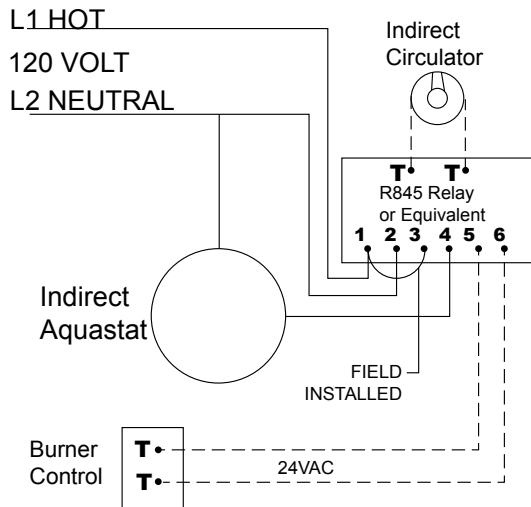
Figure 8. Boiler
