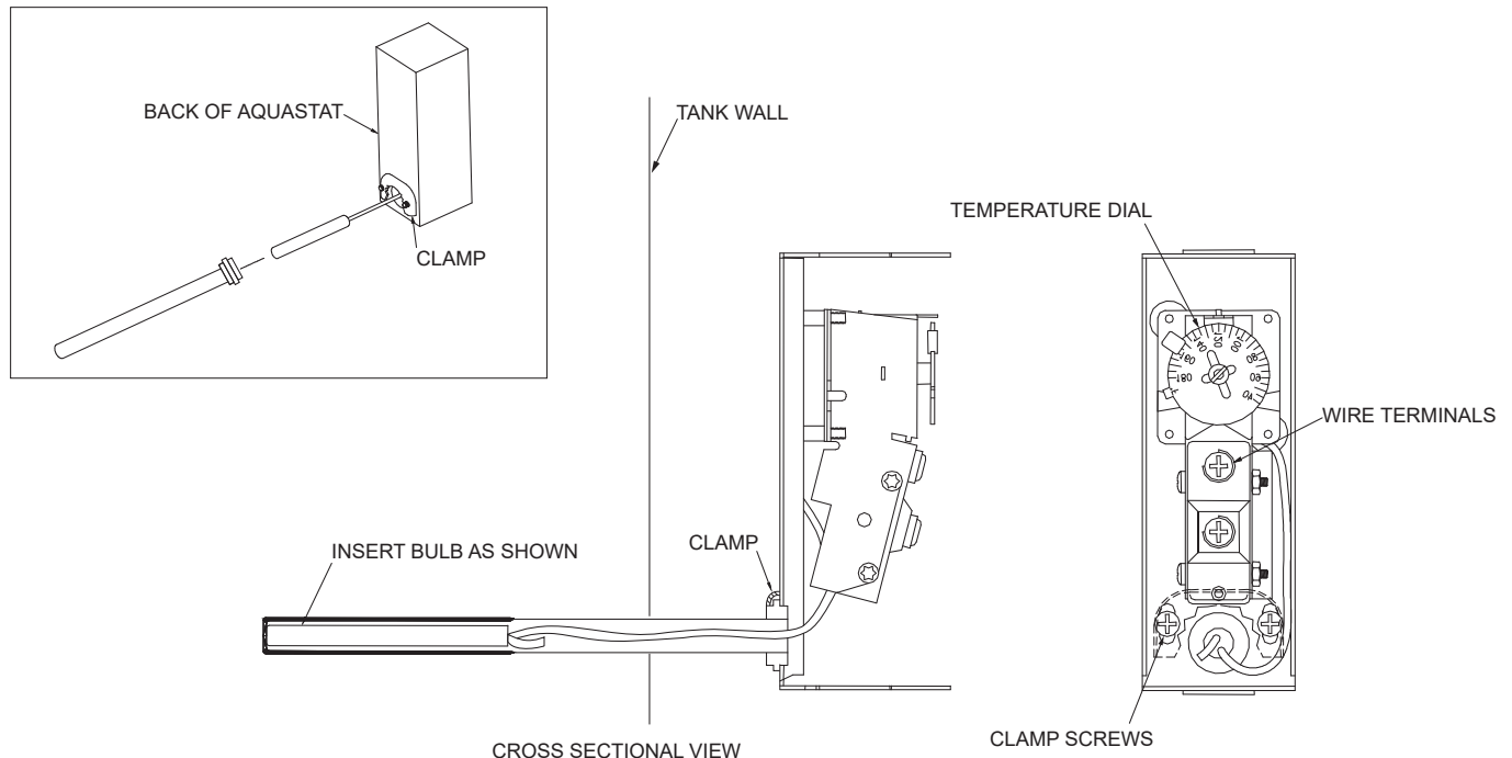
Figure 6. Aquastat Well
