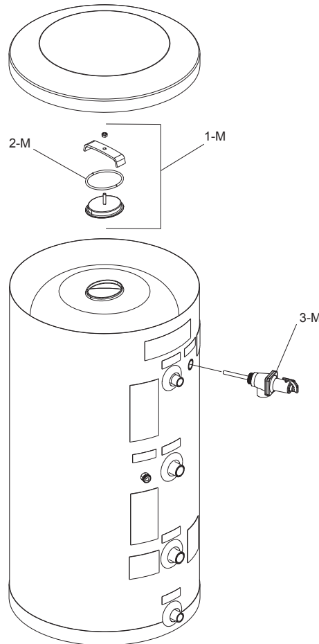
Figure 9. Replacement Parts
