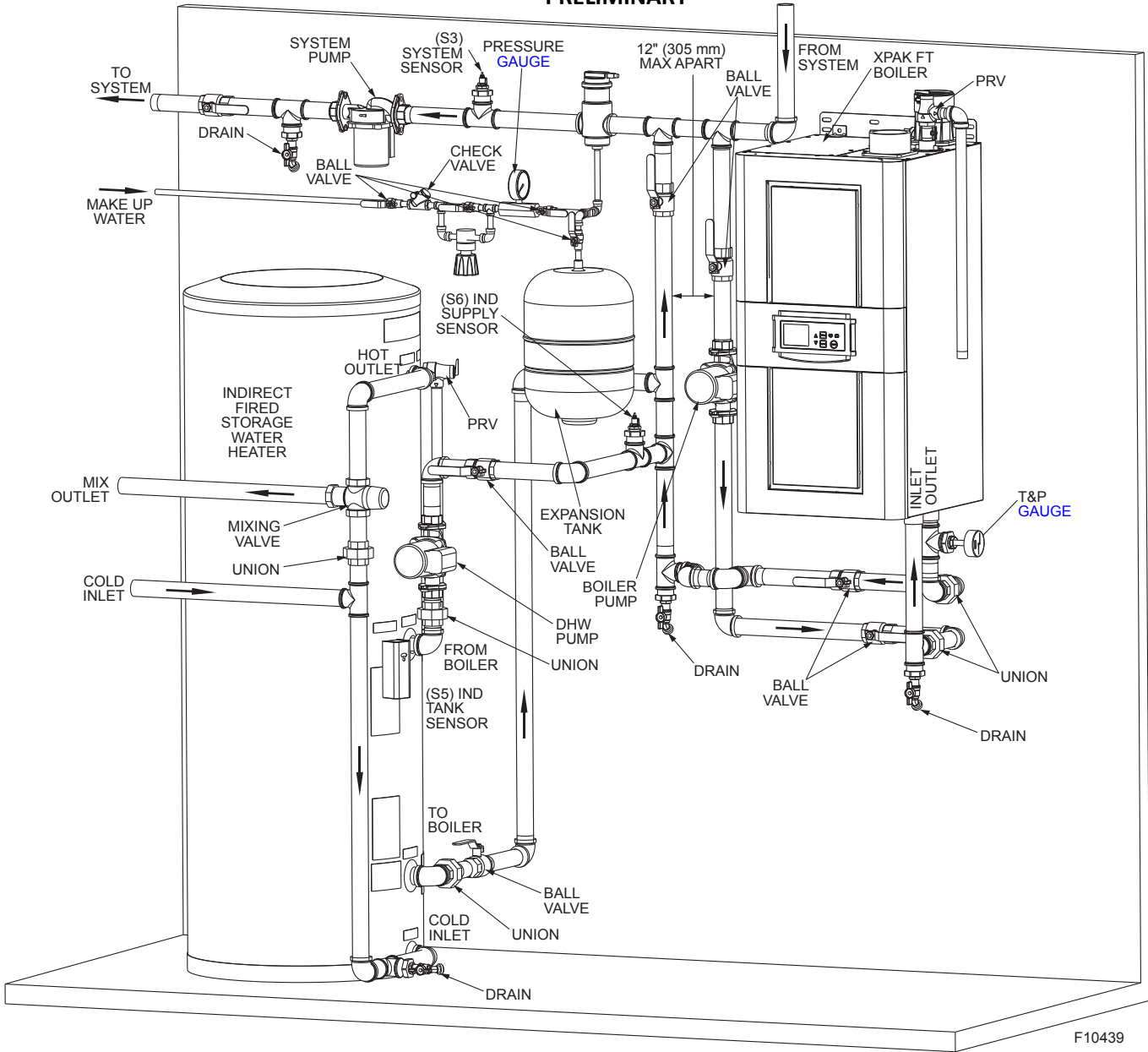
Figure 4. VERSA Mode 3
