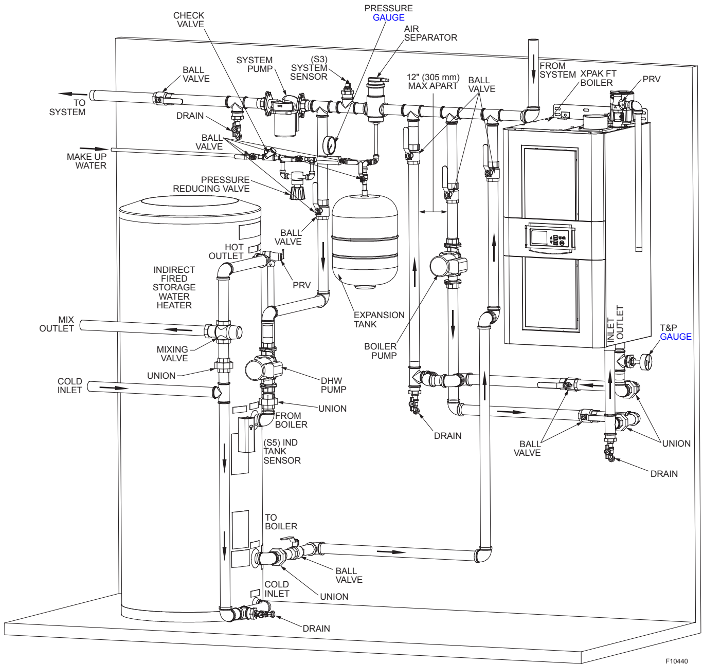
Figure 3. VERSA Mode 2
