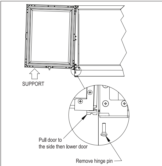
Figure 3. Door Removal
