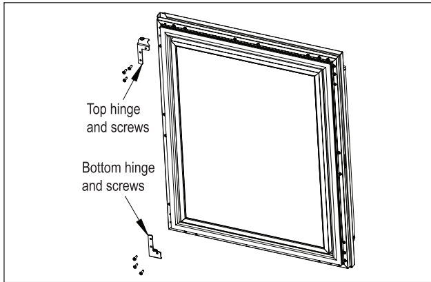
Figure 9. Door Hinges
