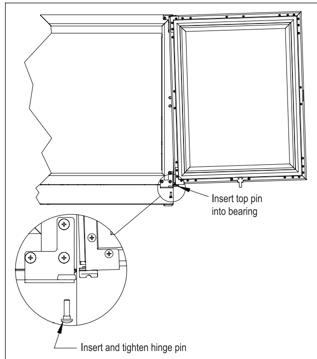
Figure 11. Installing Door
