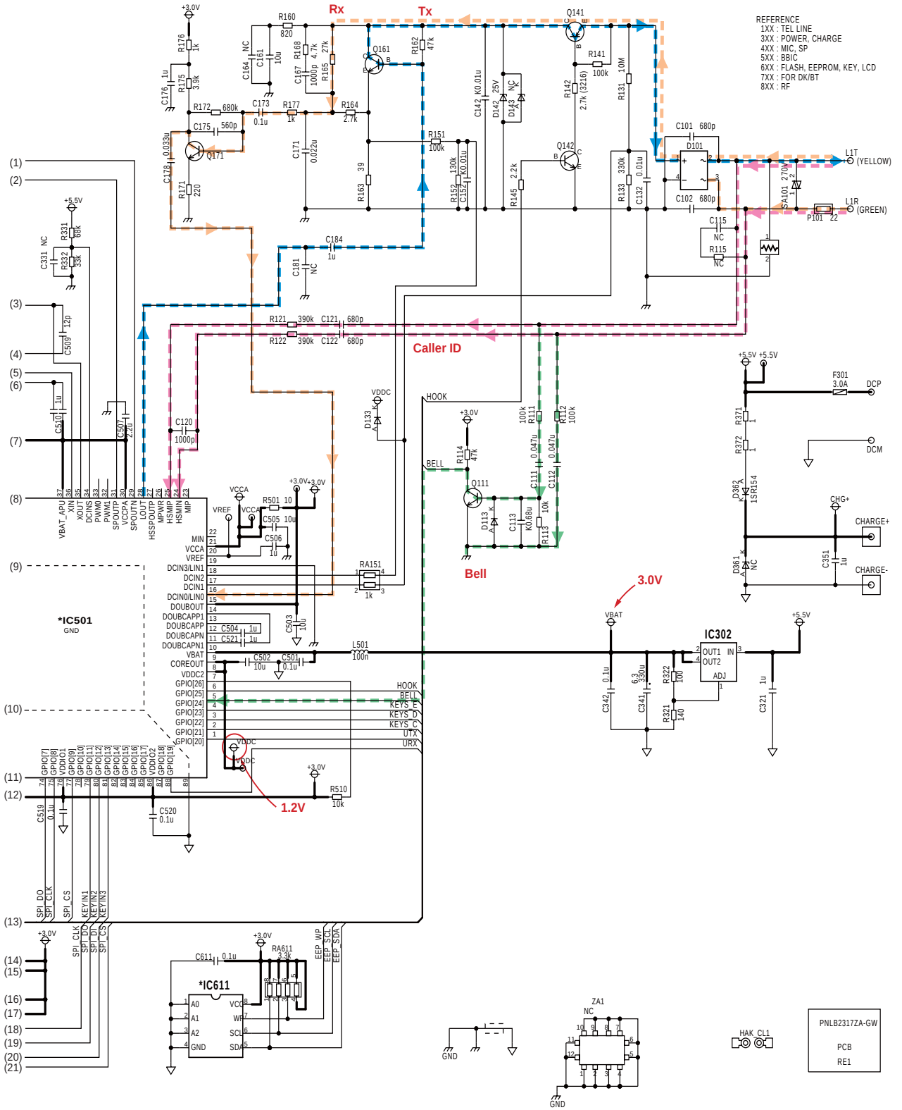
KX-TGD210 SCHEMATIC DIAGRAM (Base Unit_Main)
