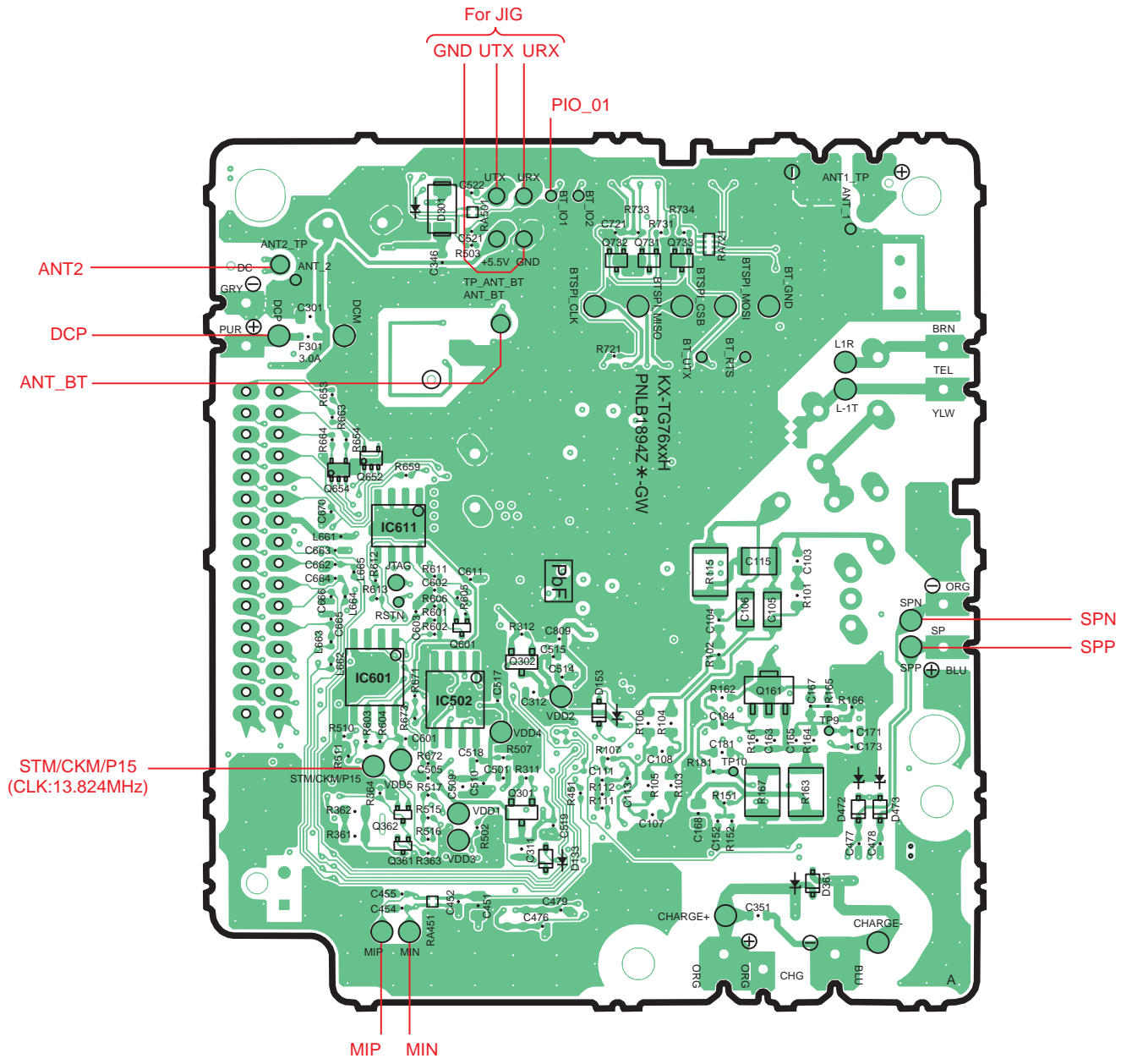
KX-TG155 CIRCUIT BOARD (Base Unit_Main (Bottom View))
