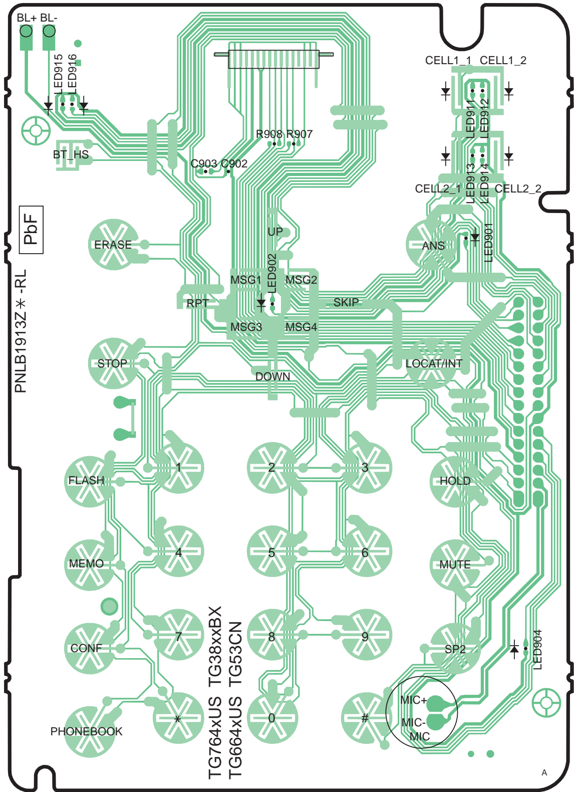
KX-TG155 CIRCUIT BOARD (Base Unit_Operation (Component View))
