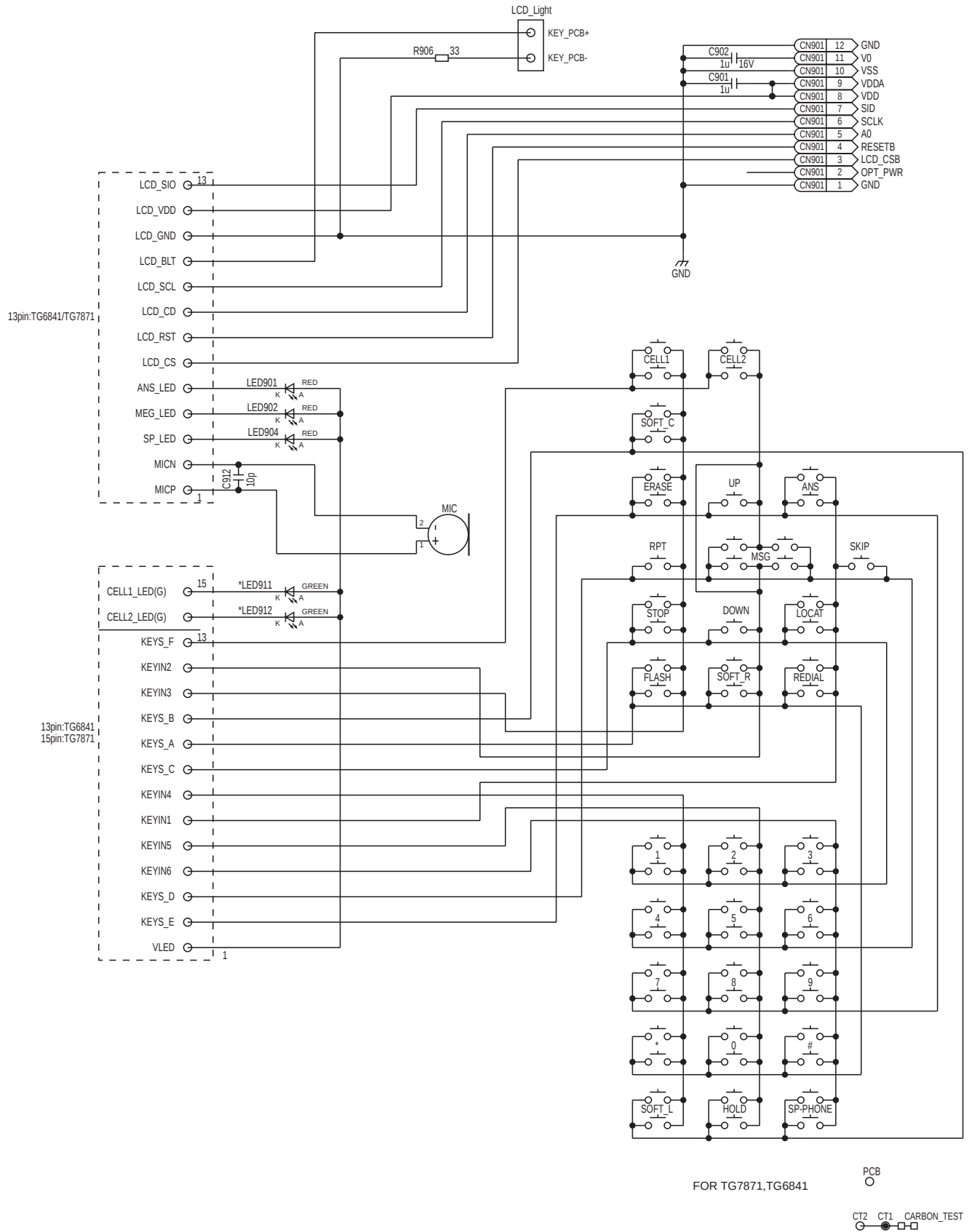
KX-TG6841/6842/6843/6844/6845/6873 SCHEMATIC DIAGRAM (Base Unit_Operation)
