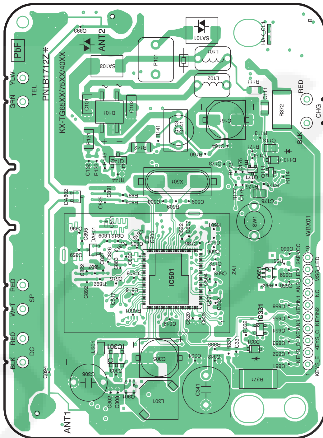
KX-TG6572 CIRCUIT BOARD (Base Unit_Main (Bottom View))
