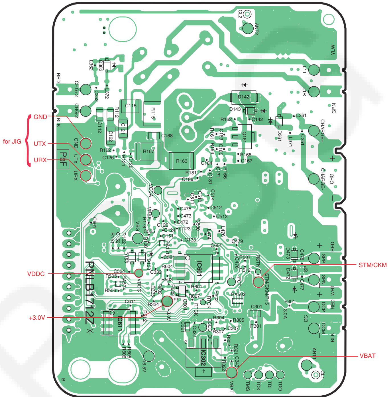
KX-TG6572 CIRCUIT BOARD (Base Unit_Main (Component View))
