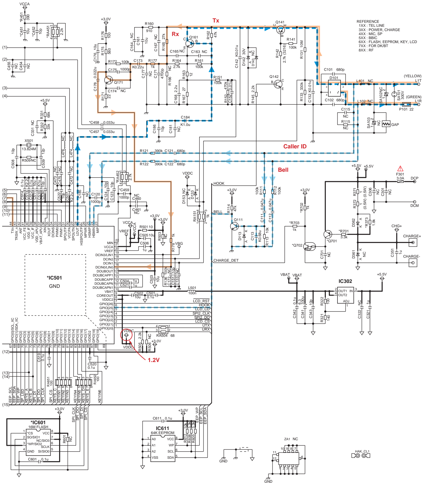
NC: No Components KX-TG4763 SCHEMATIC DIAGRAM (Base Unit_Main)
