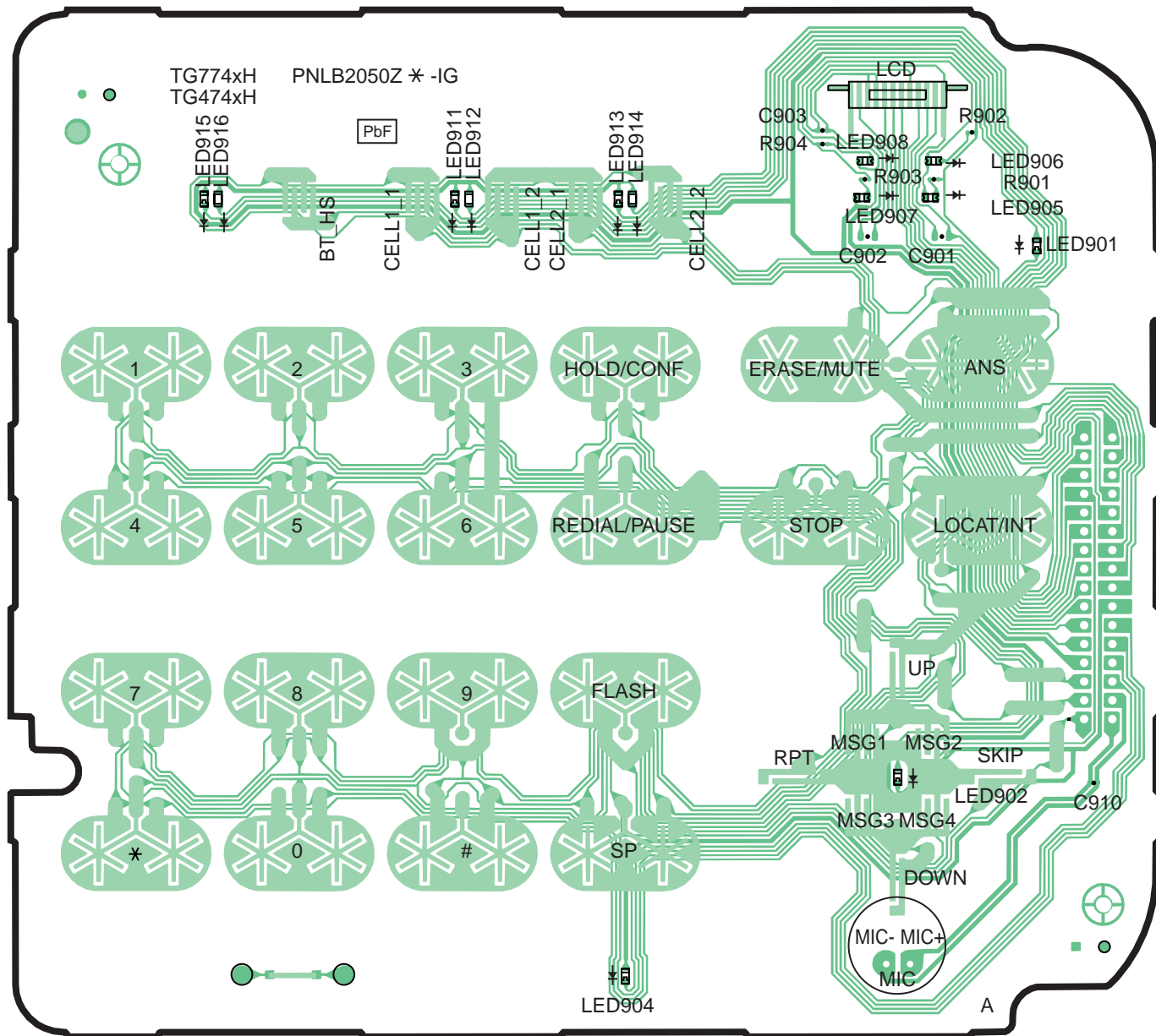
KX-TG4763 CIRCUIT BOARD (Base Unit_Operation (Component View))
