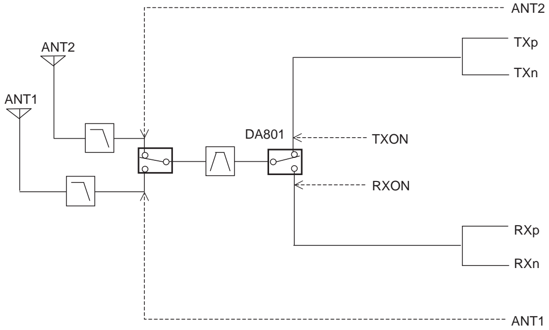
KX-TG4763 BLOCK DIAGRAM (Base Unit_RF Part)
