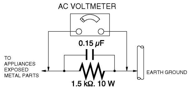
Hot-Check Circuit
