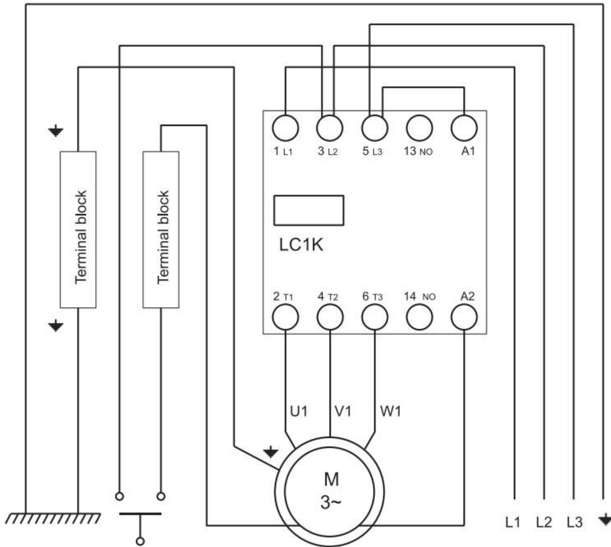
Motor with internal thermo protection
