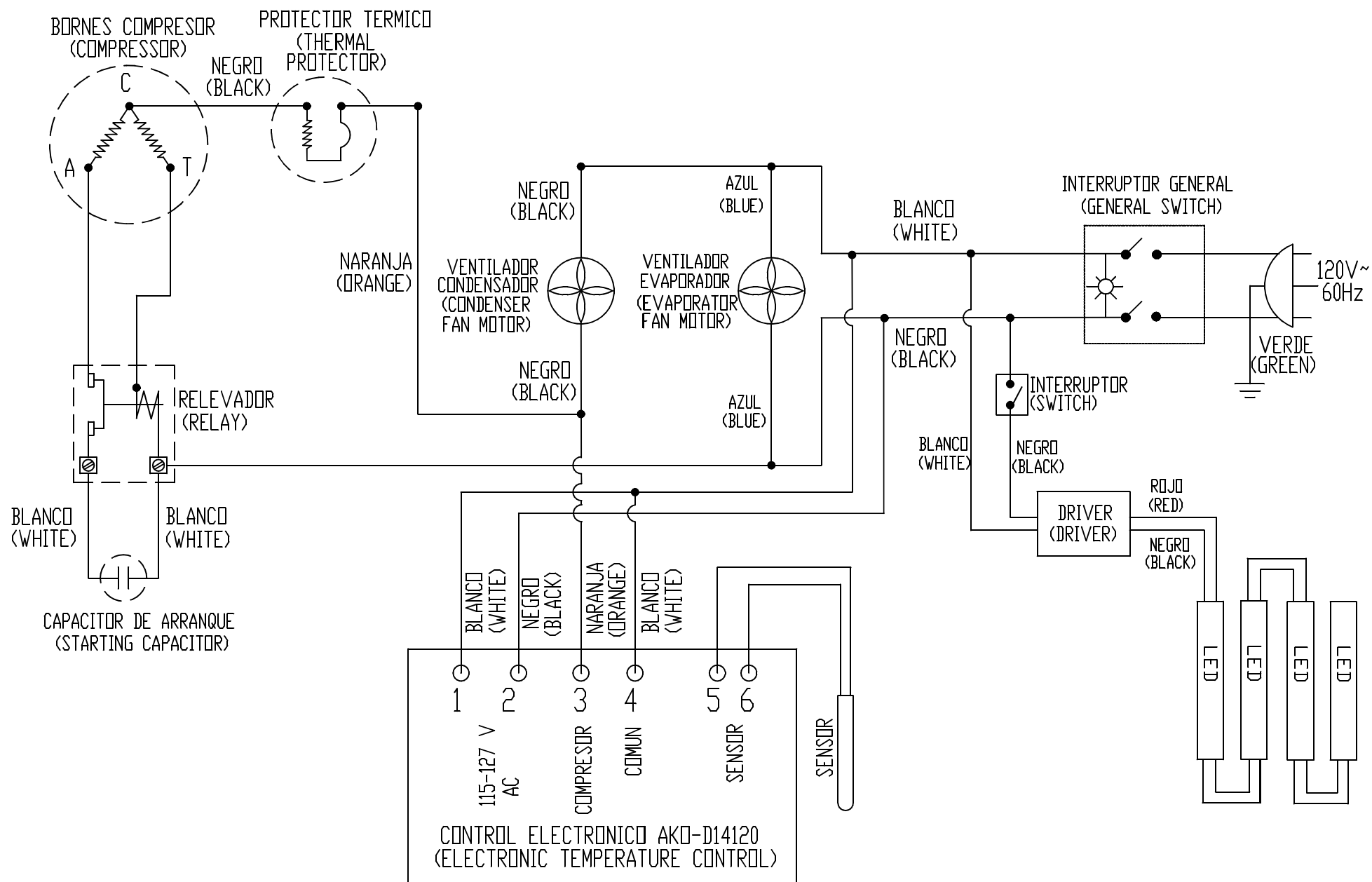
DIAGRAMA ELECTRICO (ELECTRIC DIAGRAM) RMH-33-PT-54
