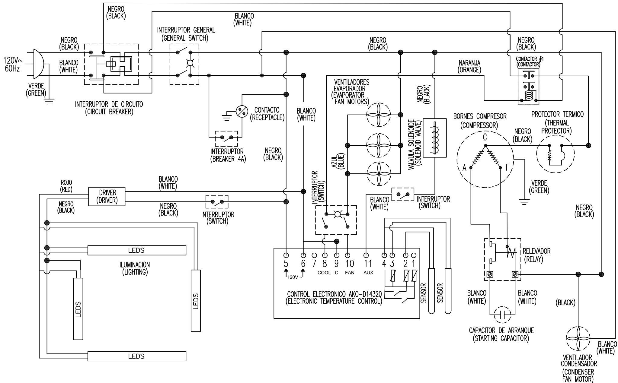
DIAGRAMA ELECTRICO (ELECTRIC DIAGRAM)
