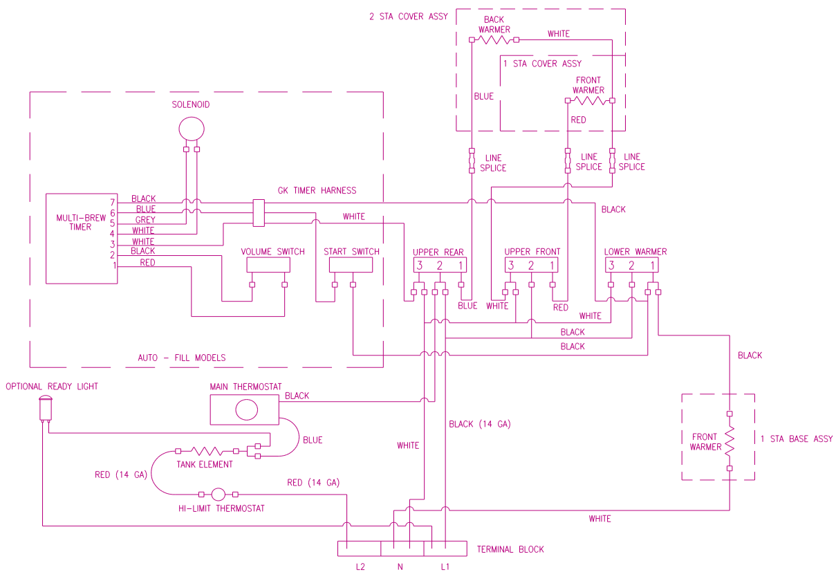
GK Series Brewer - 120 V / 240 V
