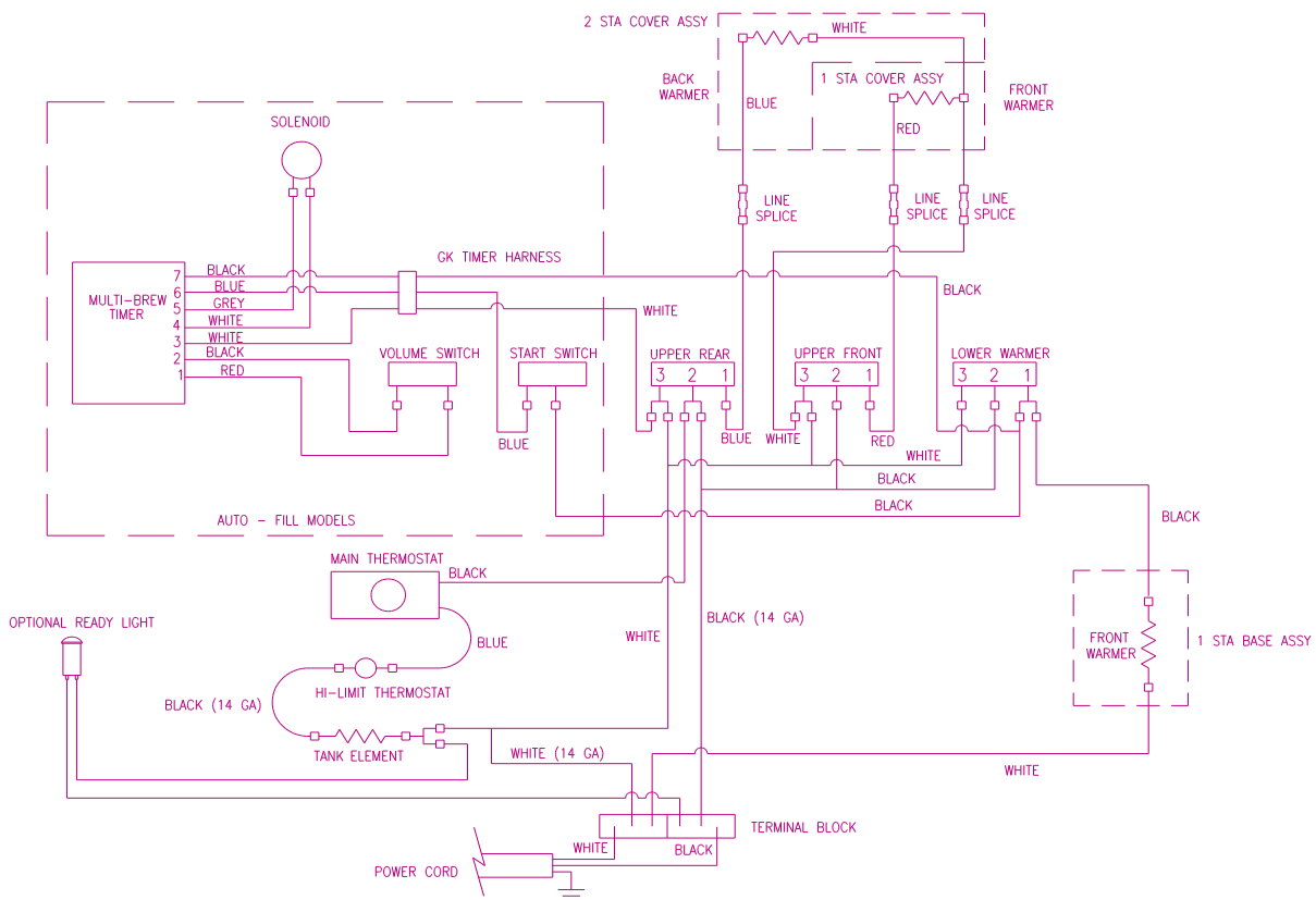
GK Series Brewer - 120 V
