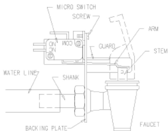
Micro Switch Section View
