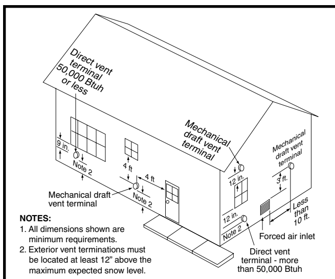
Figure 8. Vent Locations
