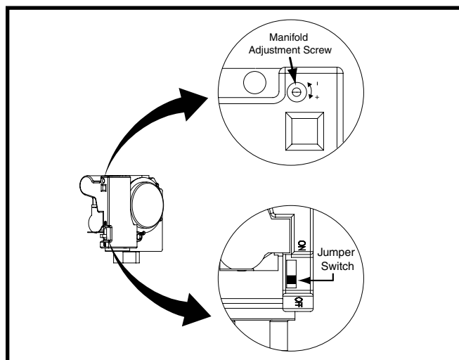
Figure 21. Modulating Gas Valve
