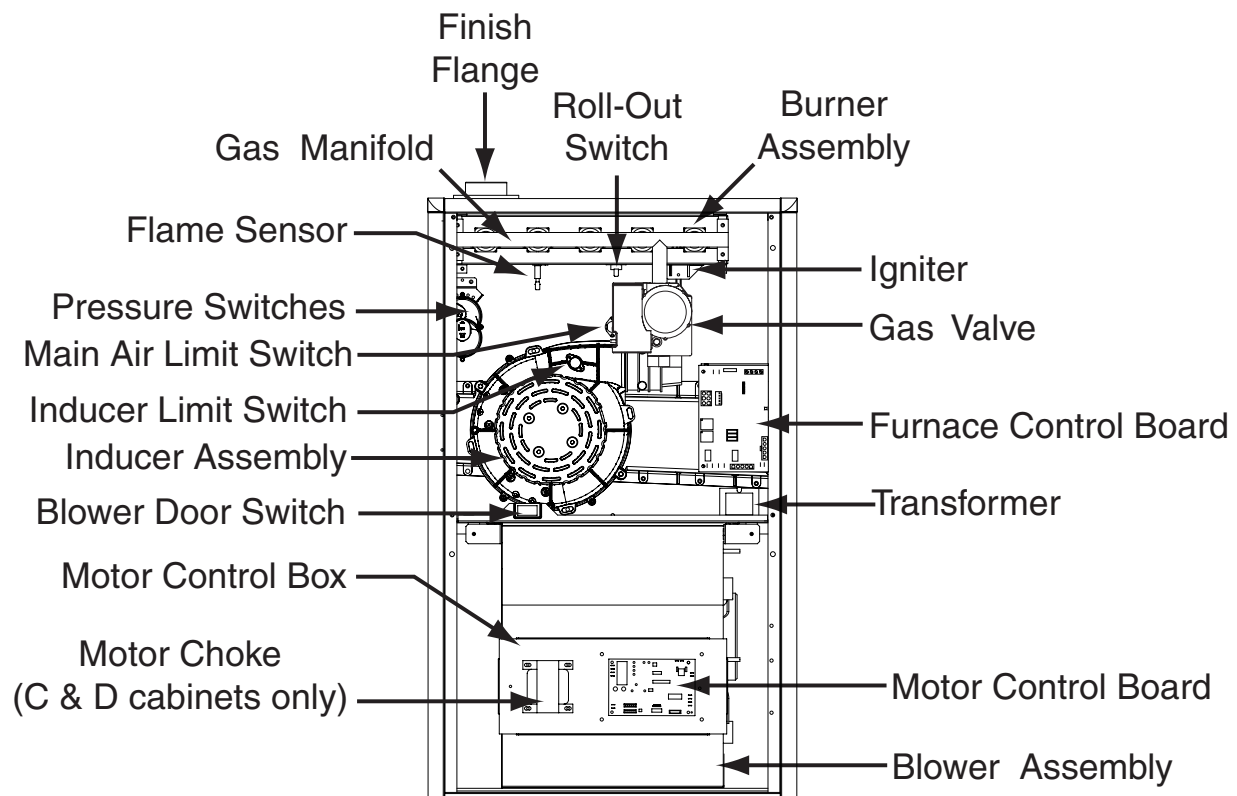
Figure 29. Component Locations
