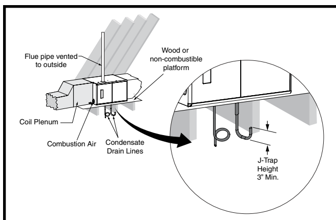
Figure 11. Horizontal installation on a Platform
