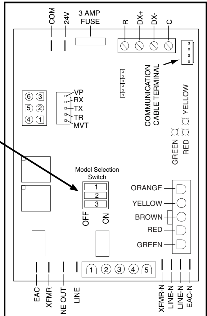
Figure 24. Modulating Furnace Control Board
