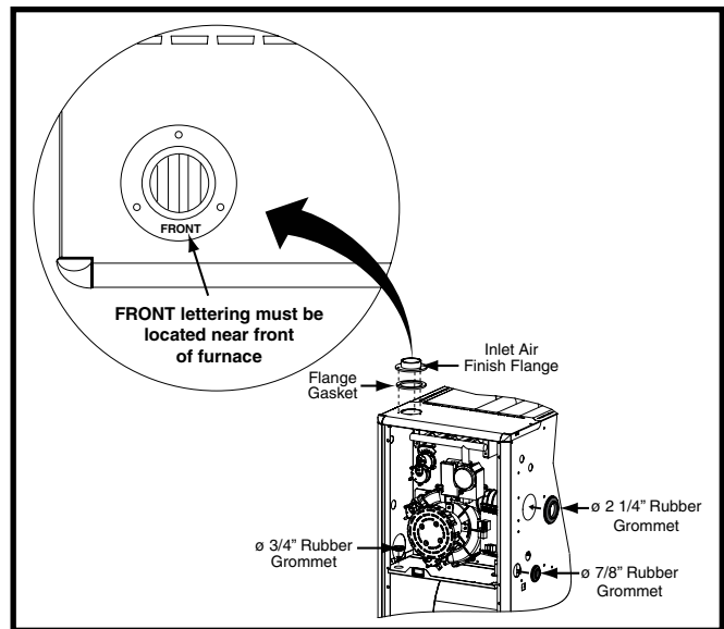
Figure 15. Rubber Grommets
