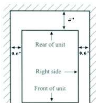
INSTALLATION CLEARANCES: TOP VIEW
