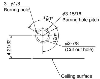
Fresh air intake hole diagram (Unit : inch)
