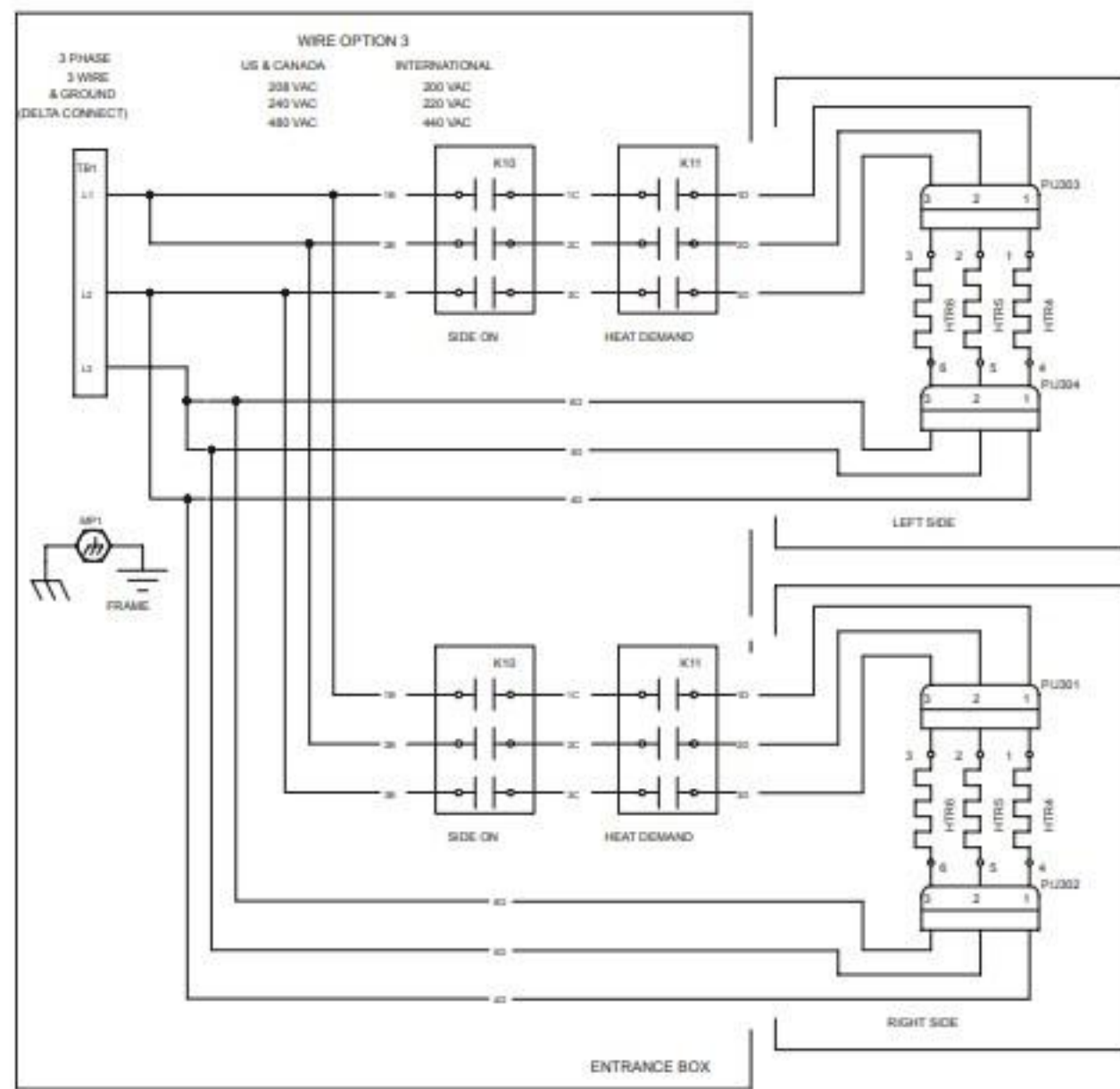
SPLIT VAT- DELTA LOAD CONNECTION
