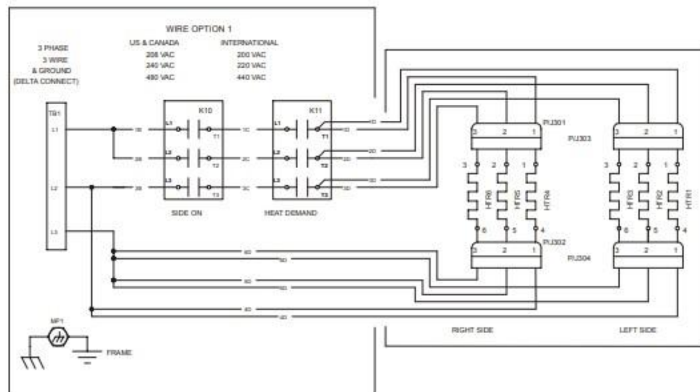
SINGLE VAT- DELTA LOAD CONNECTION
