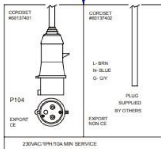
CORD BOX EXPORT NO HOOD CONTROL
