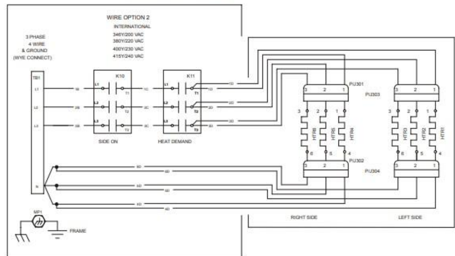
SINGLE VAT- WYE LOAD CONNECTION
