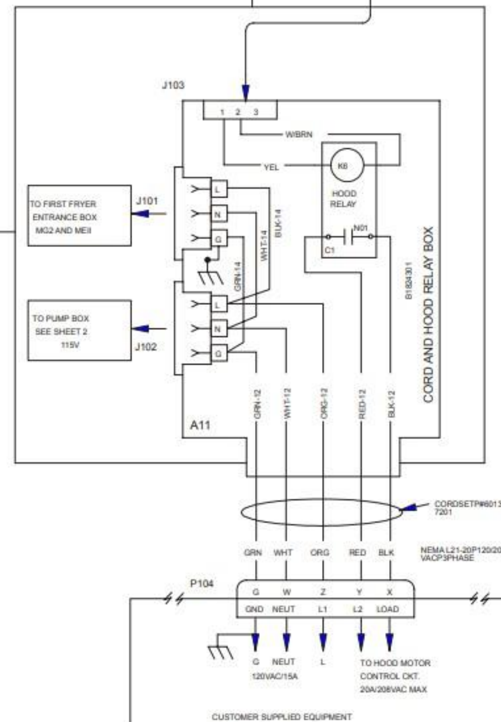
CORD BOX WITH HOOD CONTROL DOMESTIC ONLY
