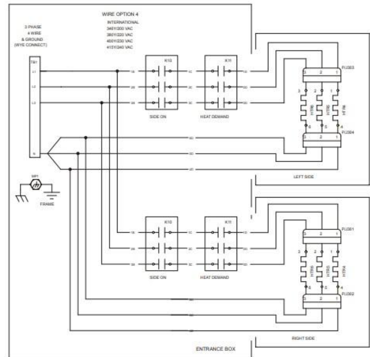
SPLIT VAT- WYE LOAD CONNECTION
