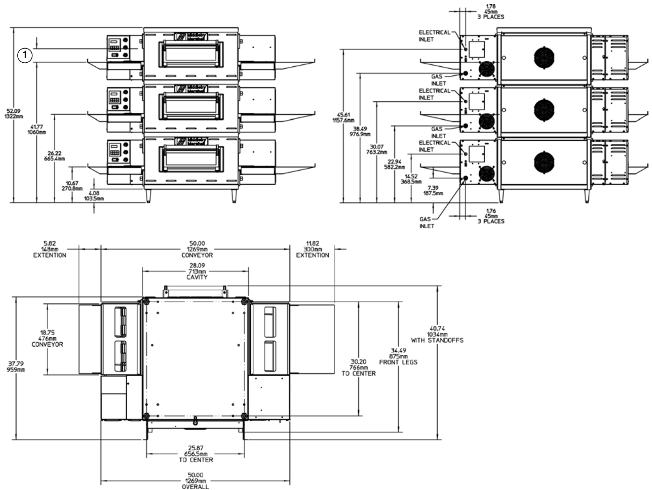
Figure 2-7. MODEL 528 TRIPLE OVEN DIMENSIONS
