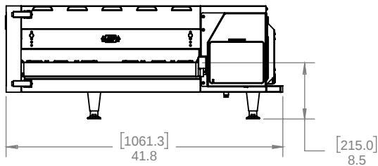
Figure 1: PS2620 Oven Dimensions – Side
