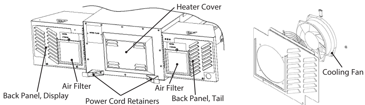
Figure B-3: Rear Oven Components
