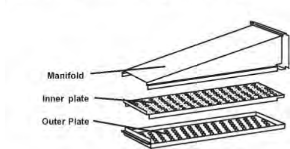
Figure 4-3. Disassembling the Air Fingers
