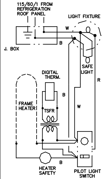
WIRING DIAGRAM CM-156-75
