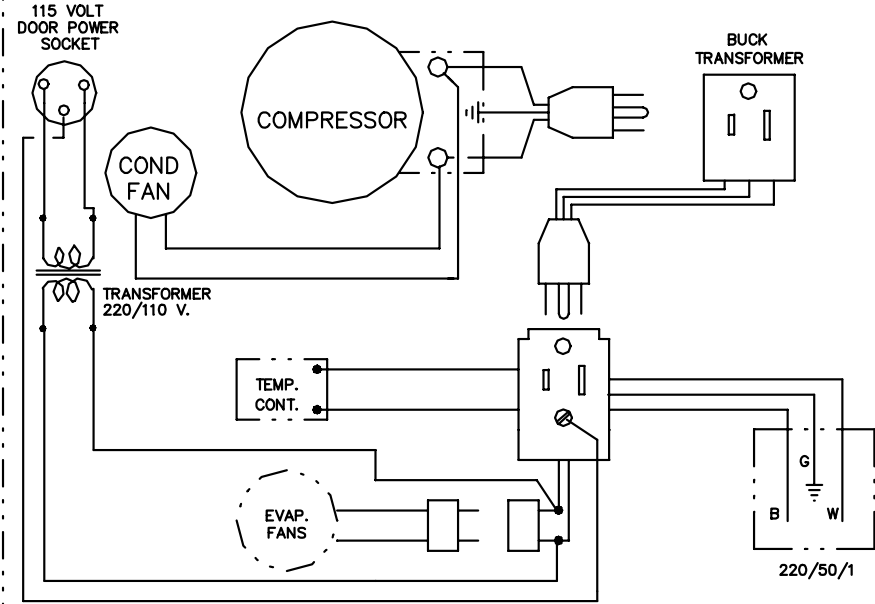
WIRING DIAGRAM 220/50/1 W\ BUCK TRANSF.
