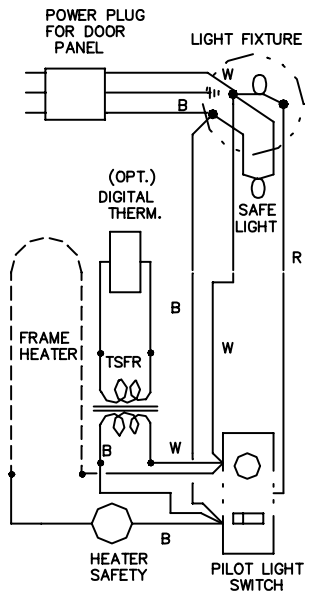
WIRING DIAGRAM CM-3-(1/3 & 1/2)
