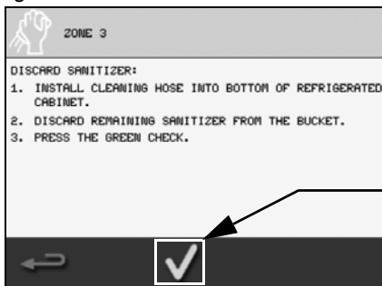
Discard Sanitizer Screen
