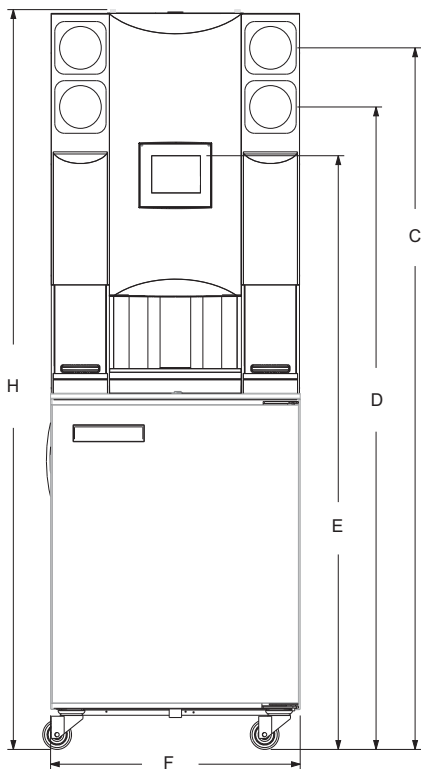
Elevation View
