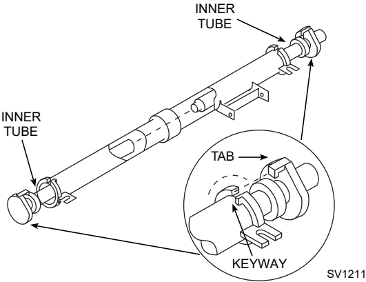
Q210/Q270 Water Distribution Tube Disassembly
