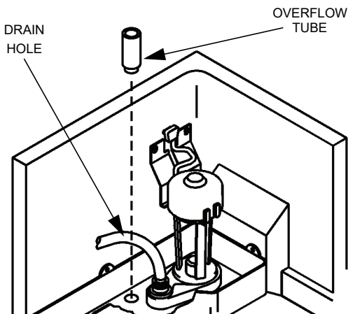
Removing the Overflow Tube
