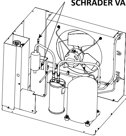
ALTERNATE CONNECTIONS AT CONDENSING UNIT SCHRAEDER VALVES
