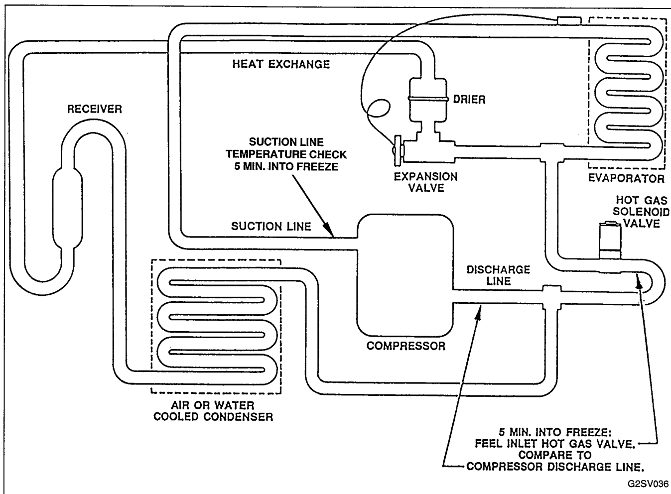
FIGURE 36. HOT GAS VALVE INLET FEEL CHECK/SUCTION LINE TEMPERATURE CHECK
