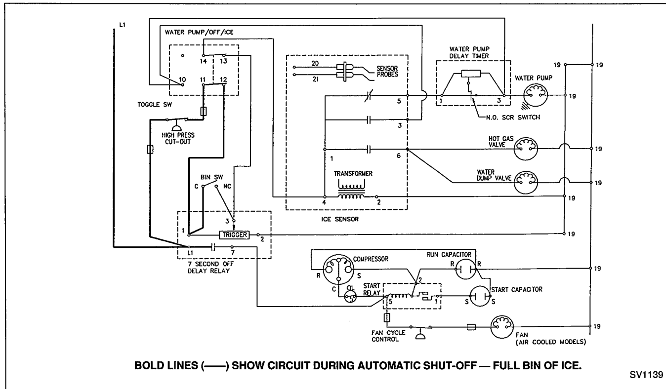
FIGURE 24. AUTOMATIC SHUT-OFF ELECTRICAL SEQUENCE
