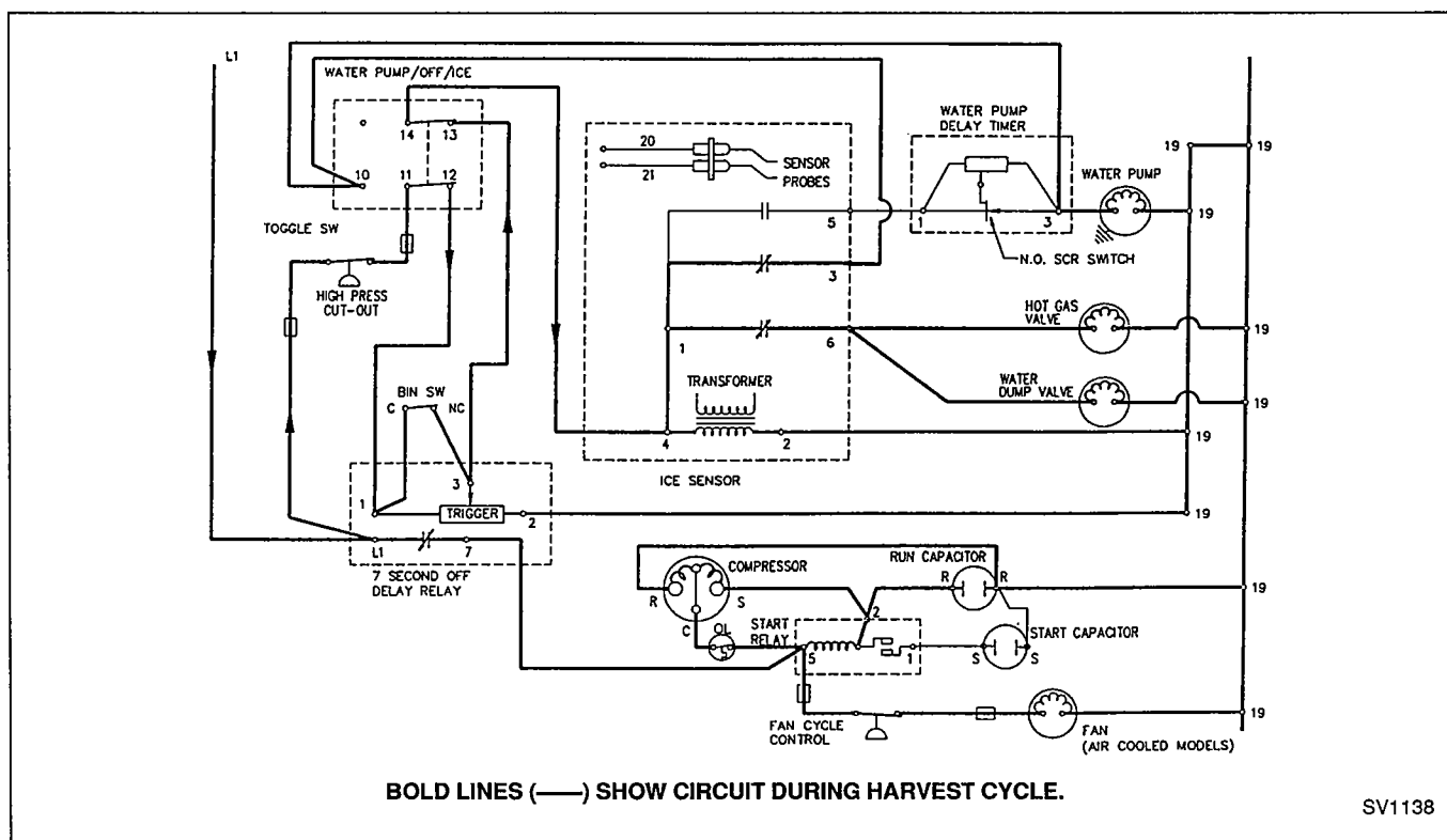
FIGURE 21. HARVEST CYCLE ELECTRICAL SEQUENCE
