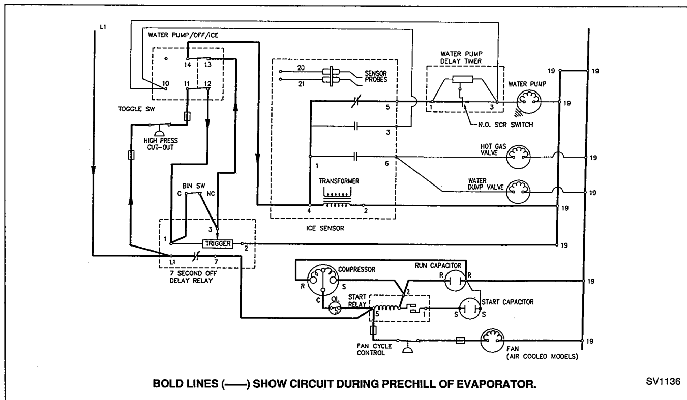
FIGURE 16. PRECHILL ELECTRICAL SEQUENCE
