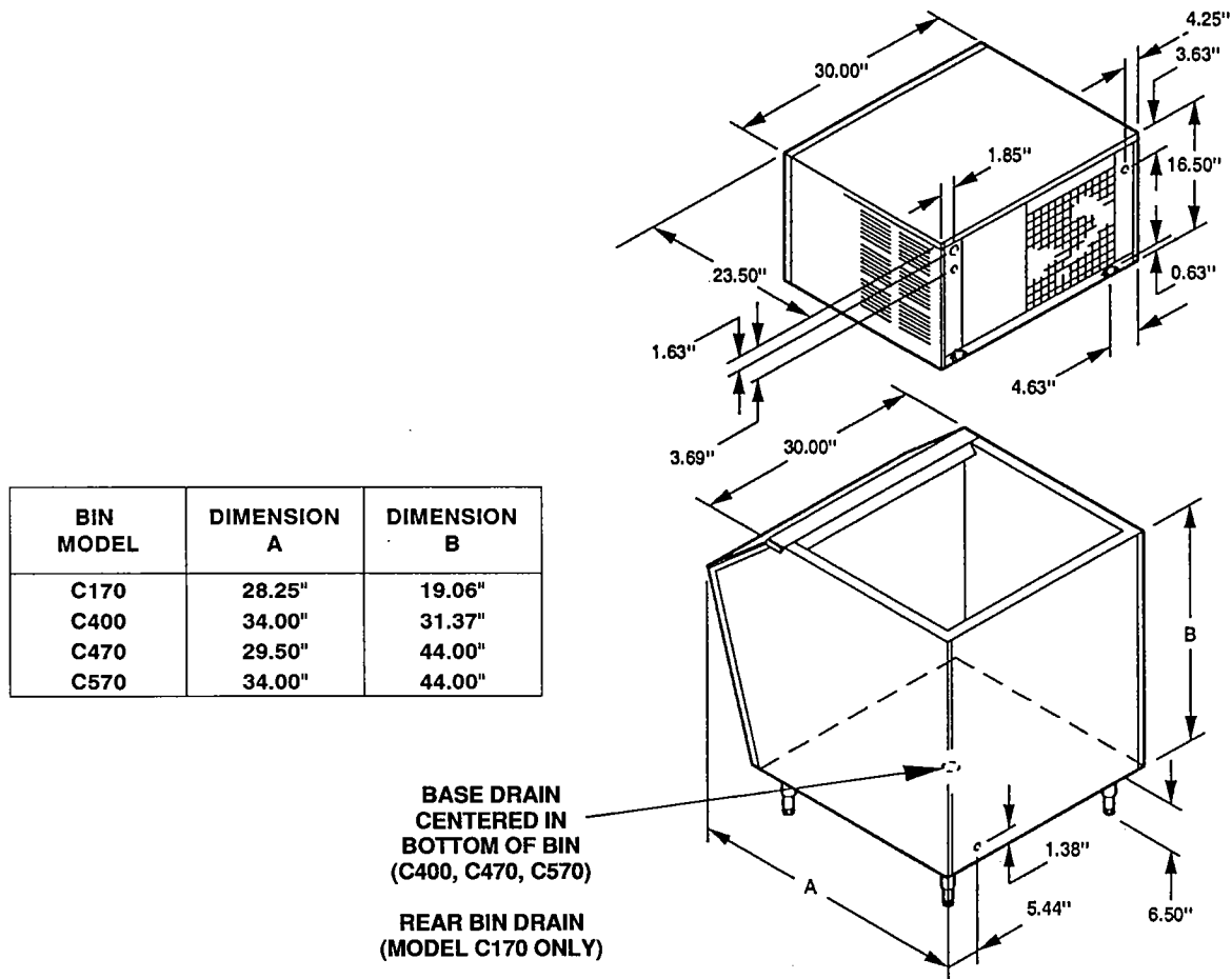
FIGURE 2. DIMENSIONS
