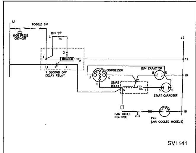
FIGURE 30. 7-SECOND OFF DELAY RELAY
