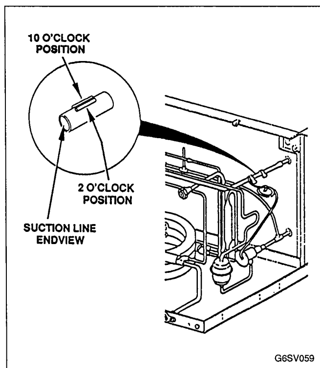
FIGURE 39. TXV BULB LOCATION
