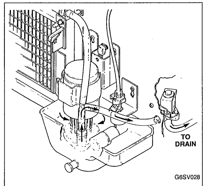
FIGURE 23. HARVEST CYCLE WATER FLOW SEQUENCE
