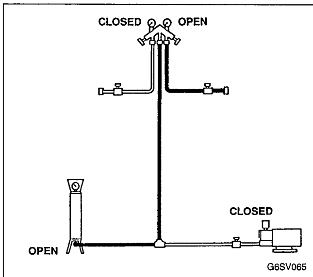
FIGURE 45. RECHARGING OF SELF-CONTAINED SYSTEMS
