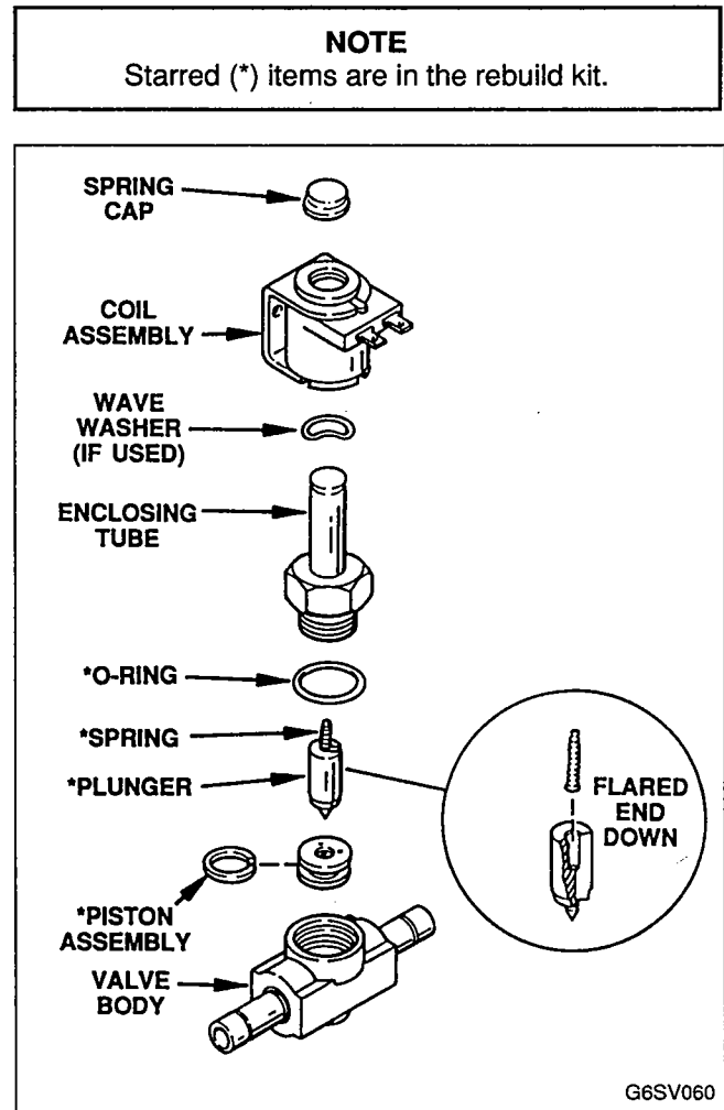
FIGURE 40. REFRIGERATION SOLENOID VALVE
