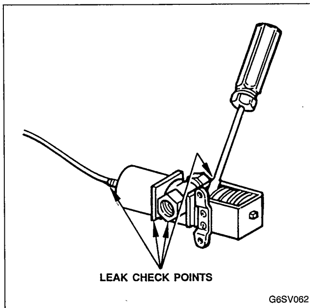
FIGURE 42. WATER REGULATING VALVE LEAK CHECK POINTS
