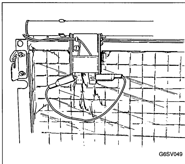
FIGURE 32. JUMPER WIRE CONNECTED TO PROBES
