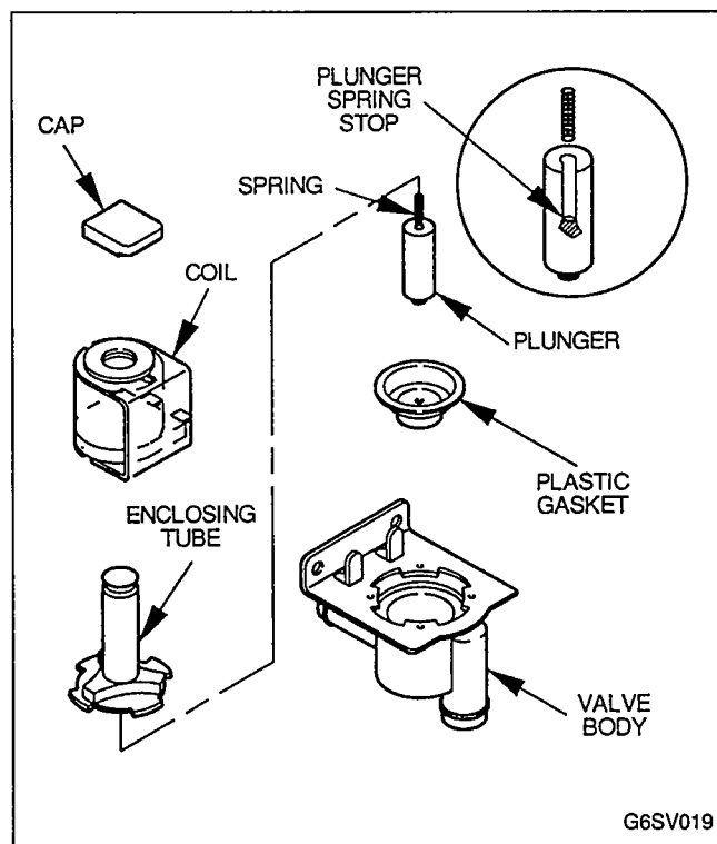
FIGURE 15. WATER DUMP VALVE DISASSEMBLY
