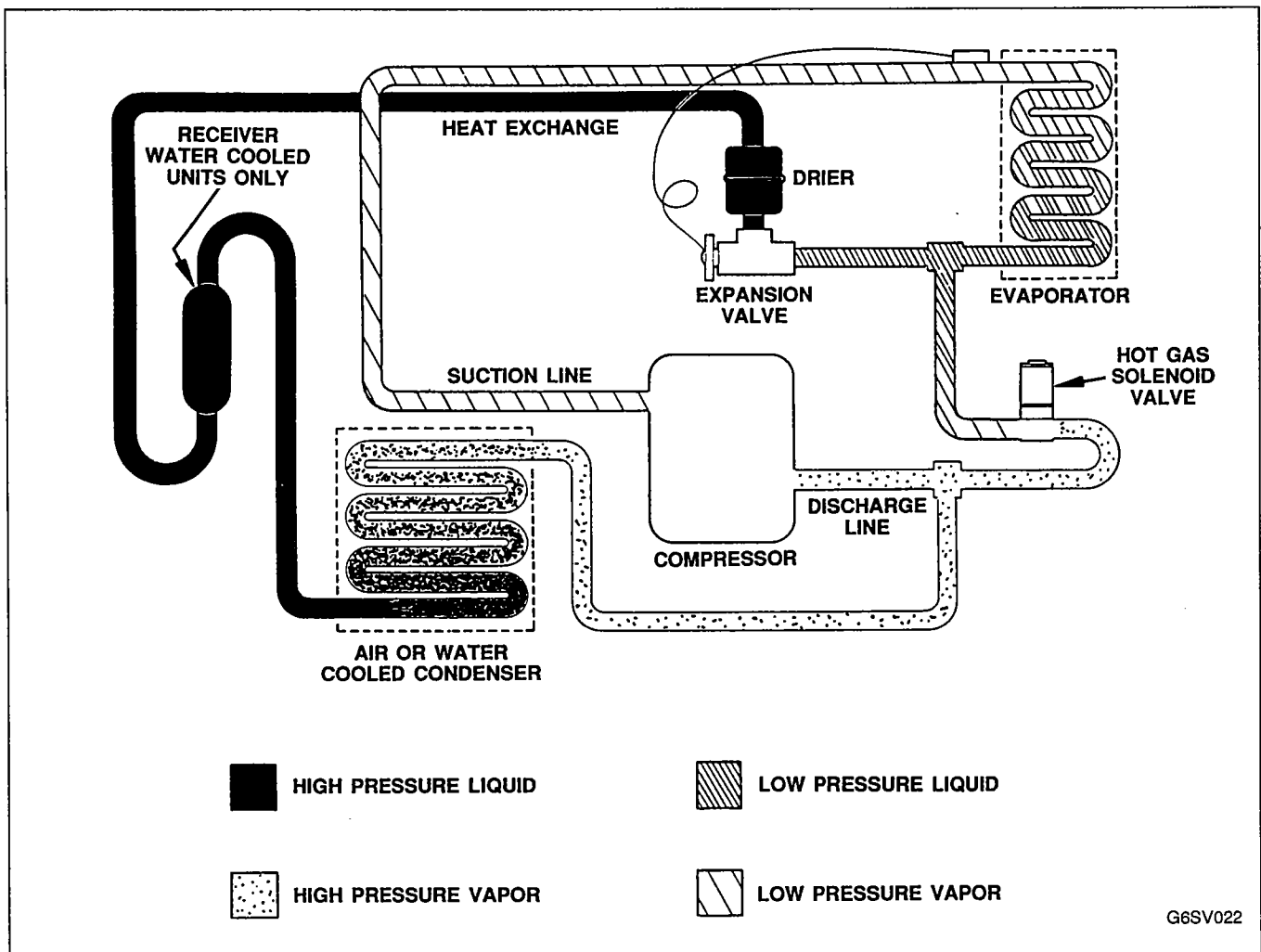
FIGURE 17. PRECHILL REFRIGERATION SEQUENCE
