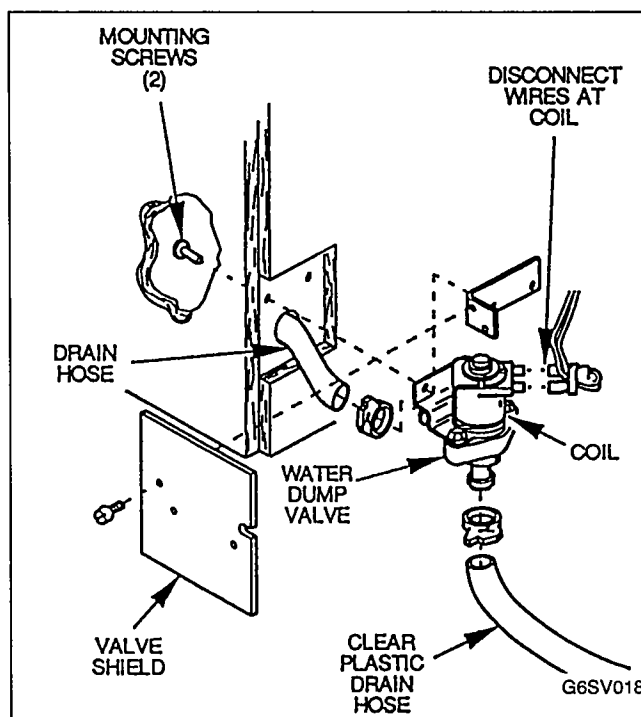
FIGURE 14. WATER DUMP VALVE REMOVAL
