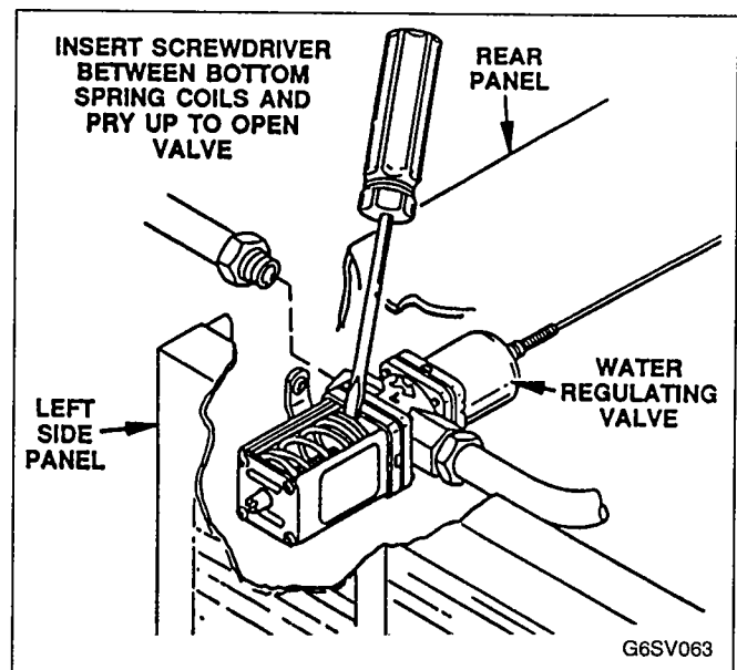
FIGURE 43. MANUALLY OPENING WATER REGULATING VALVE
