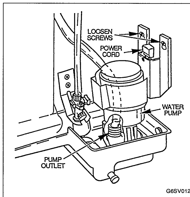
FIGURE 8. WATER PUMP REMOVAL
