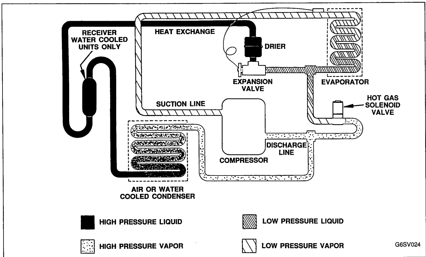
FIGURE 19. FREEZE CYCLE REFRIGERATION SEQUENCE
