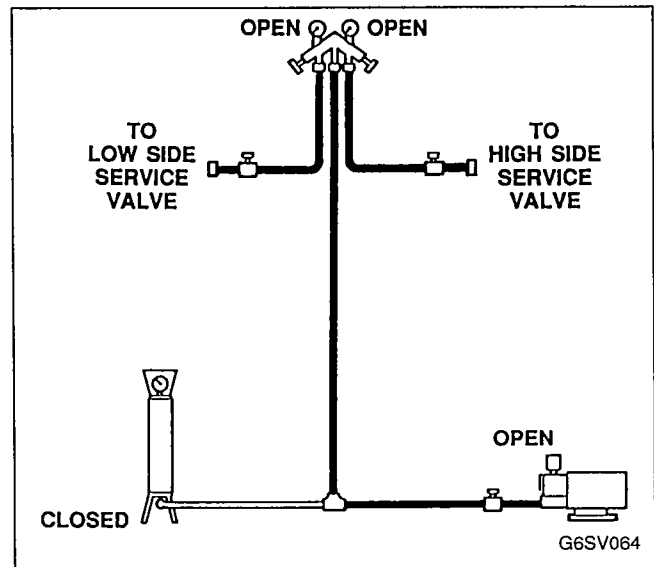
FIGURE 44. EVACUATION OF SELF-CONTAINED SYSTEMS
