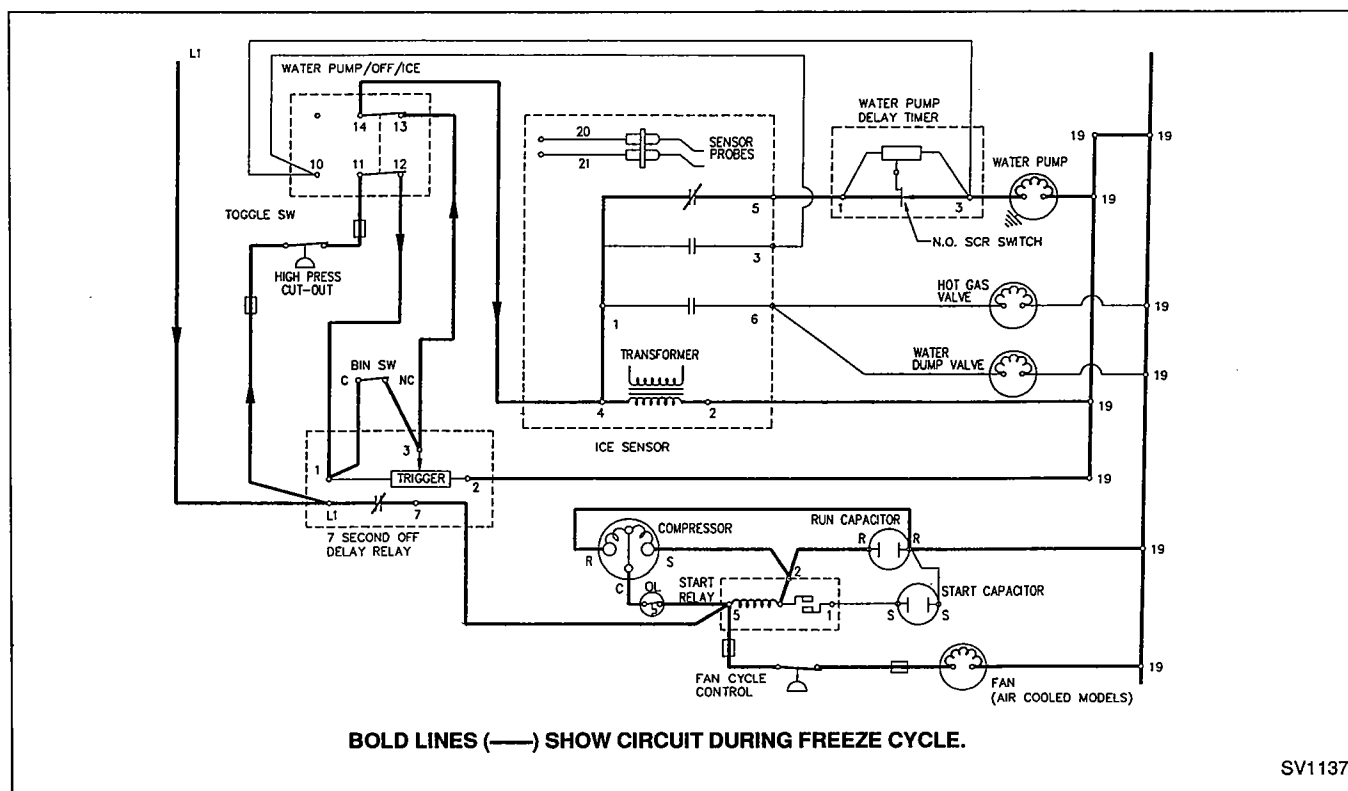
FIGURE 18. FREEZE CYCLE ELECTRICAL SEQUENCE
