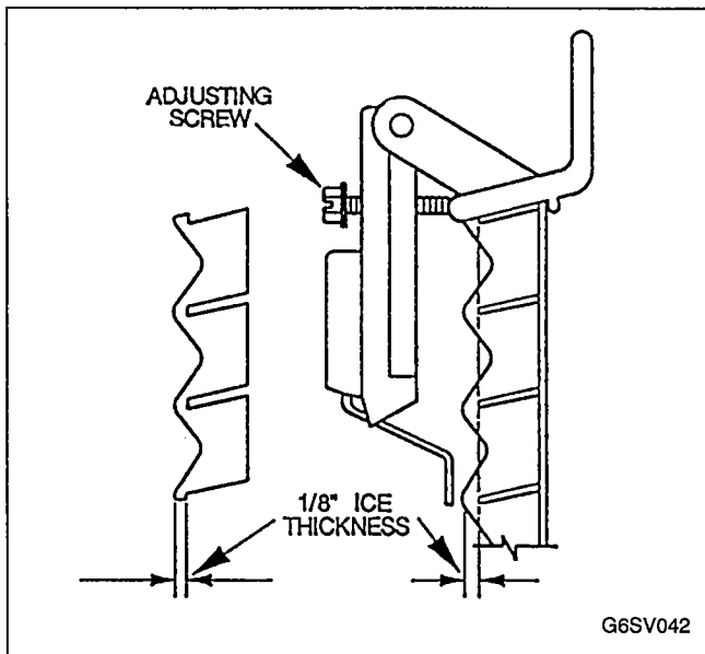
FIGURE 27. ICE THICKNESS CHECK
