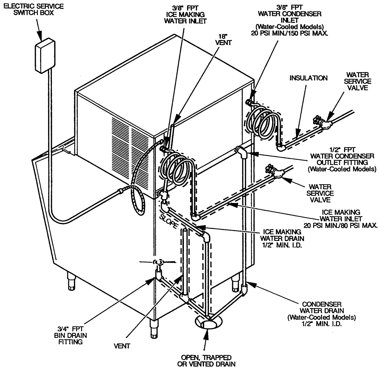
FIGURE 3. TYPICAL INSTALLATION
