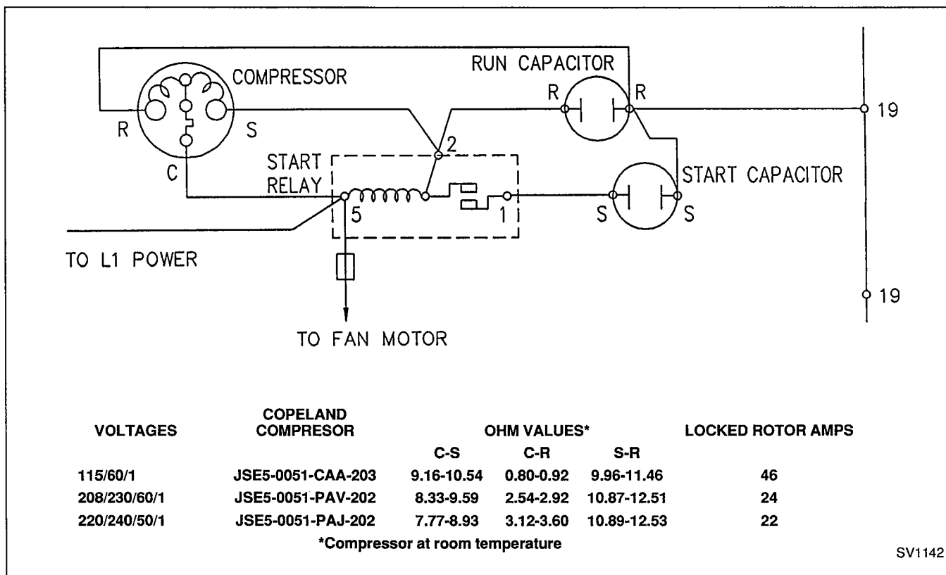
FIGURE 34. COMPRESSOR AND START COMPONENTS SCHEMATIC
