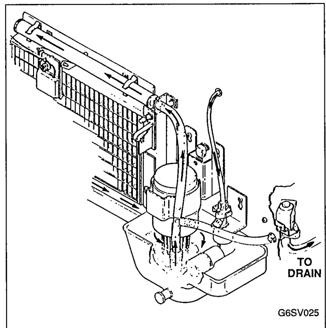
FIGURE 20. FREEZE CYCLE WATER FLOW SEQUENCE
