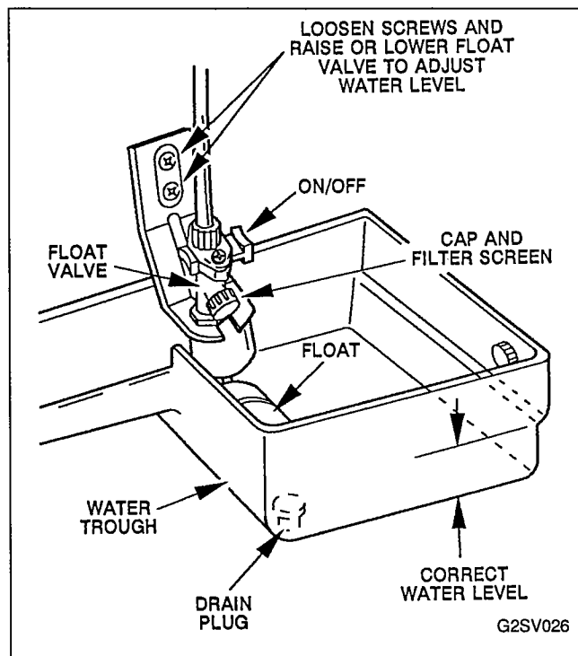
FIGURE 26. FLOAT VALVE CHECK
