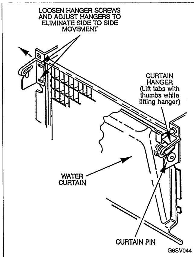
FIGURE 29. WATER CURTAIN CHECK
