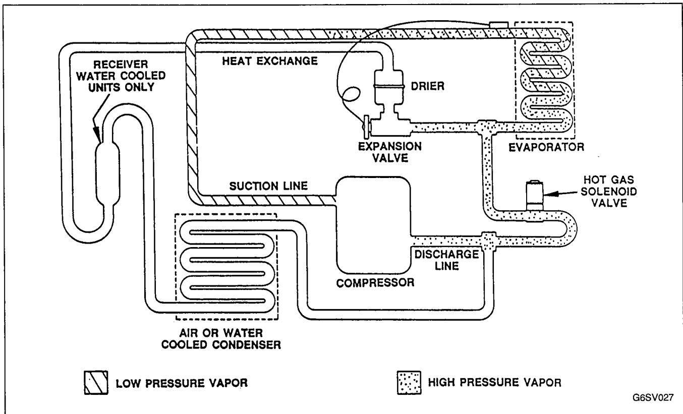
FIGURE 22. HARVEST CYCLE REFRIGERATION SEQUENCE
