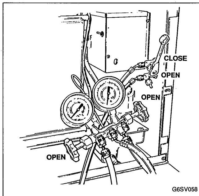
FIGURE 38. REMOVAL OF MANIFOLD GAUGES
