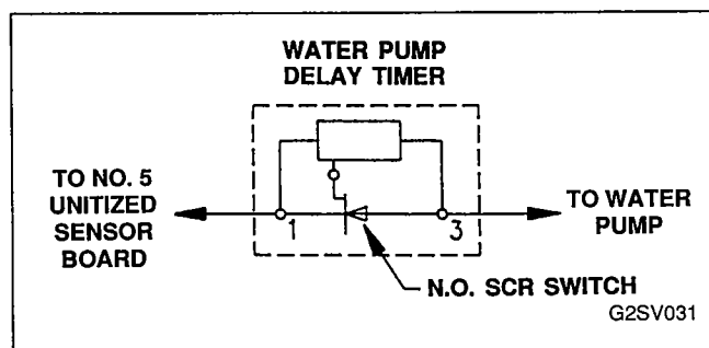
FIGURE 31. WATER PUMP DELAY TIMER CHECK
