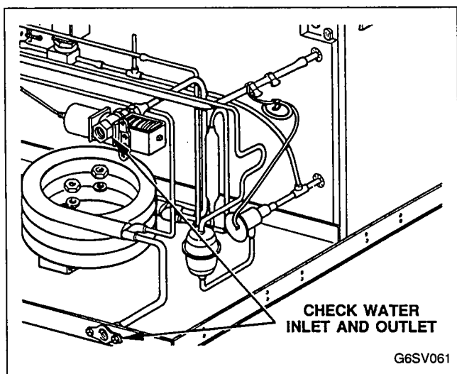
FIGURE 41. CONDENSER LEAK CHECK POINTS
