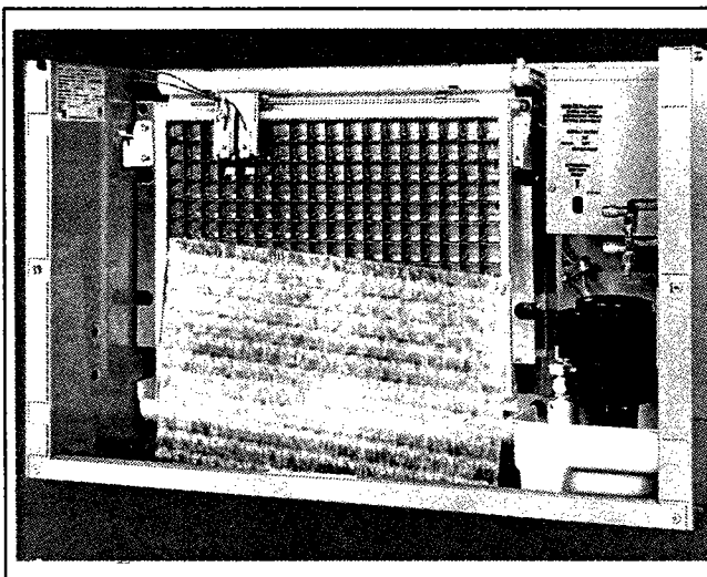
FIGURE 4. HARVEST MODE
