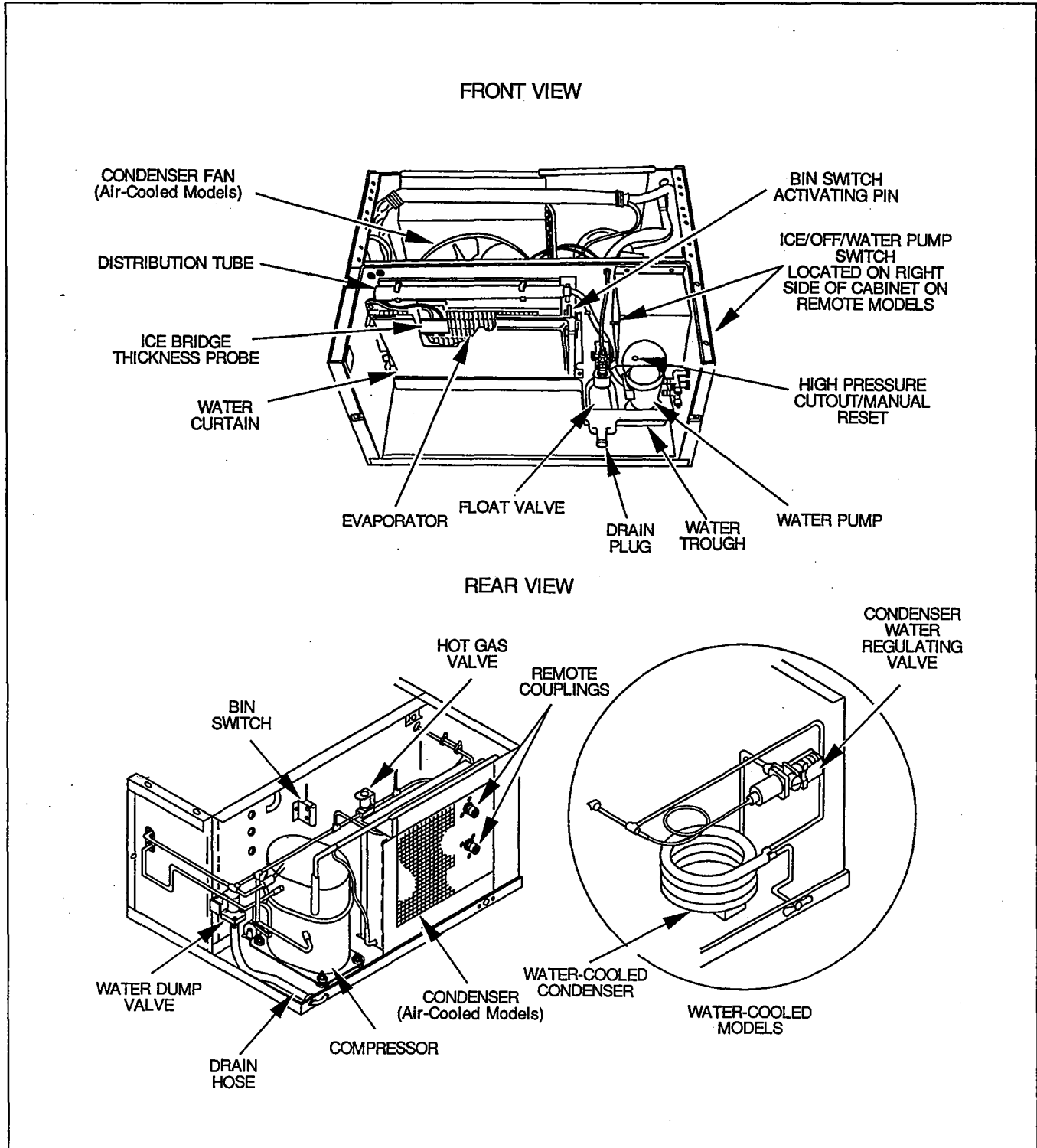
FIGURE 2. COMPONENT LOCATION
