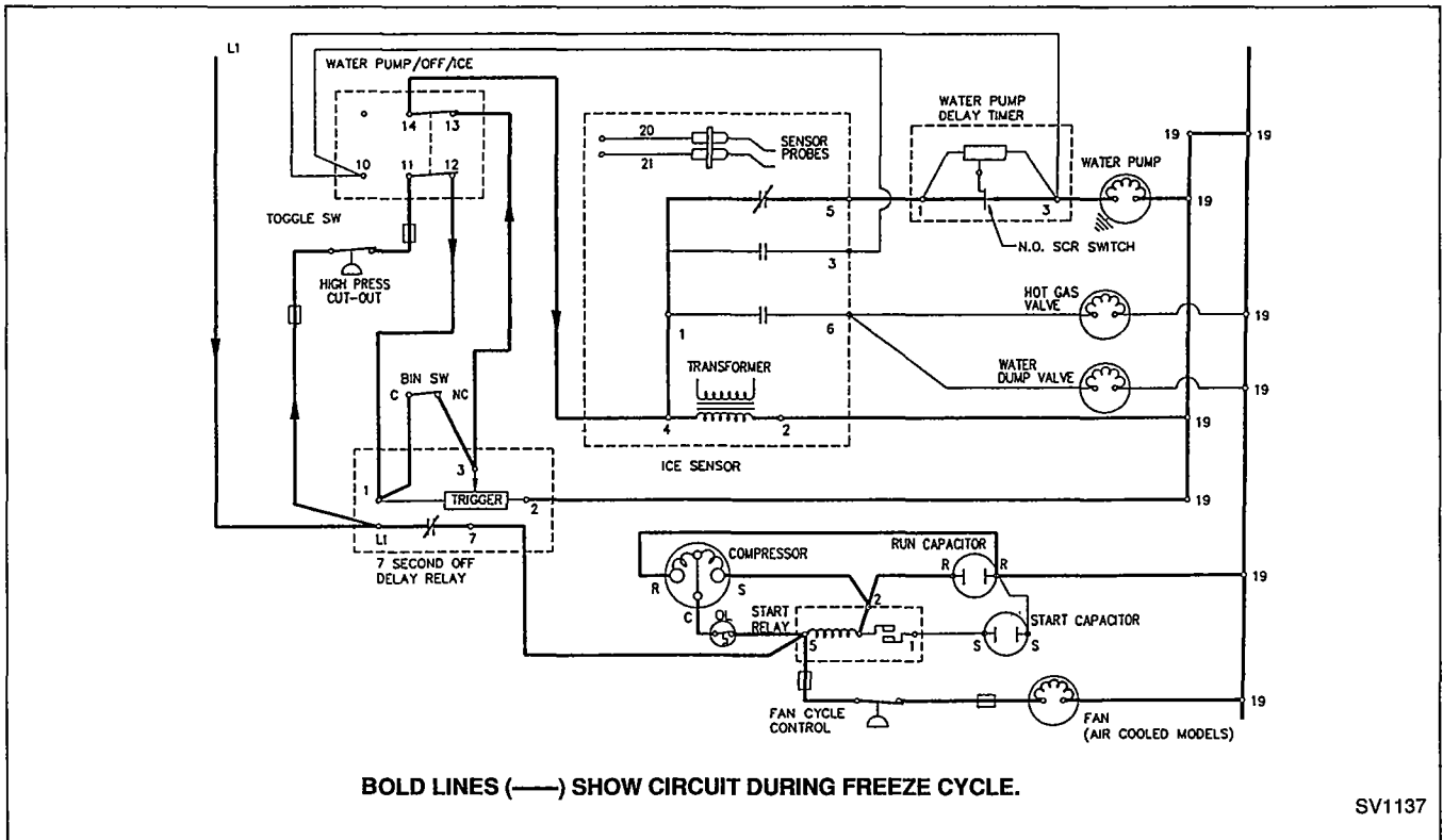
FIGURE 21. FREEZE CYCLE ELECTRICAL SEQUENCE
