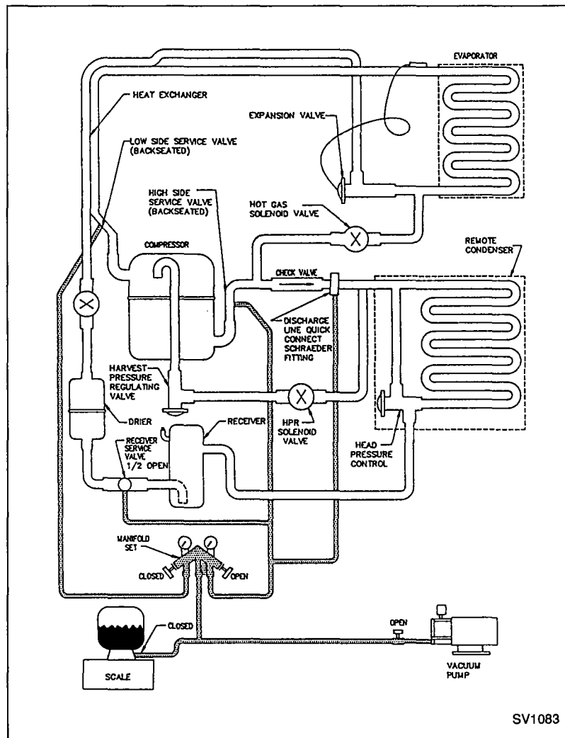
FIGURE 59. EVACUATION OF REMOTE SYSTEMS
