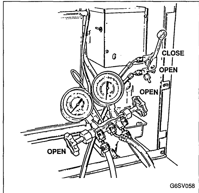
FIGURE 51. REMOVAL OF MANIFOLD GAUGES
