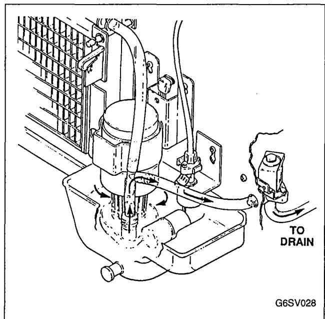
FIGURE 35. HARVEST CYCLE WATER FLOW SEQUENCE
