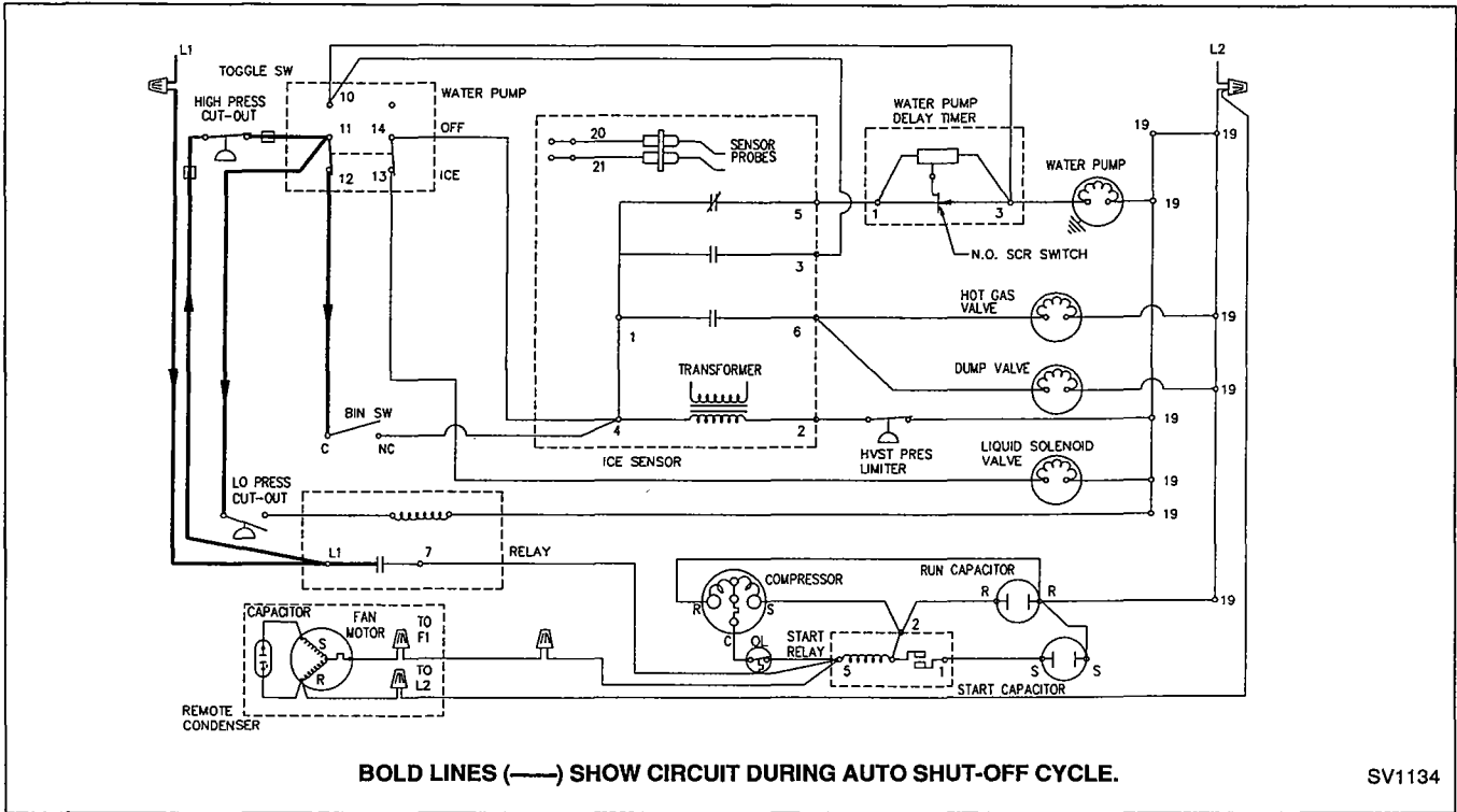
FIGURE 36. AUTOMATIC SHUT-OFF ELECTRICAL SEQUENCE
