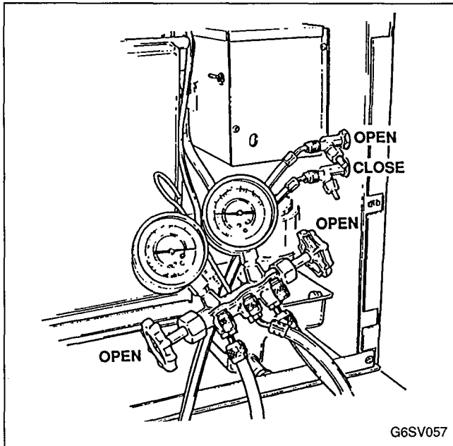
FIGURE 50. INSTALLING MANIFOLD GAUGES
