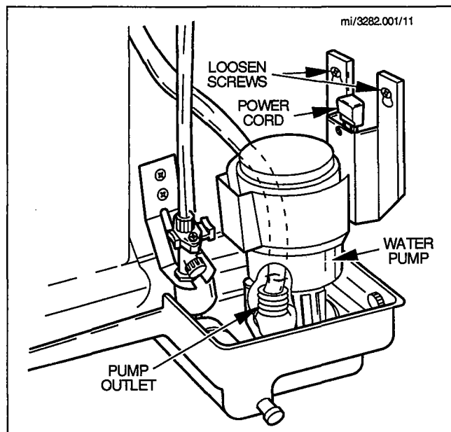
FIGURE 11. WATER PUMP REMOVAL (G200 MODELS SHOWN)
