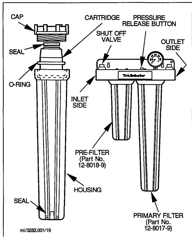
FIGURE 19. WATER FILTRATION
