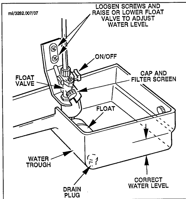
FIGURE 6. WATER LEVEL CHECK (G200 MODELS SHOWN)
