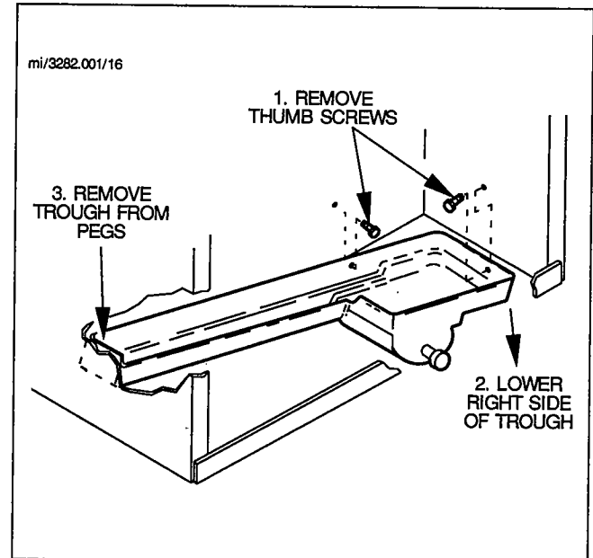
FIGURE 16. WATER TROUGH REMOVAL (G200 MODELS SHOWN)
