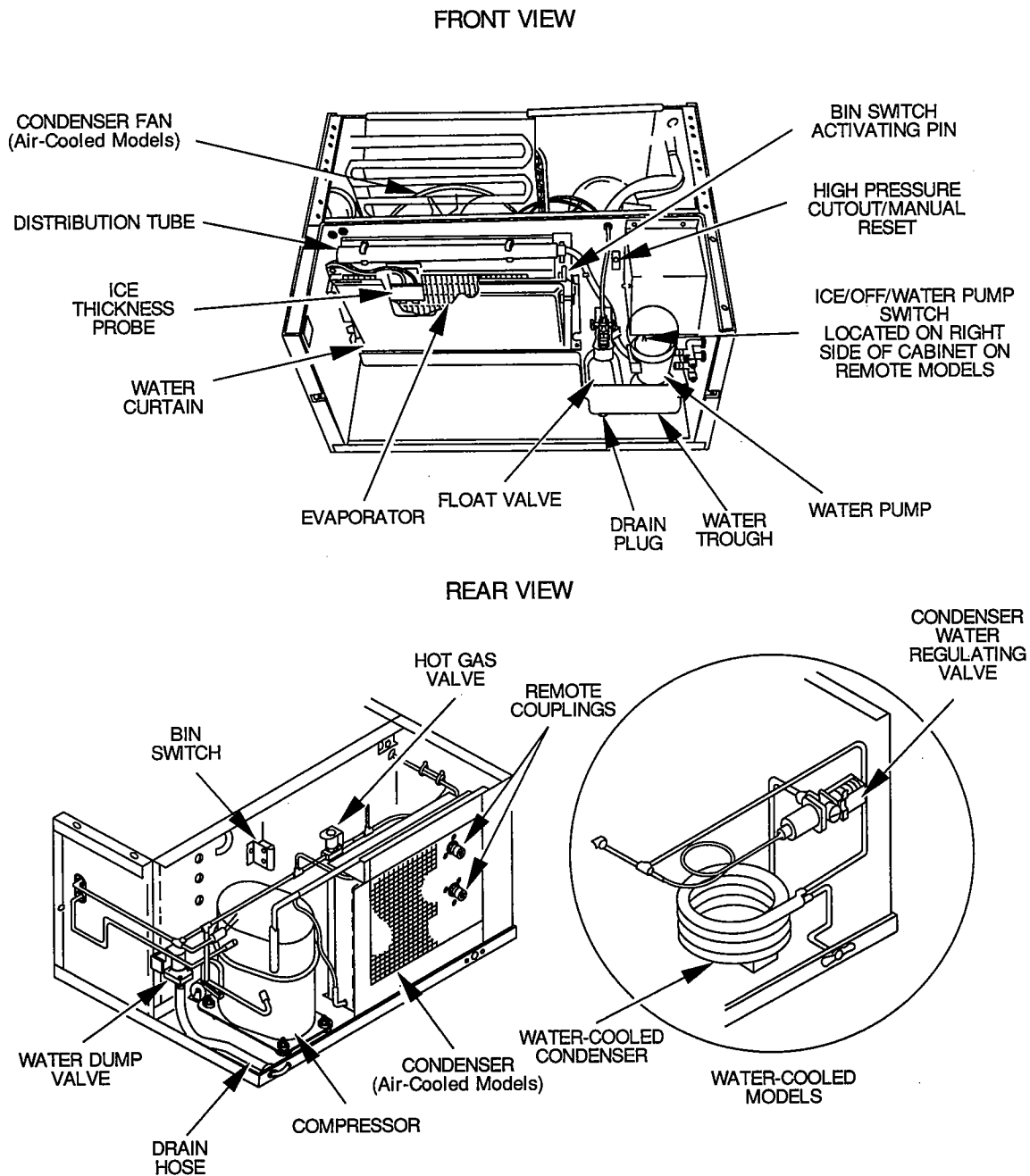
FIGURE 2. COMPONENT LOCATION
