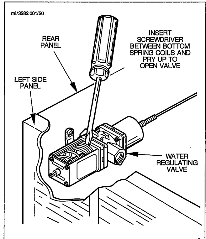
FIGURE 20. MANUALLY OPEN WATER REGULATING VALVE
