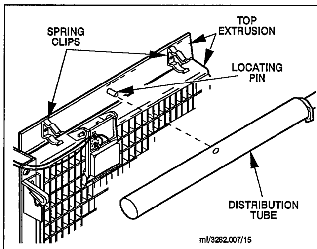
FIGURE 13. DISTRIBUTION TUBE REMOVAL
