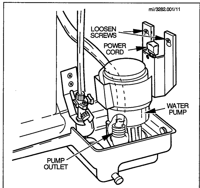
FIGURE 11. WATER PUMP REMOVAL (G200 MODELS SHOWN)
