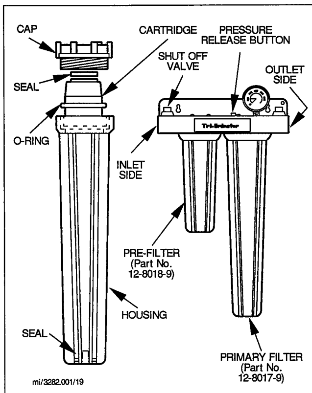
FIGURE 19. WATER FILTRATION
