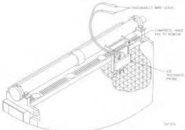
Figure 13. ICE THICKNESS PROBE REMOVAL
