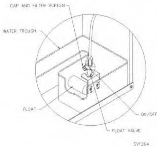
Figure 6. WATER LEVEL CHECK
