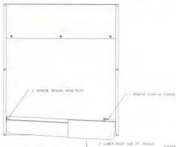
Figure 14. WATER TROUGH REMOVAL
