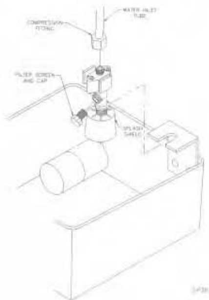
Figure 15. FLOAT VALVE REMOVAL
