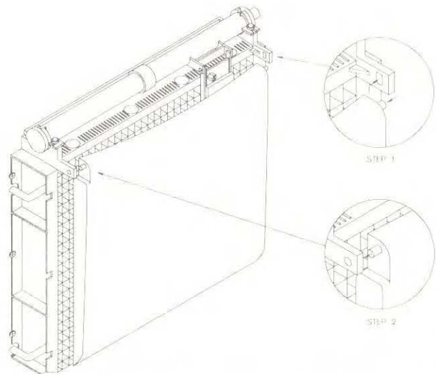
Figure 18. WATER CURTAIN REMOVAL
