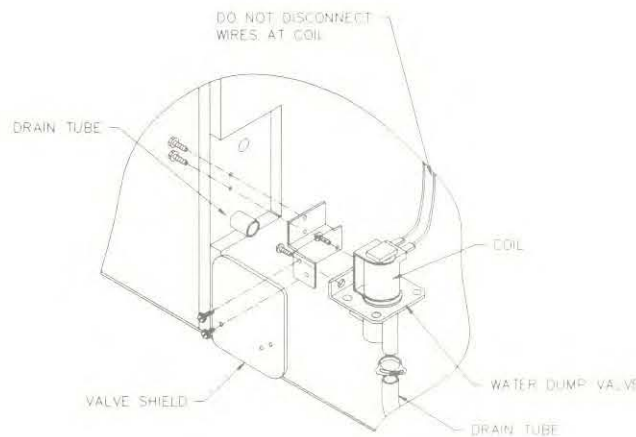
Figure 11. DUMP VALVE REMOVAL
