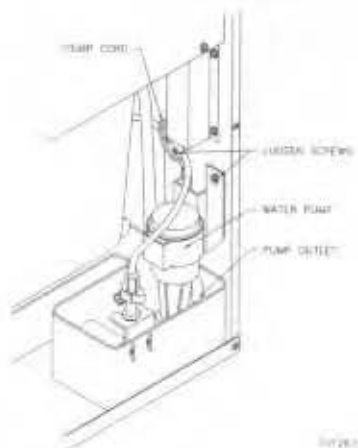
Figure 12. WATER PUMP REMOVAL
