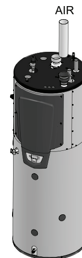
Figure 2-6 Raccordement d'air comburant
