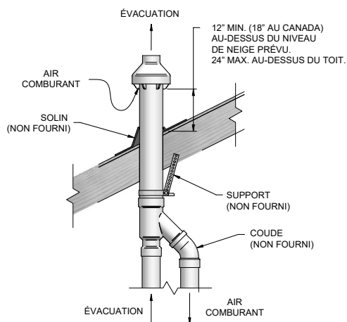
Figure 4-6 Installation de ventilation concentrique verticale
