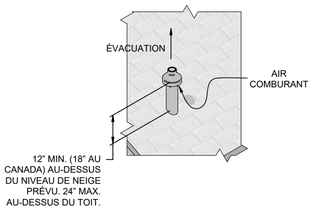
Figure 4-4 Terminaison concentrique verticale
