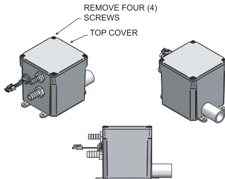
Figure 2-1 Condensate Trap
