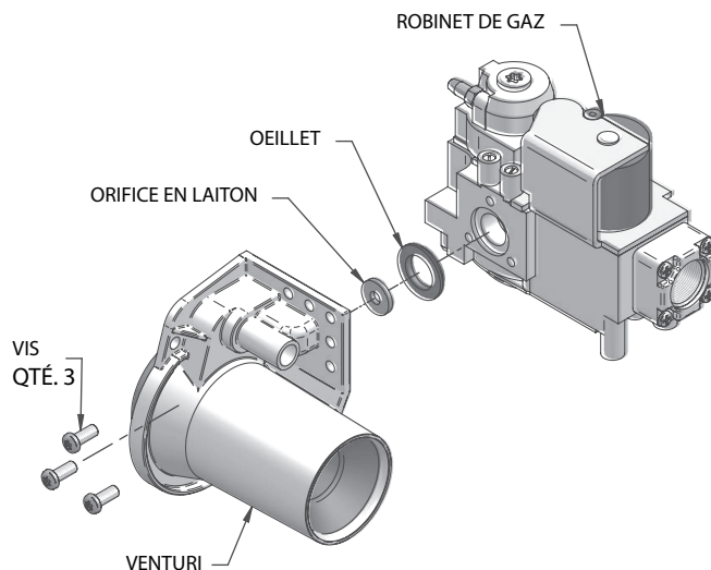
Figure 2-2 Orifice Propane Installation
