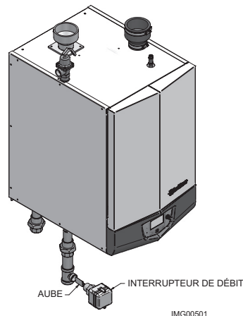
Figure 6-1 Installation du flussostat
