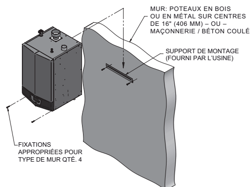
Figure 2-4 Montage de la Chauffe-eau
