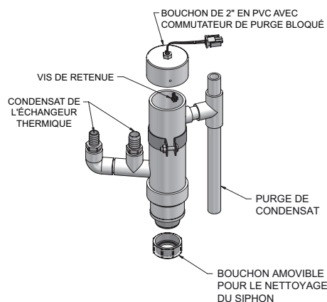
Figure 12-1 Siphon du condensat
