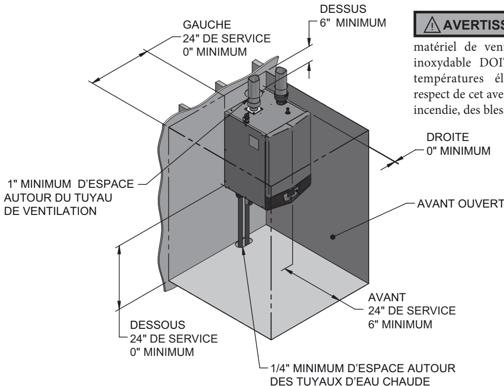
Figure 1-2 Installation en alcôve – Espaces minimum requis
