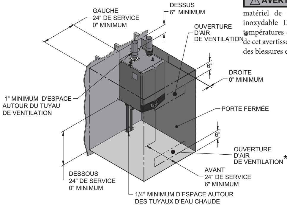
Figure 1-1 Installation en placard – Espaces minimum requis
