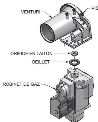
Figure 2-3 Orifice Propane Installation
