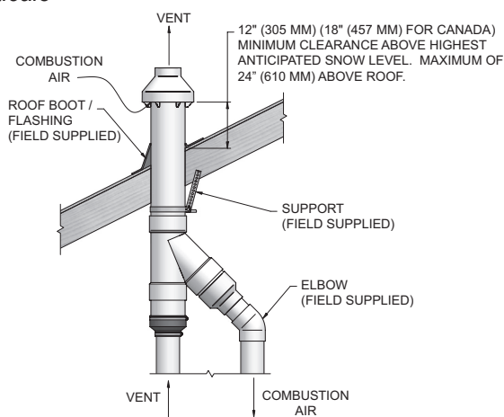
Figure 5-6 Installation de ventilation concentrique verticale
