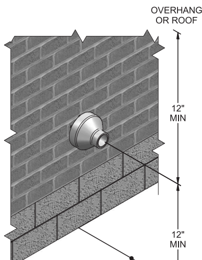
Figure 4-7 Terminaison concentrique murale
