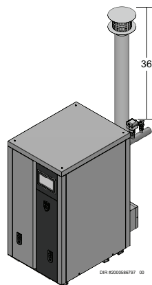
Figure 6-1 Installation extérieure
