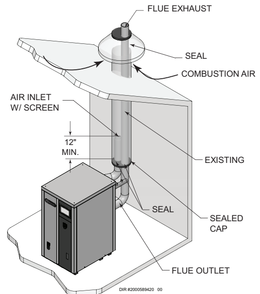
Figure 5-8 Ventilation concentrique, exemple 1
