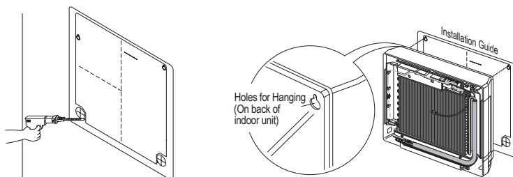
Typical Art Cool Gallery IDU Installation.
