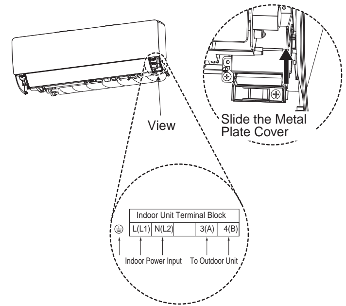
Figure 64: Location of Power Wiring / Communications Cable Terminals in SJ and SK Frame Indoor Units.
