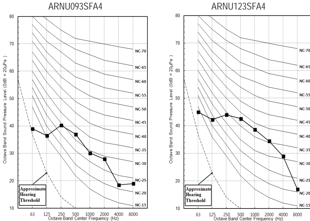
Figure 7: ARNU093SFA4 and ARNU123SFA4 Sound Pressure Level Diagrams.
