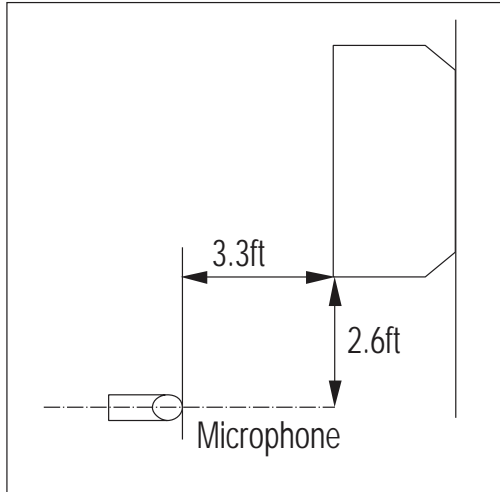
Figure 6: Sound Pressure Measurement Location.
