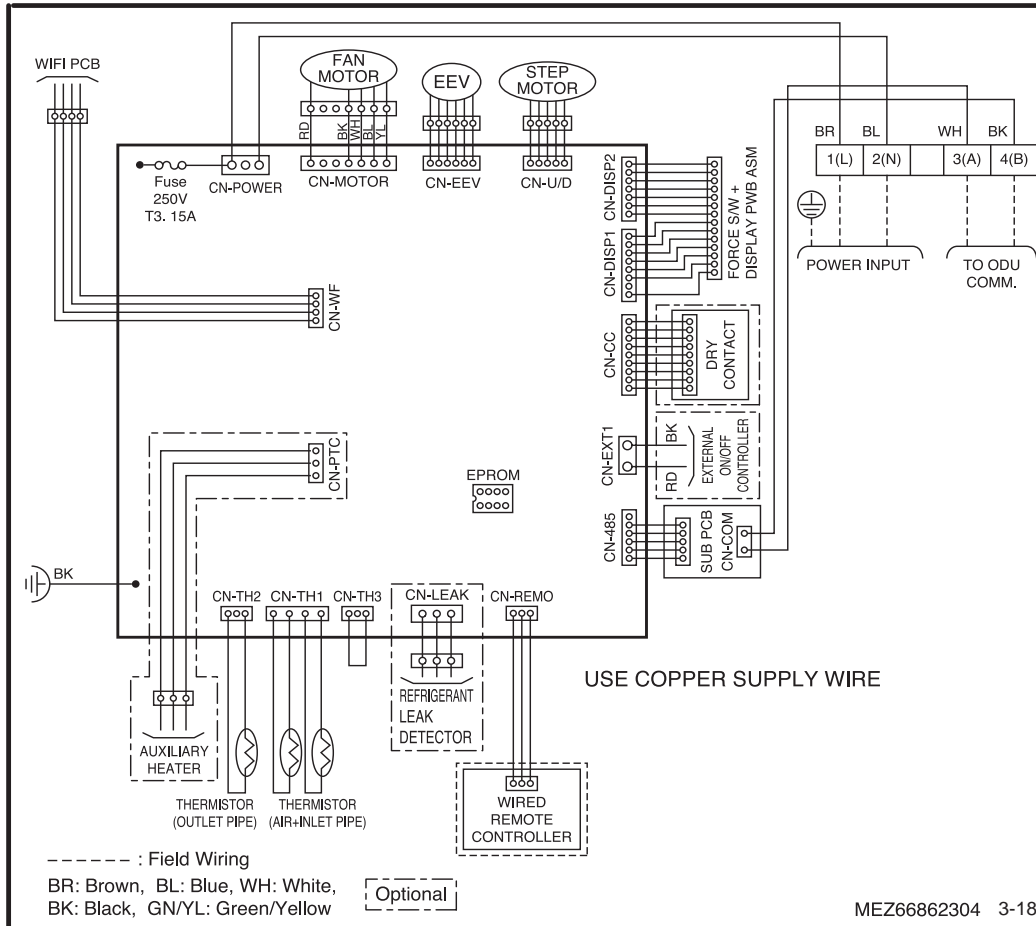
Figure 13: ARNU053~153SJR4 and ARNU183-243SKR4 Wiring Diagram.
