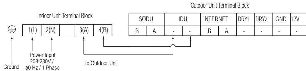
Figure 67: Simplified View of Indoor Unit Terminal Connections—SJ and SK Frames.
