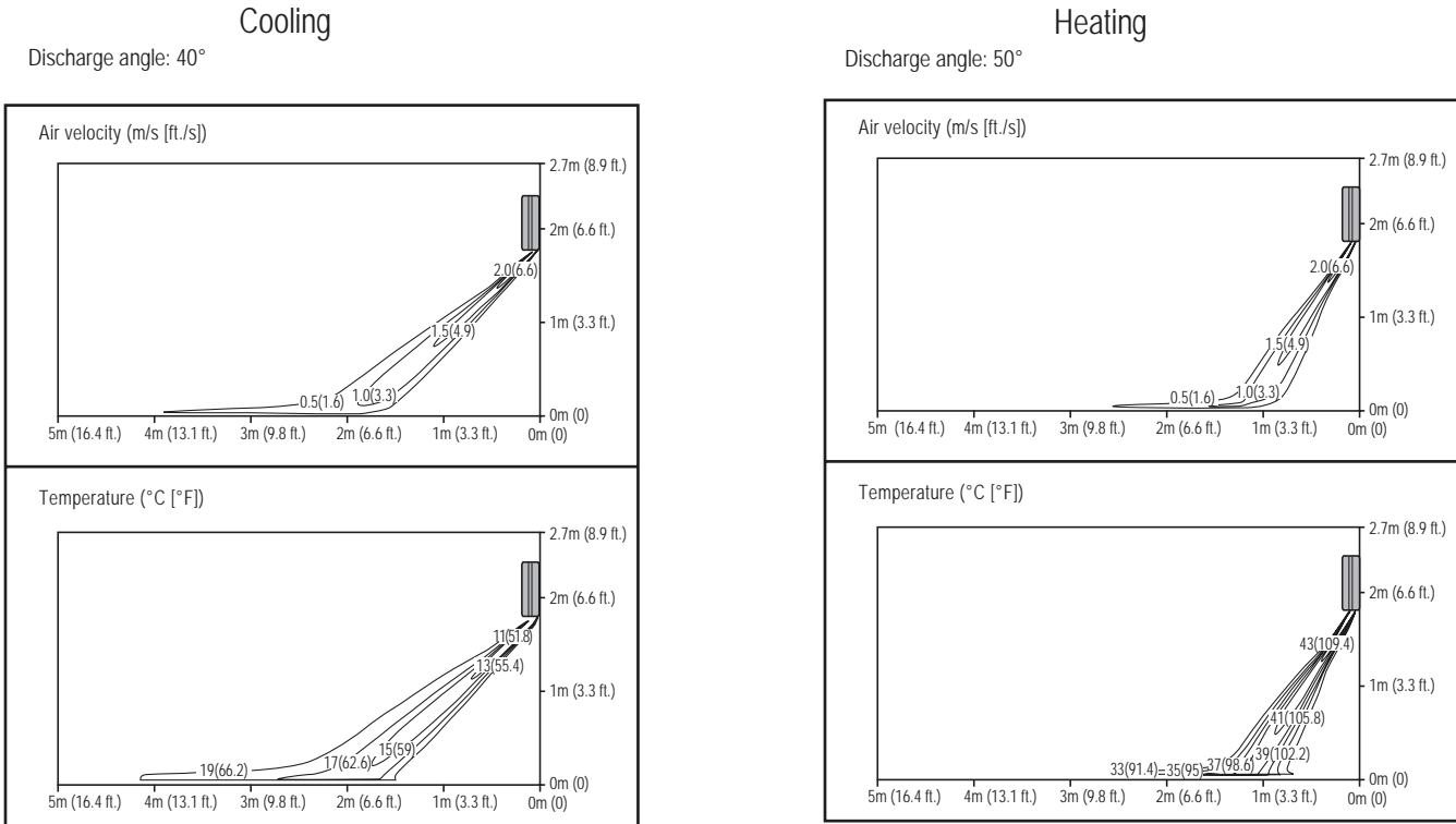
Figure 10: ARNU123SFA4.
