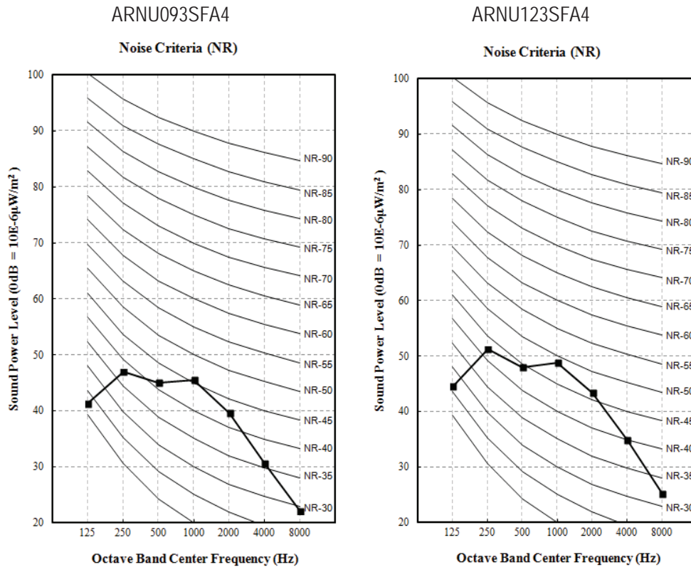
Figure 8: ARNU093SFA4 and ARNU123SFA4 Sound Power Level Diagrams.
