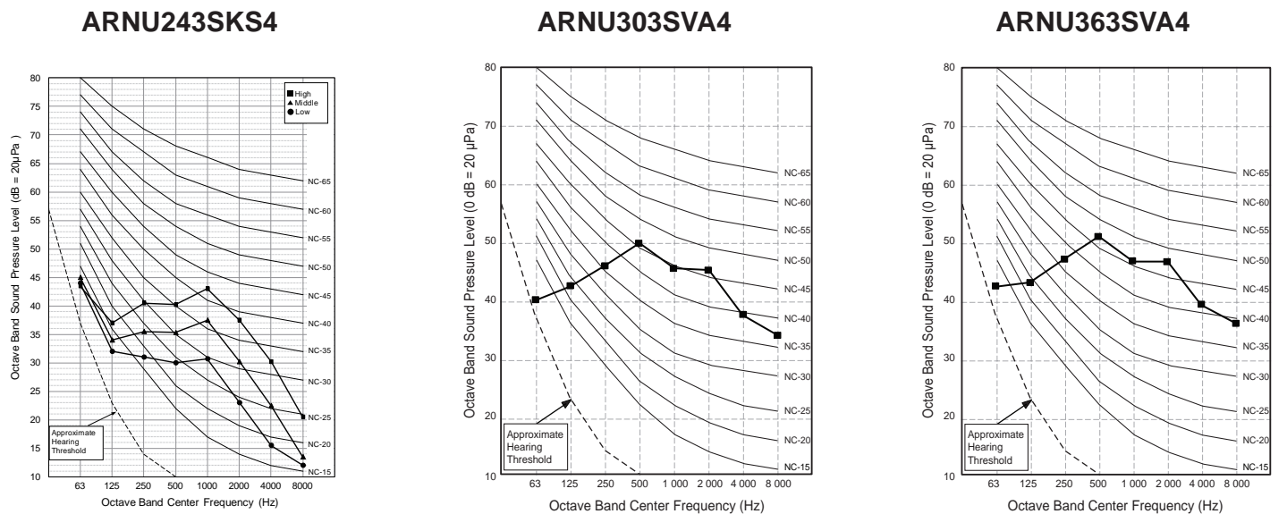
Figure 31: ARNU243SKS4, ARNU303SVA4, and ARNU363SVA4 Sound Pressure Level Diagram.
