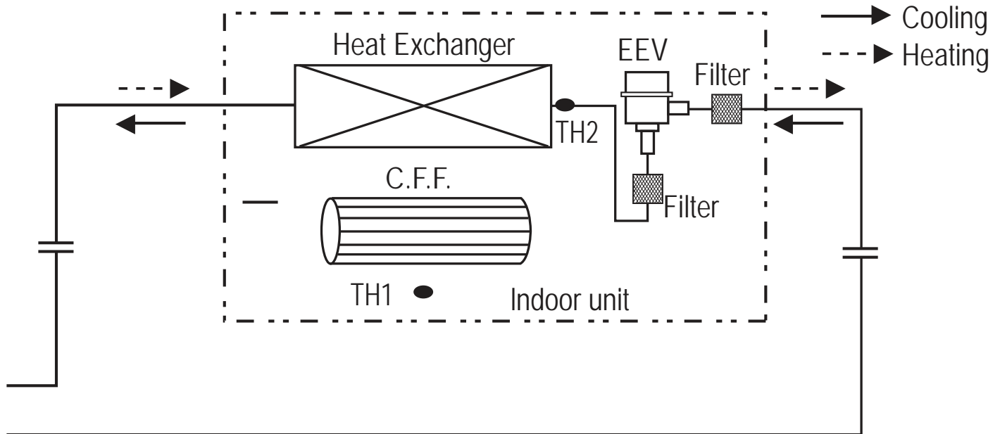
Figure 14: SJ, SK Frame Piping Diagram.
