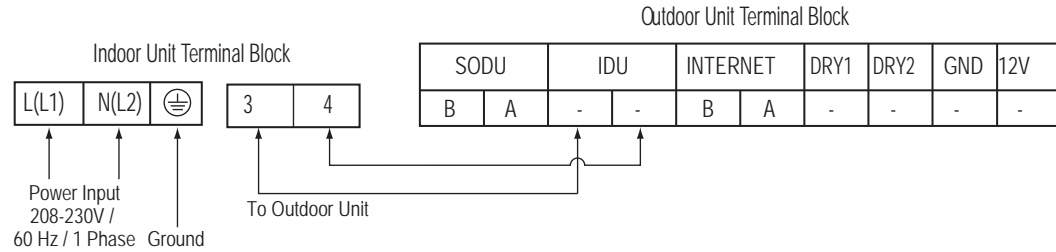
Figure 66: Simplified View of Indoor Unit Terminal Connections—SF Gallery Frames.
