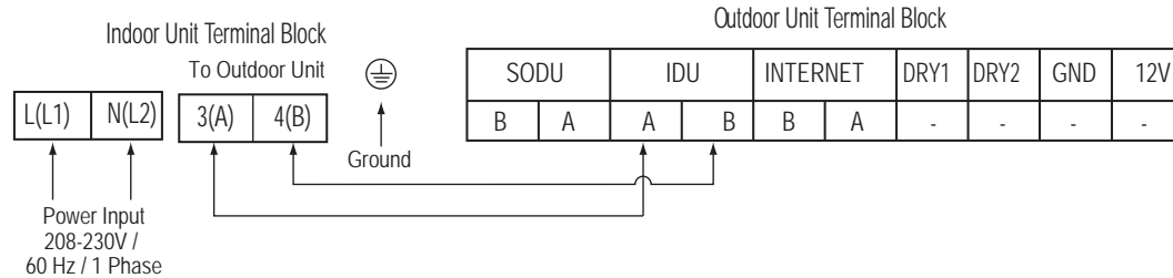
Figure 68: Simplified View of Indoor Unit Terminal Connections—SV Frames.
