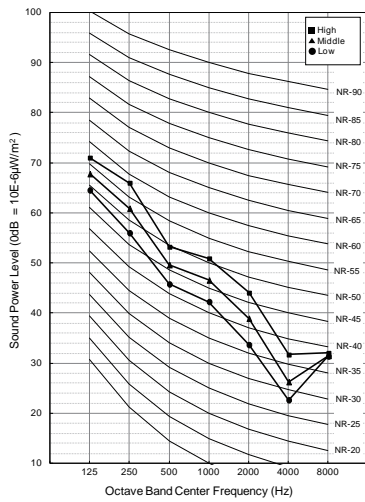
Figure 21: ARNU243SKR4 Sound Power Level Diagrams.
