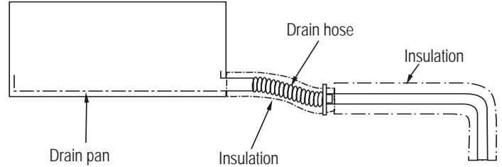
Figure 60: Diagram of an Indoor Unit with a Gravity Drain.
