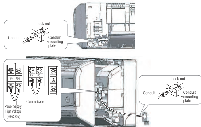
Figure 65: Location of Power Wiring / Communications Cable Terminals in SV Frame Indoor Units.
