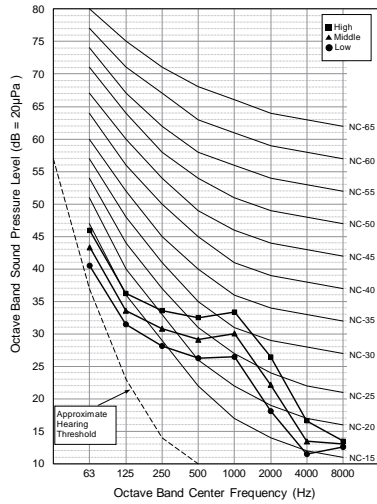
Figure 18: ARNU243SKR4 Sound Pressure Level Diagrams.
