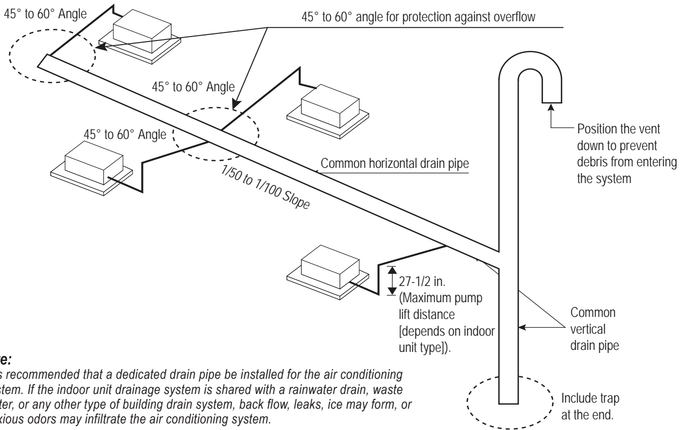
Figure 62: Example of a Common Indoor Unit Drainage System.
