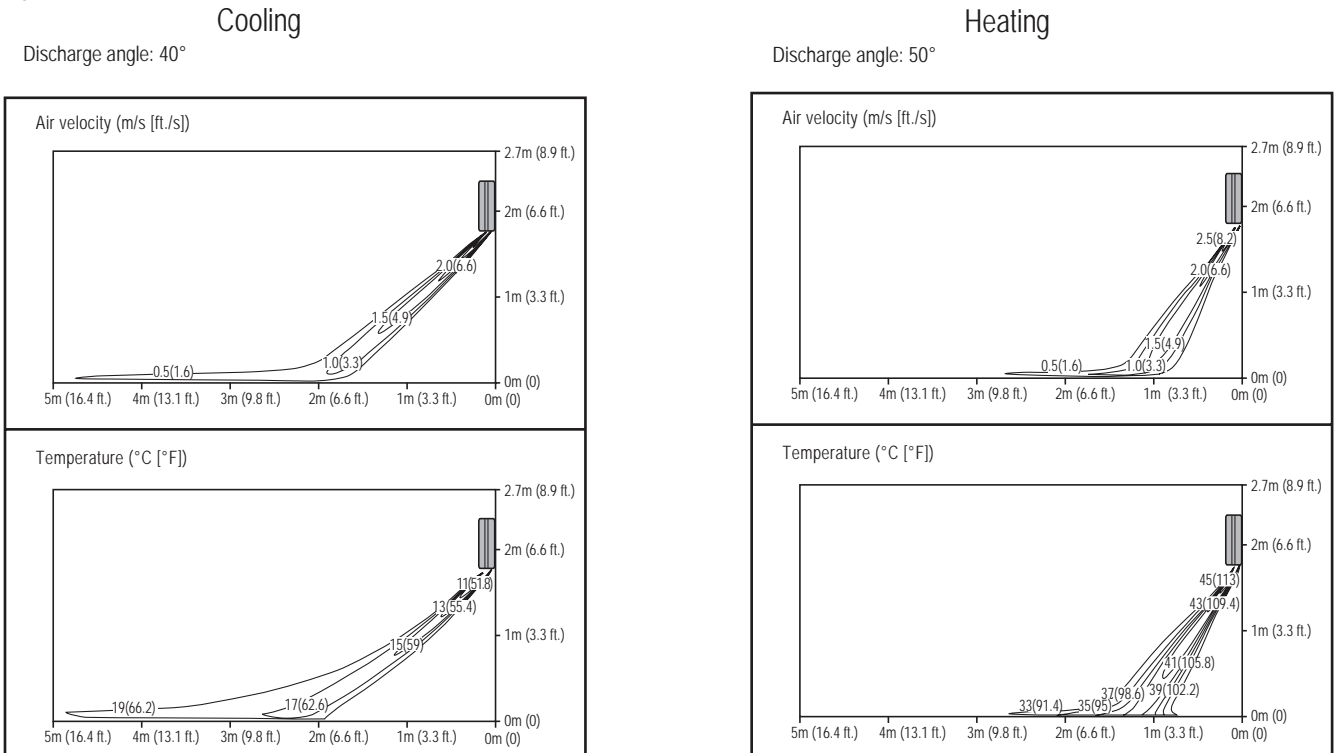
Figure 10: ARNU123SFA4.
