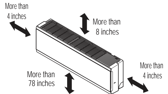
Figure 50: Minimum Clearance Requirements for SJ, SK, SV Frame Wall-Mounted Indoor Units.
