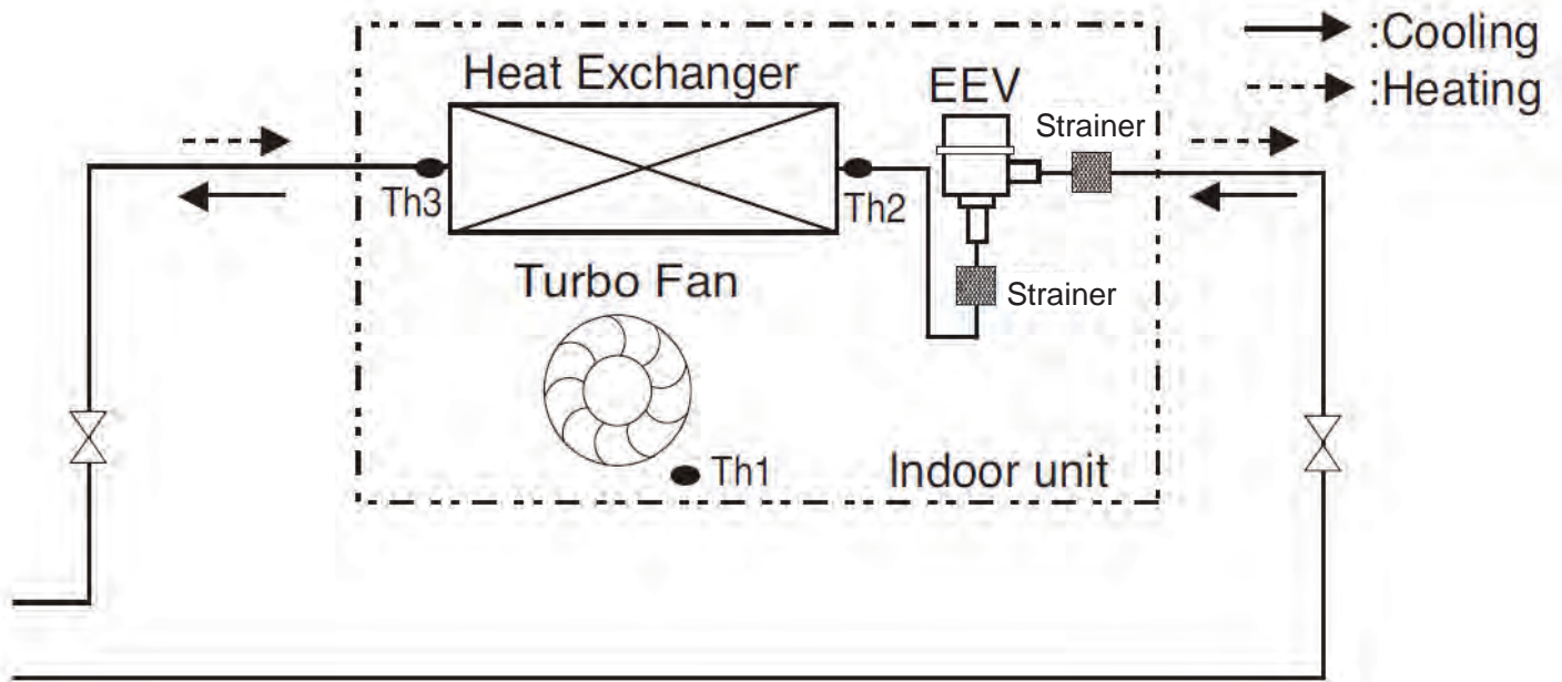
Figure 5: SF Frame Piping Diagram.
