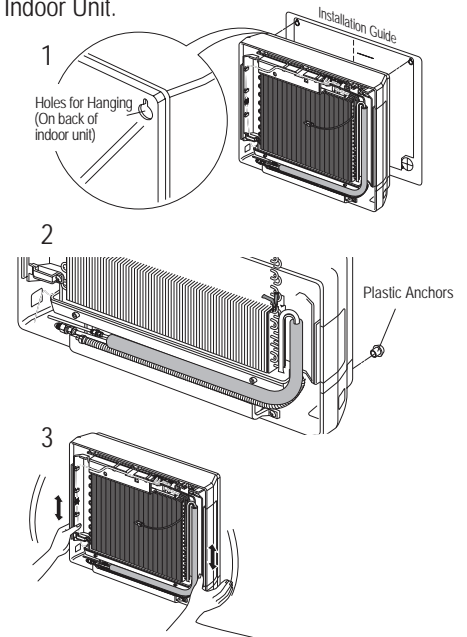
Figure 54: Hanging the SF Frame Gallery Indoor Unit.
