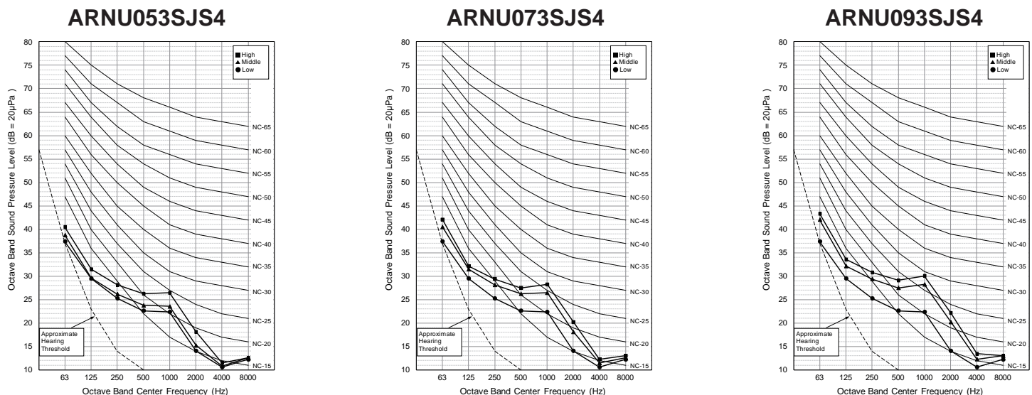
Figure 29: ARNU053SJS4, ARNU073SJS4, and ARNU093SJS4 Sound Pressure Level Diagrams.
