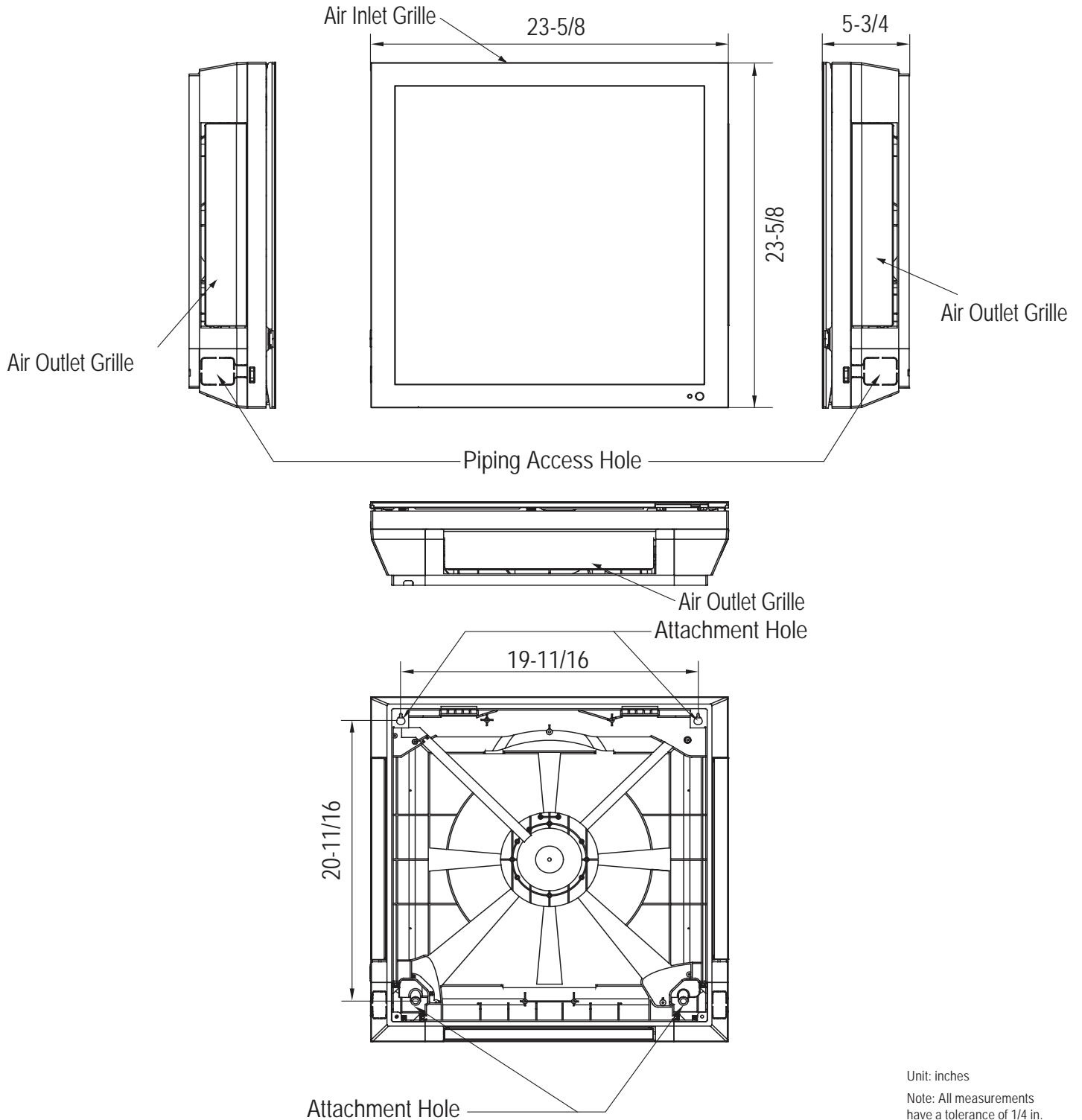
Figure 3: ARNU093SFA4 and ARNU123SFA4 Dimensions.
