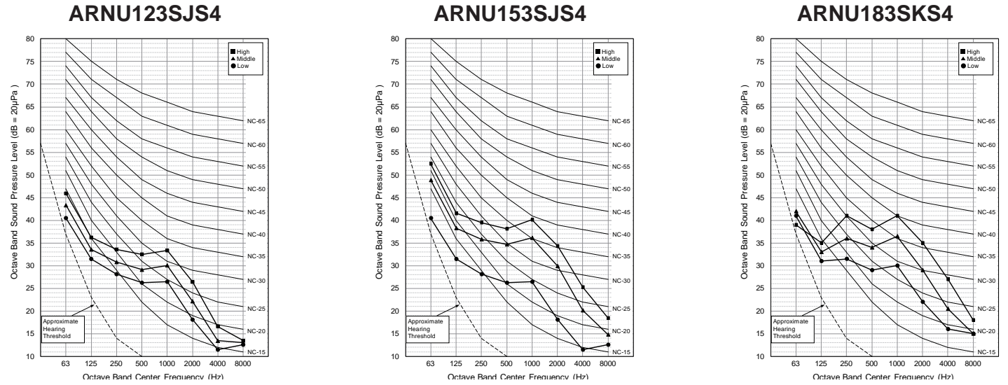
Figure 30: ARNU123SJS4, ARNU153SJS4, and ARNU183SKS4 Sound Pressure Level Diagrams.
