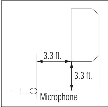
Figure 15: Sound Pressure Measurement Location.
