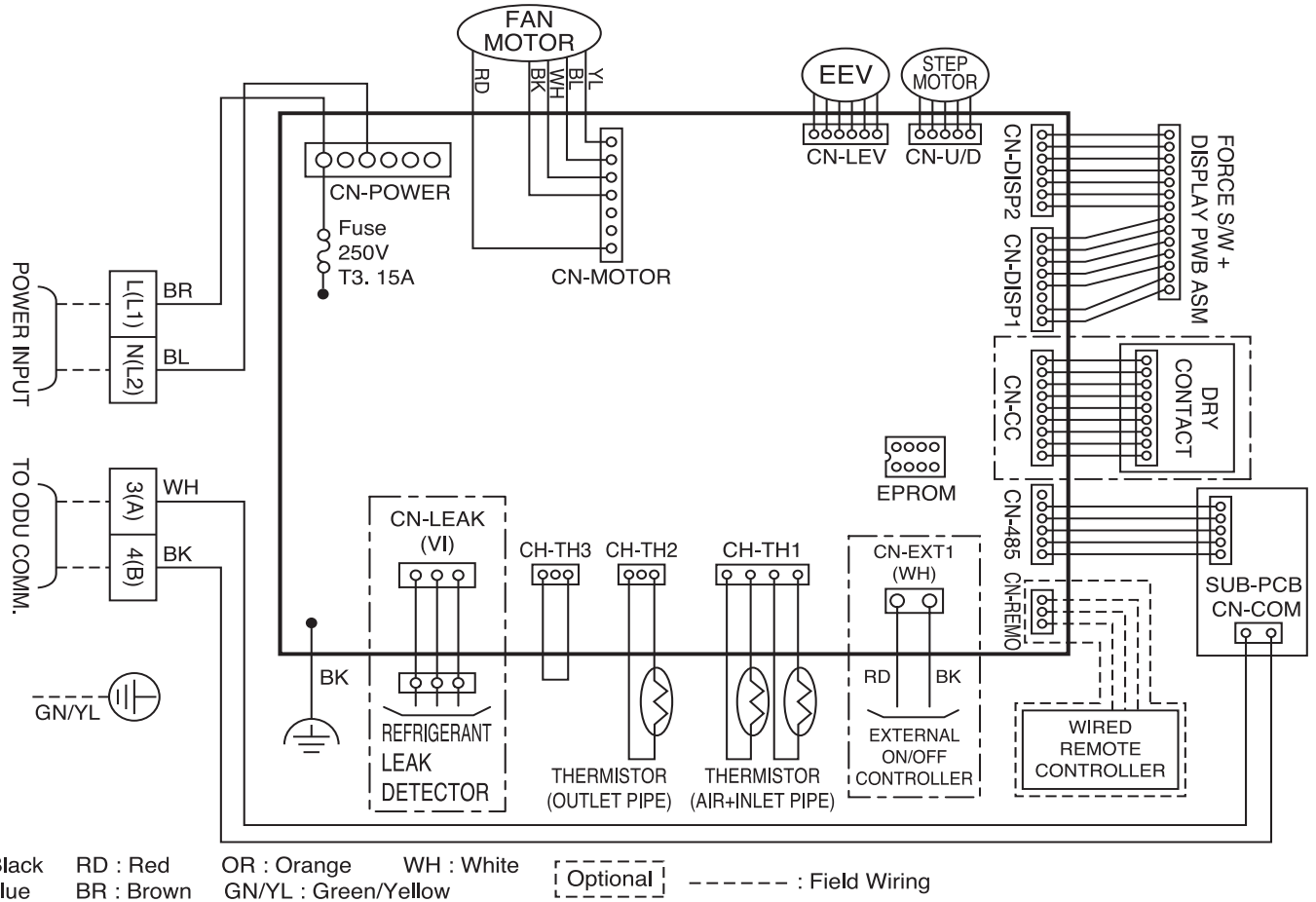
Figure 26: ARNU303SVA4 and ARNU363SVA4 Wiring Diagram.
