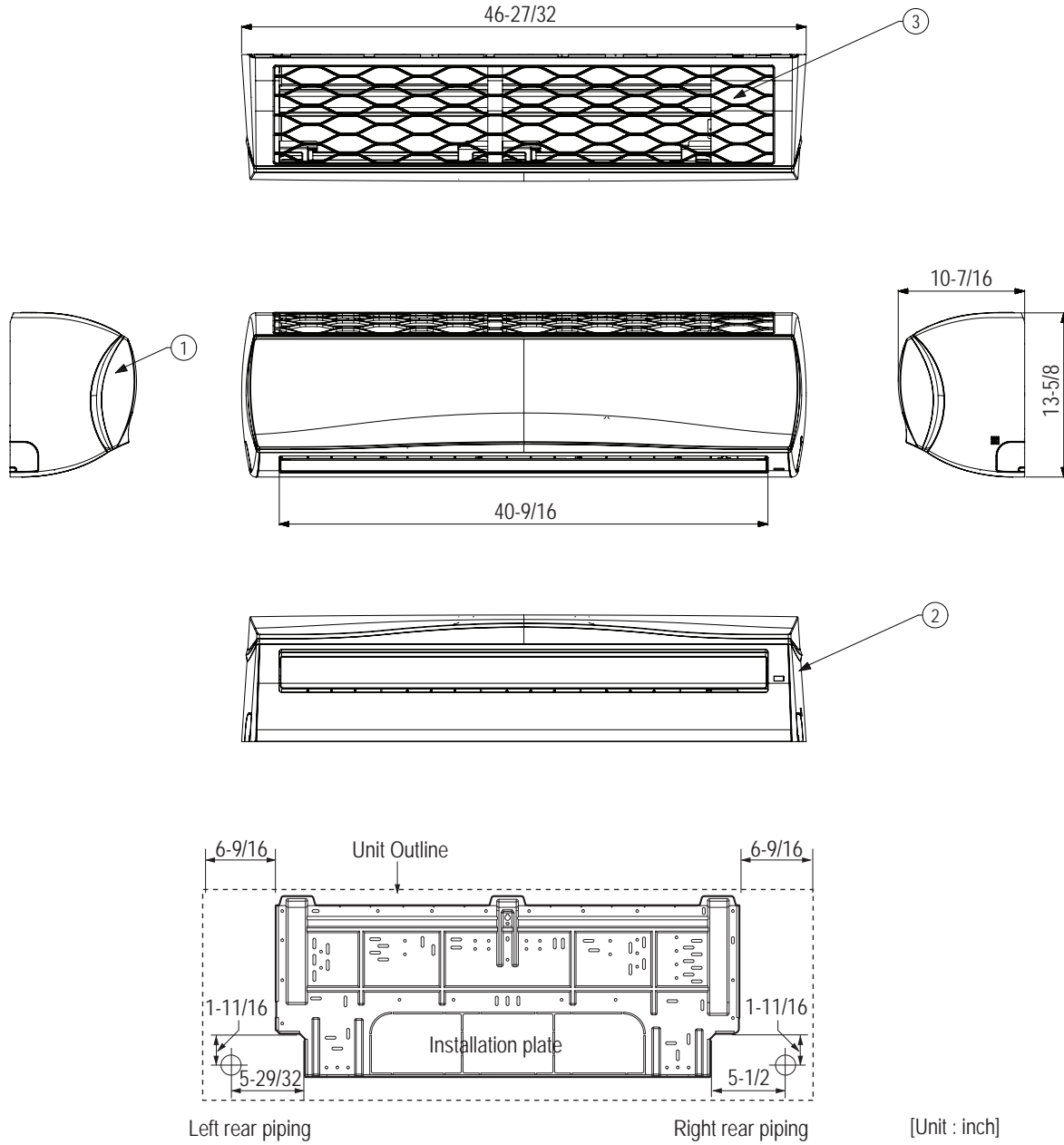
Figure 24: ARNU303SVA4, ARNU363SVA4 Dimensions.
