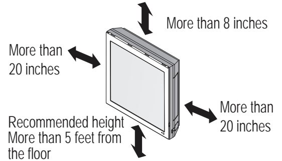
Figure 49: Minimum Clearance Requirements for SF Frame Gallery Indoor Units.
