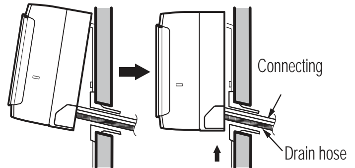
Figure 61: Drain Piping Slope.
