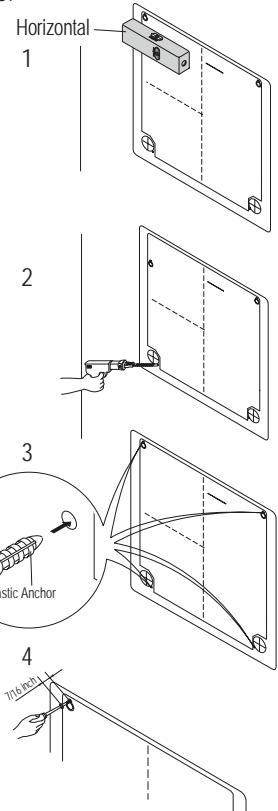
Figure 52: Using the SF Frame Gallery Indoor Unit Installation Guide.
