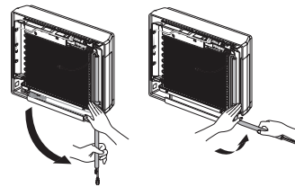
Figure 53: SF Frame Gallery Indoor Unit Right Side Piping Access.
