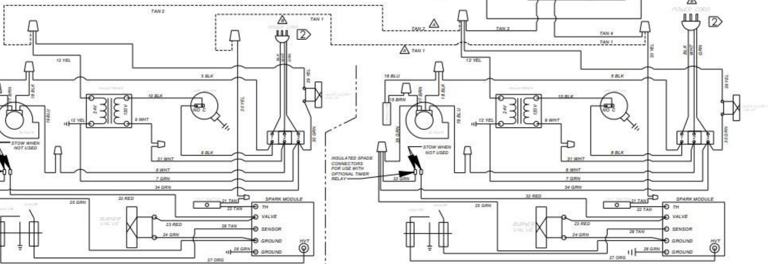
CLAMSHELL HOOD & CARRIAGE BOX 2 (OPTIONAL)
