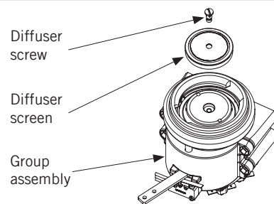
Figure 5 - Integrated Brew Group
