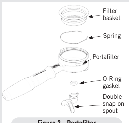
Figure 3 - Portafilter
