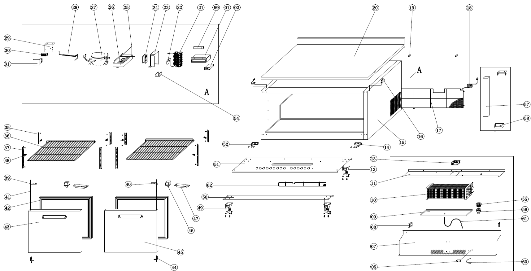
EXPLODE OF KCHUCWT60R
